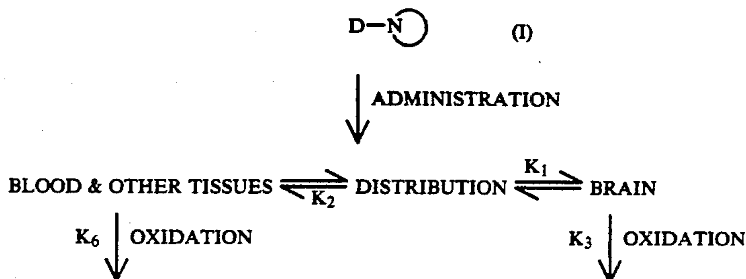
SCHEME 2
