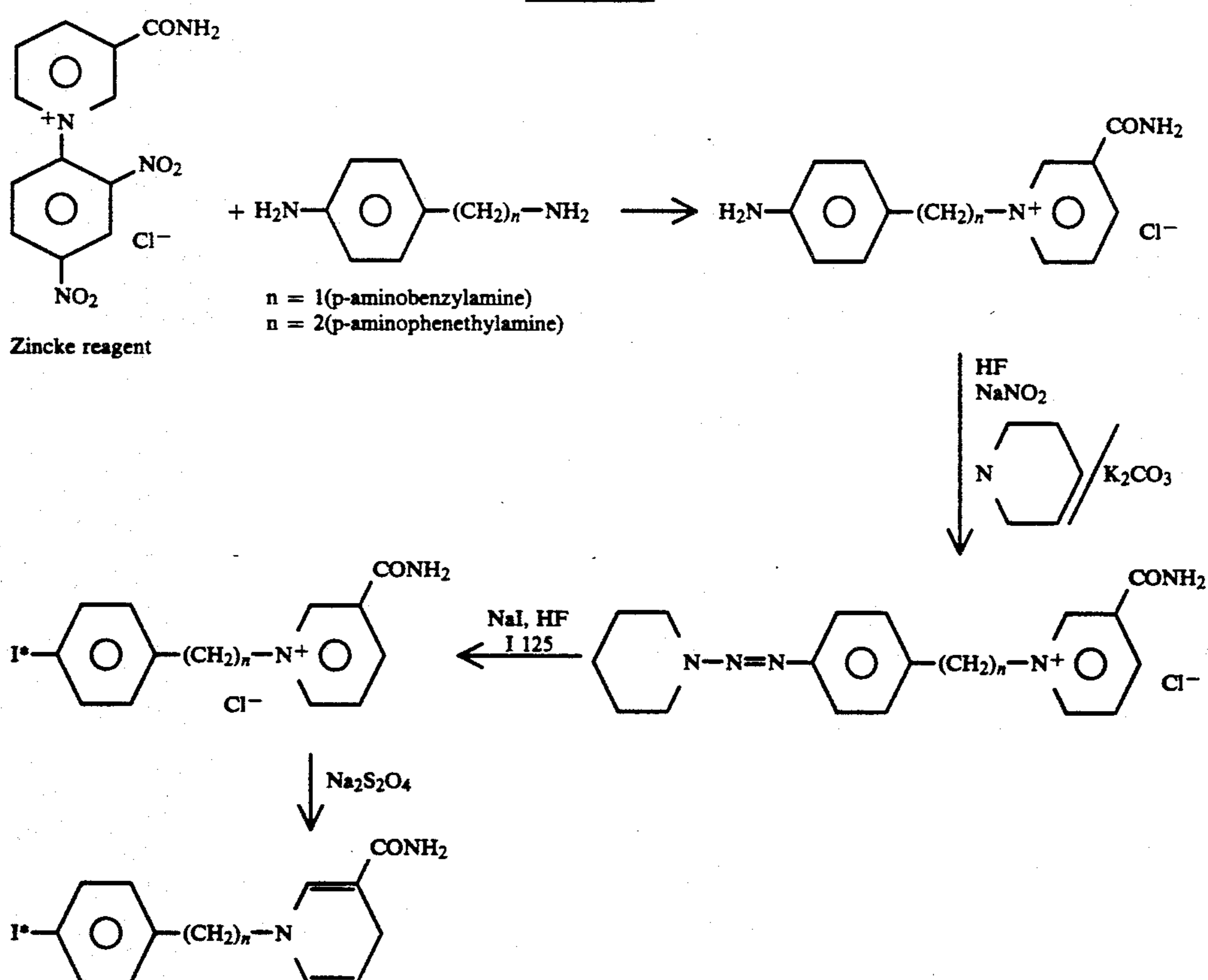
SCHEME 6
