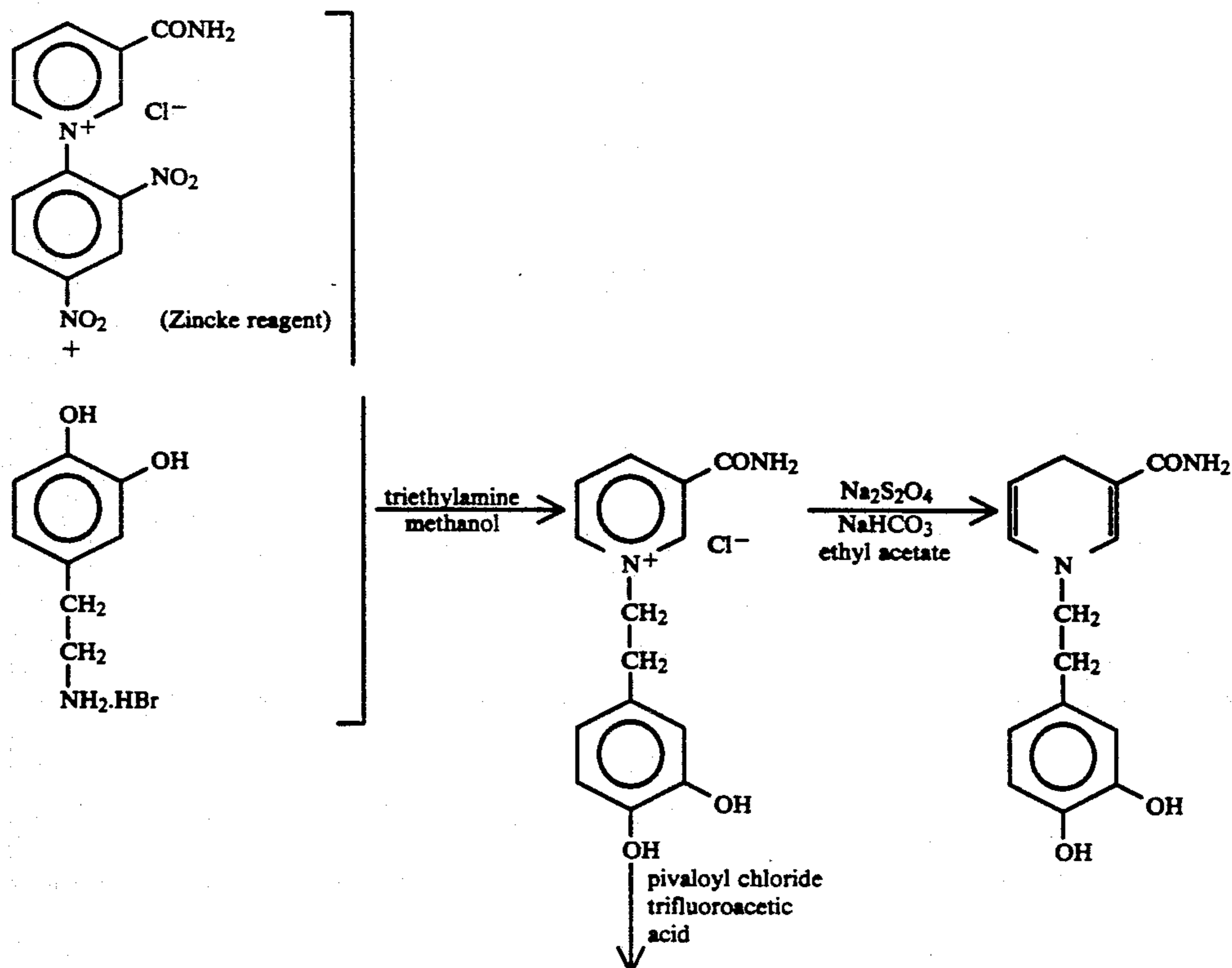
SCHEME 3
