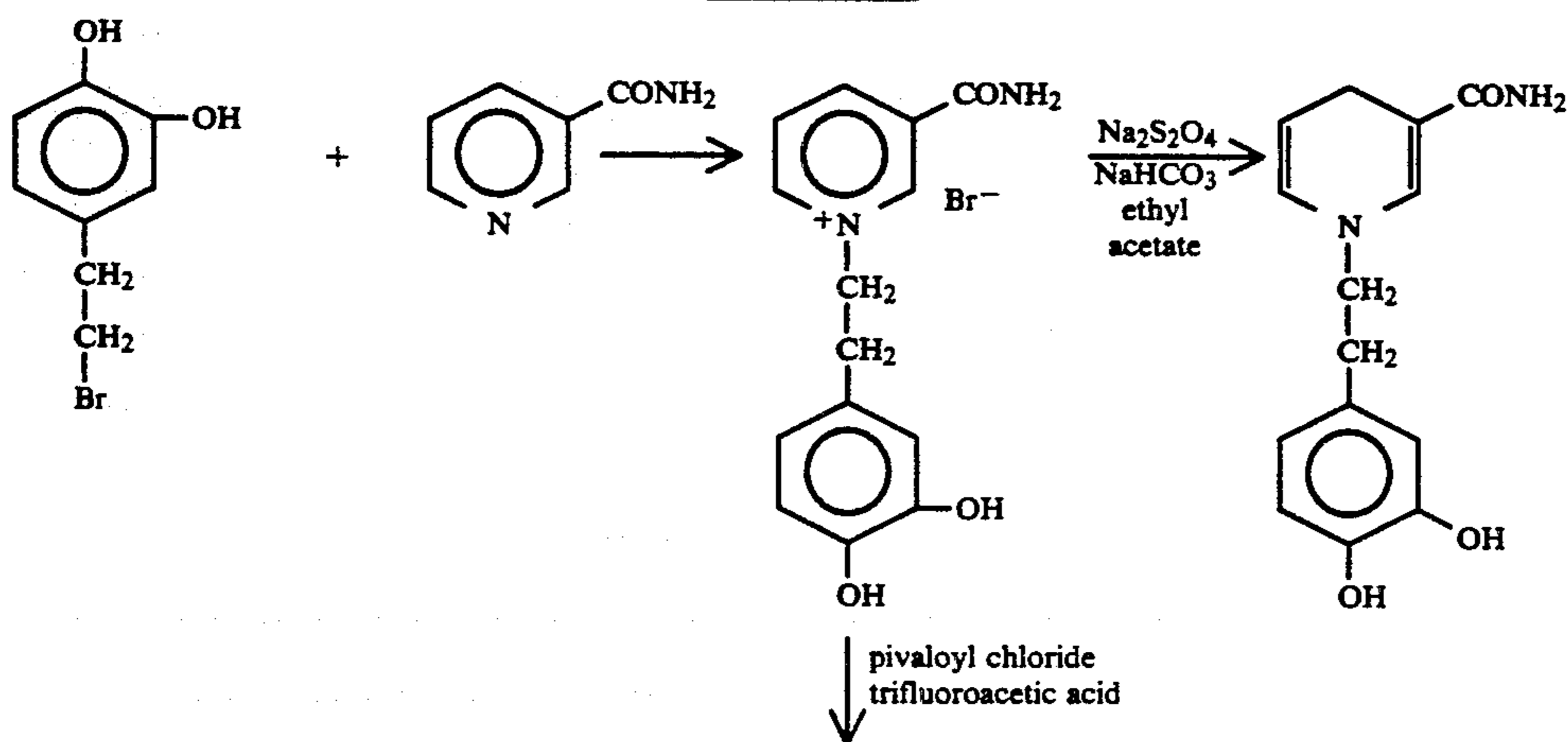
SCHEME 4
