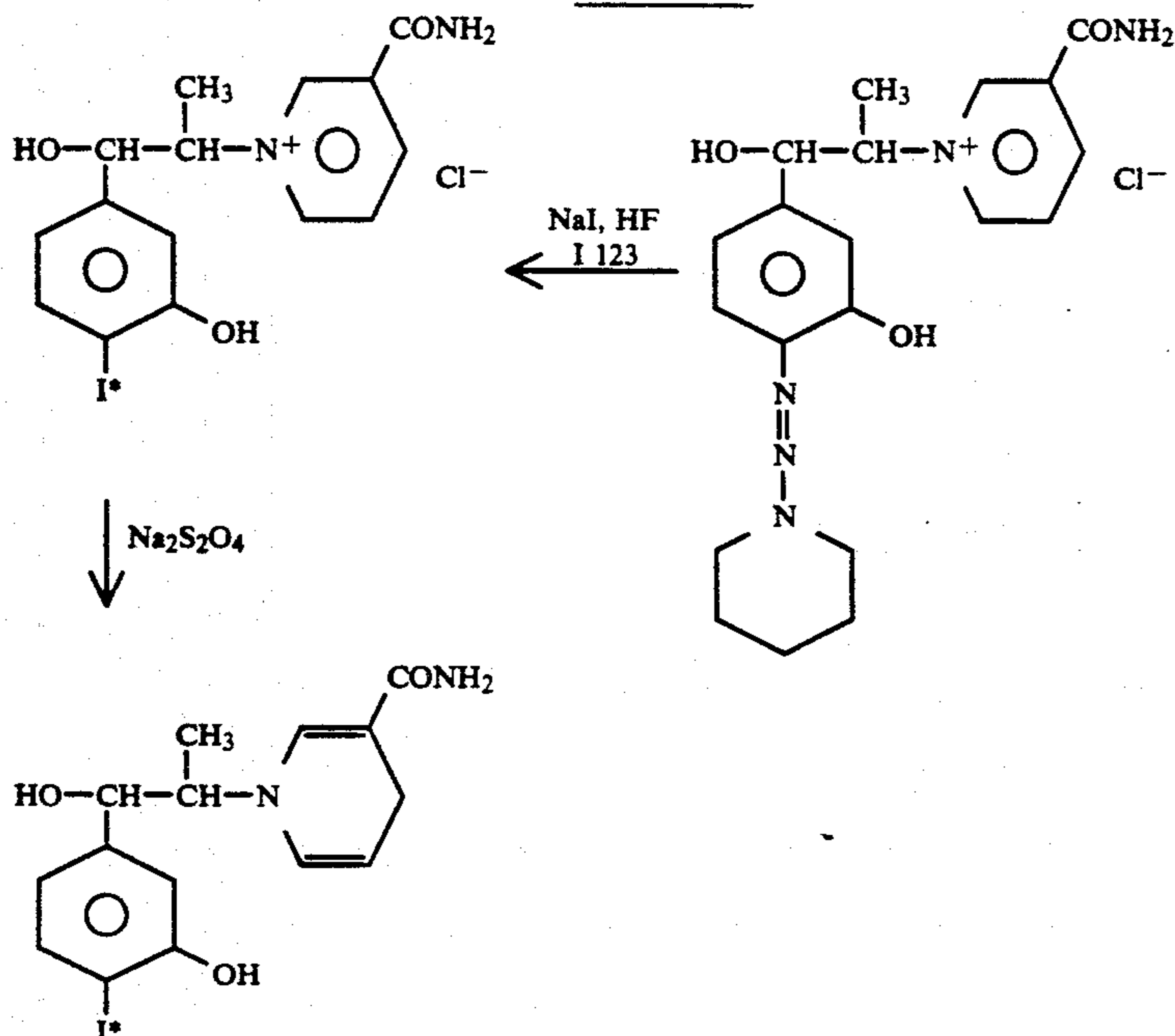
SCHEME 5
