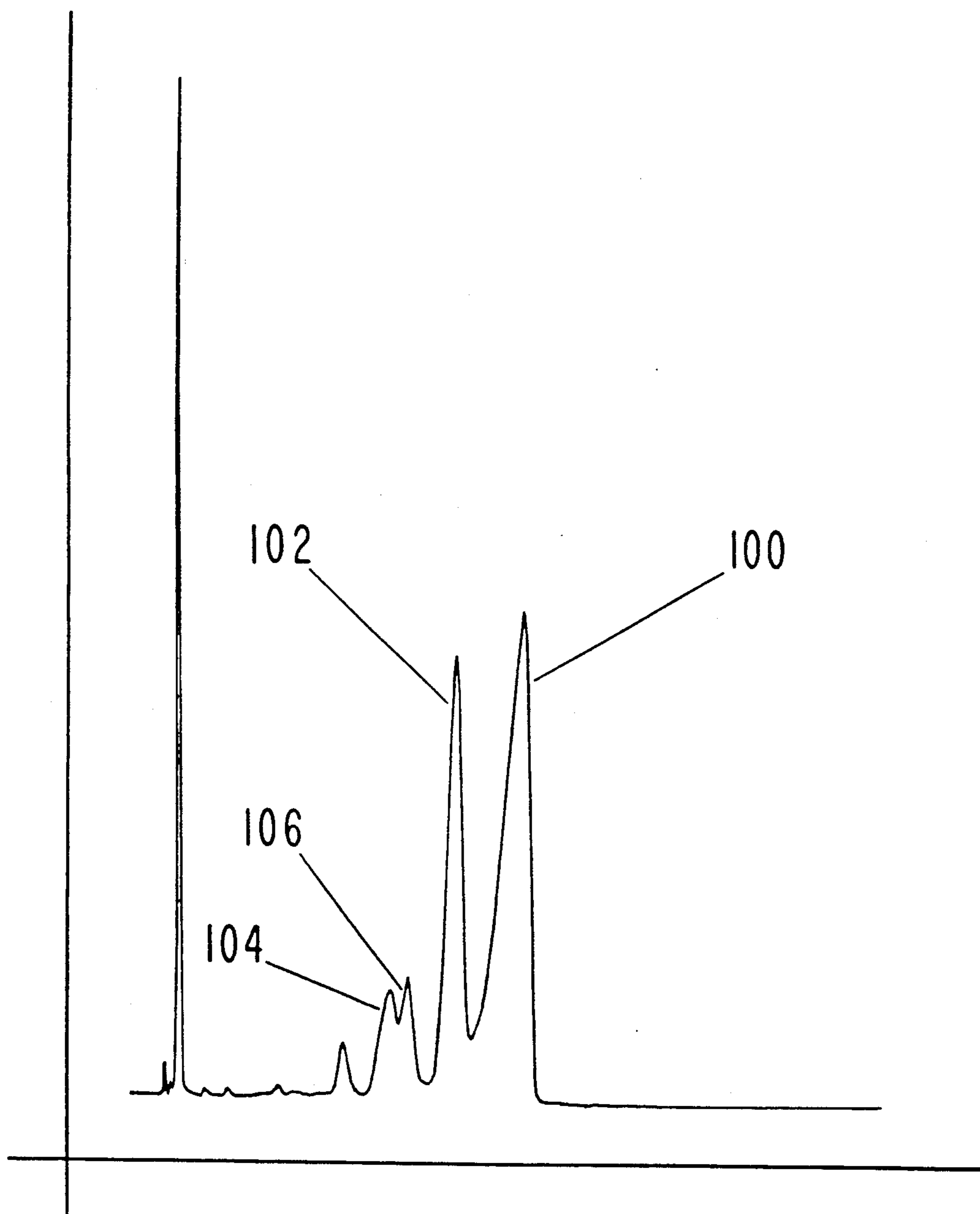
GLC PROFILE FOR EXAMPLE V.
