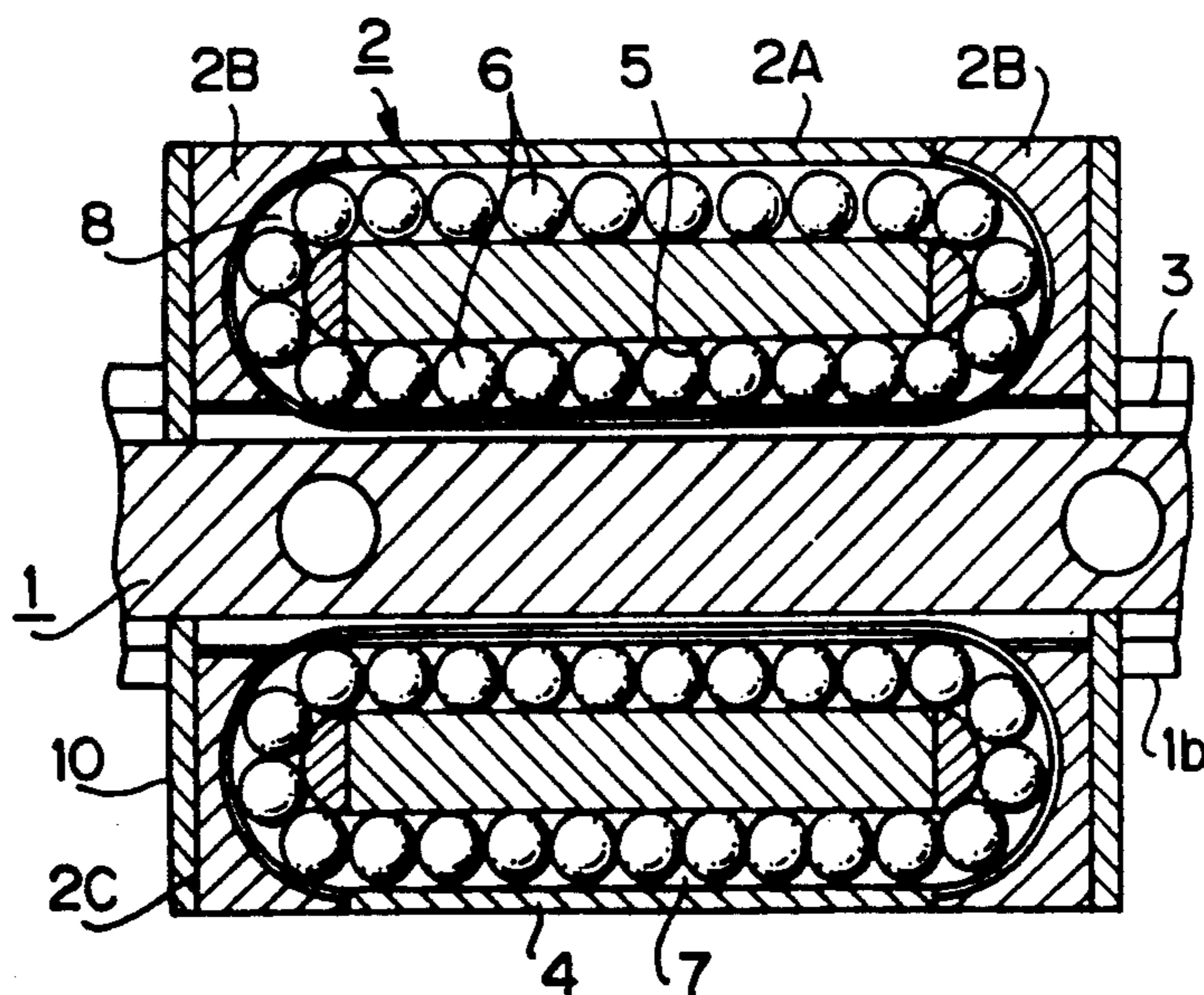
FIG. 4 (PRIOR ART)
