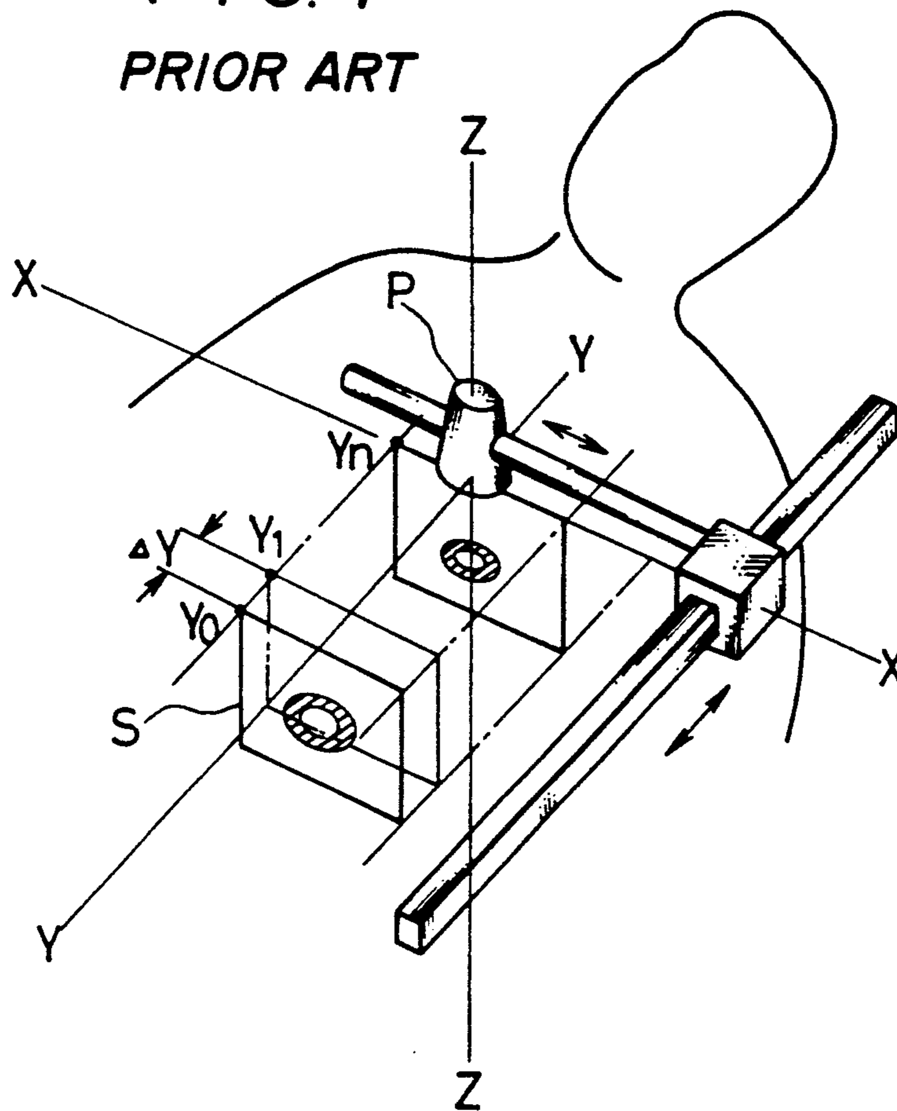
FIG. 8 PRIOR ART
