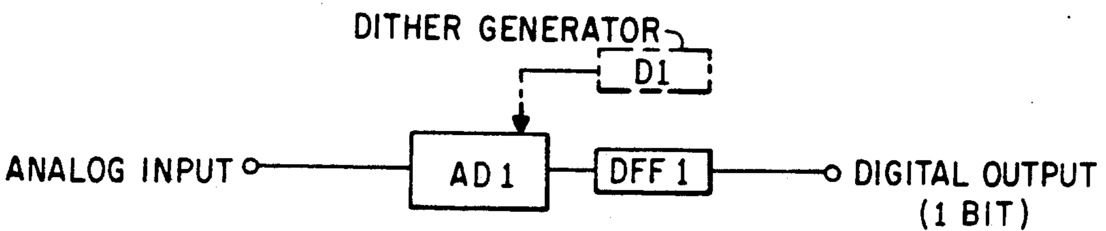
PRIOR ART FIG. 9
