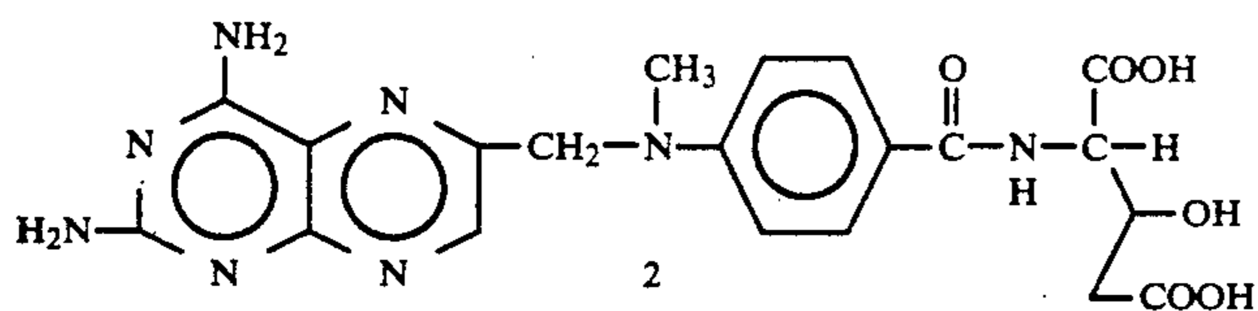
Scheme-2 Steps of the reaction synthesis of 4-amino-4-deoxy-10-methylpteroyl- \gamma -hydroxyglutamic acid (2).
