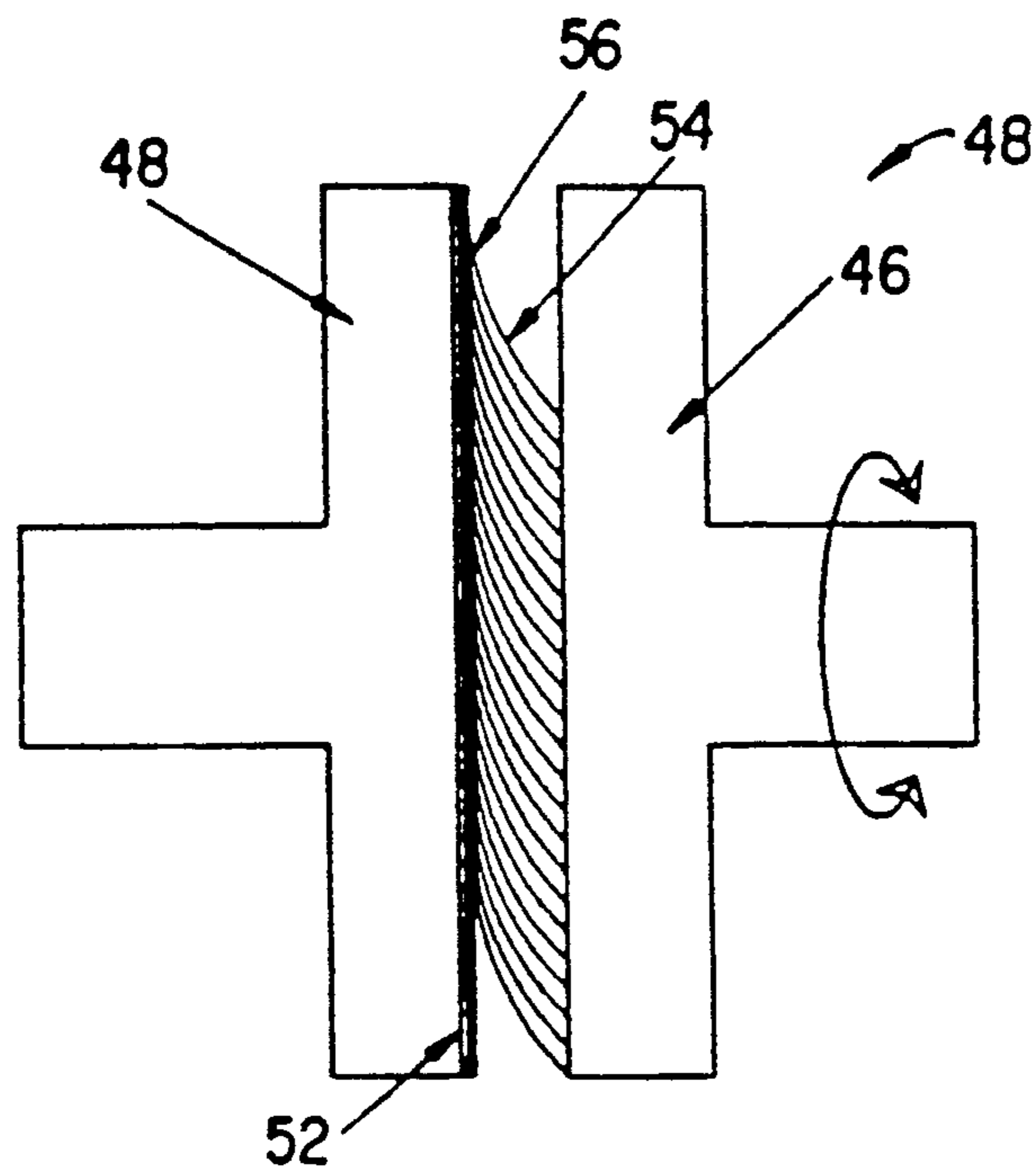
FIG. 4 (PRIOR ART)
