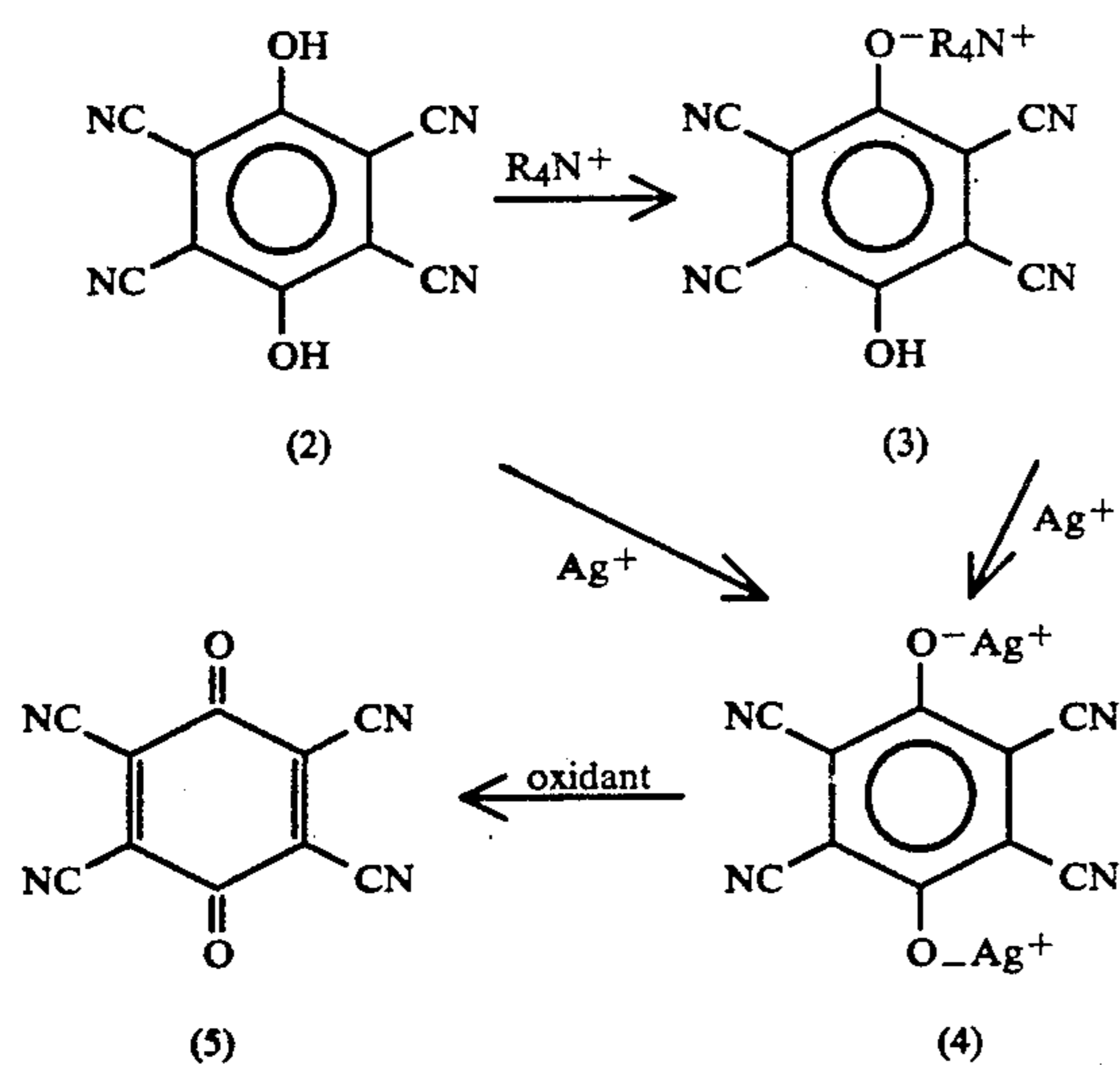
-continued Scheme 1
