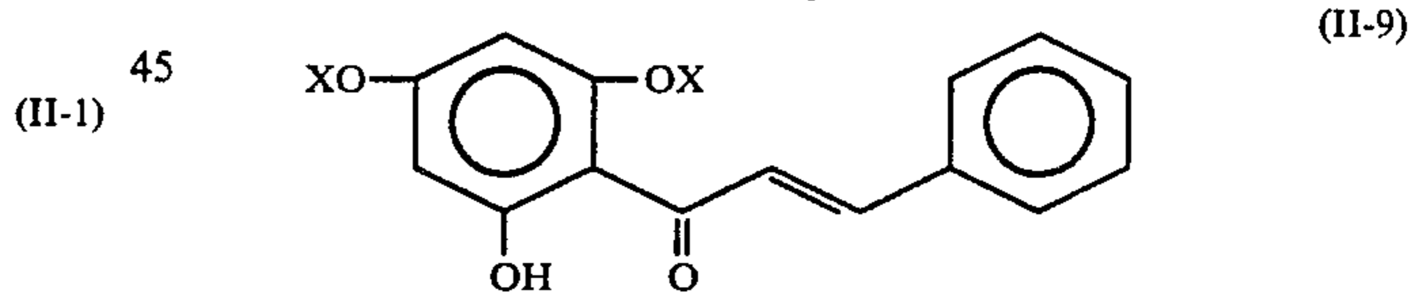
2'-Hydroxy-4,4',6'-tris(tetrahydropyranyloxy)chalcone
