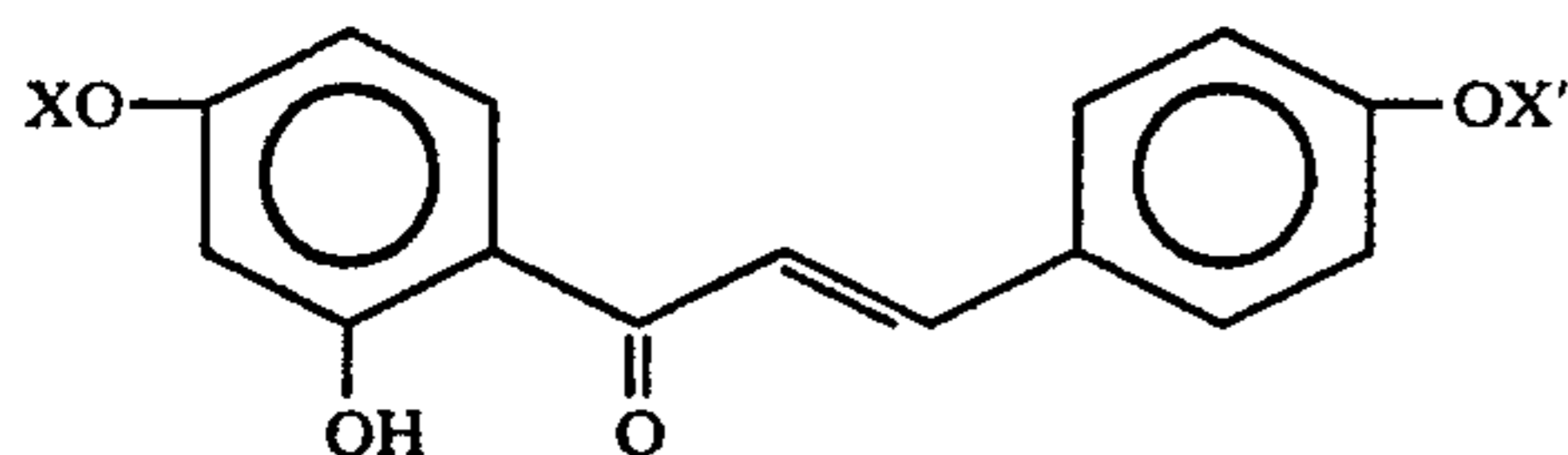
2'-Hydroxy-3,4,4'-tris(tetrahydropyranyloxy)chalcone
