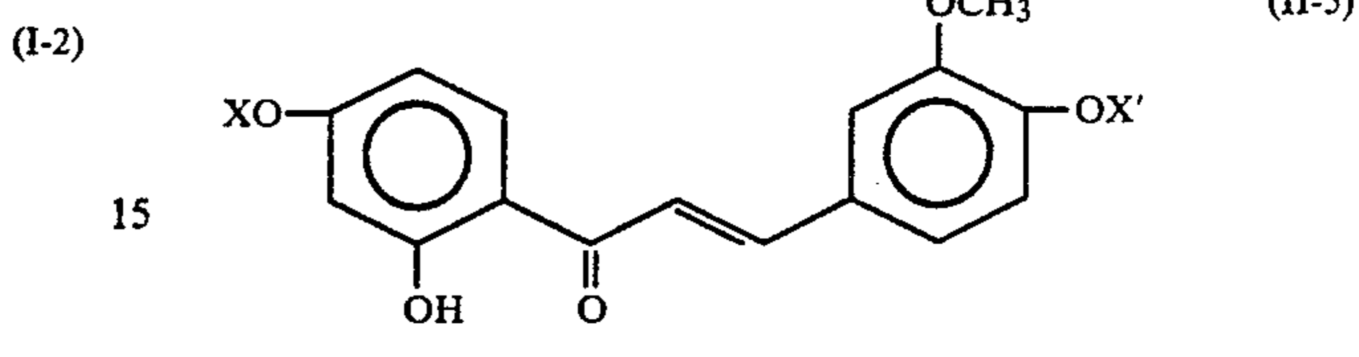
2'-Hydroxy-4-methoxy-3,4'-bis(tetrahydropyranyloxy)chalcone
