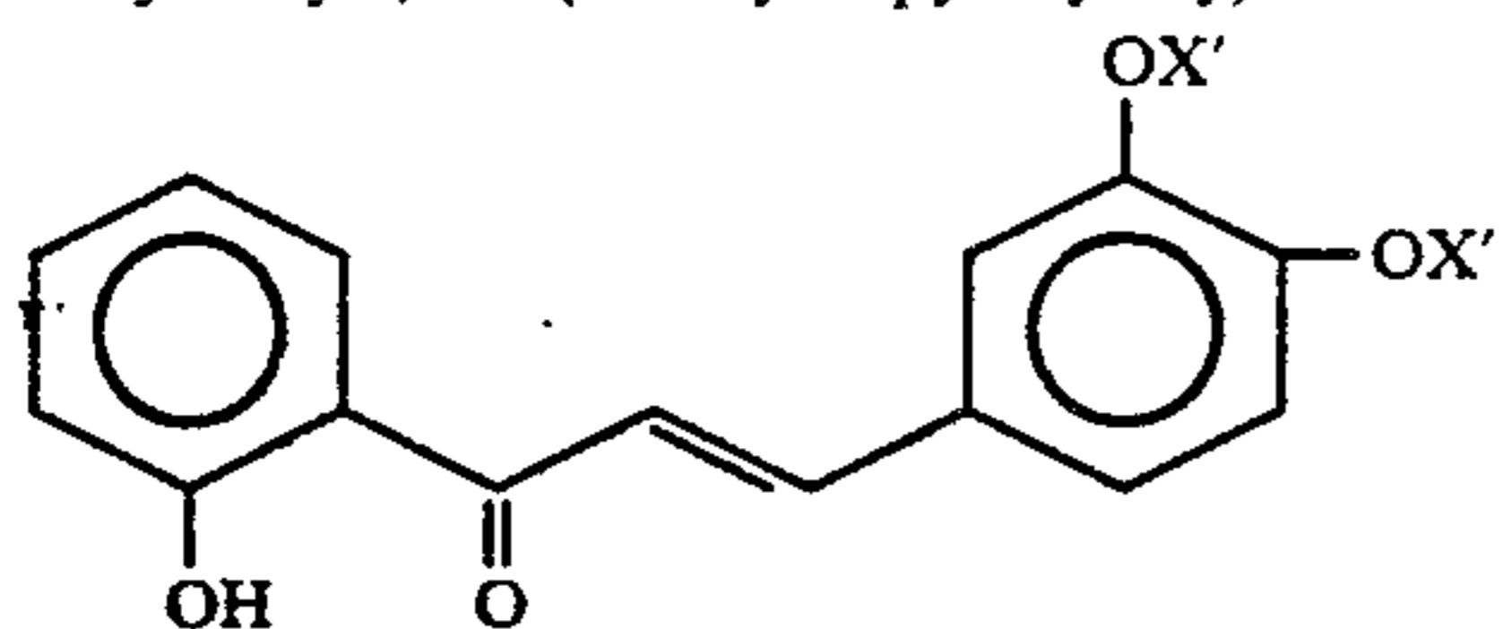
2'-Hydroxy-3,4-bis(tetrahydropyranyloxy)chalcone
