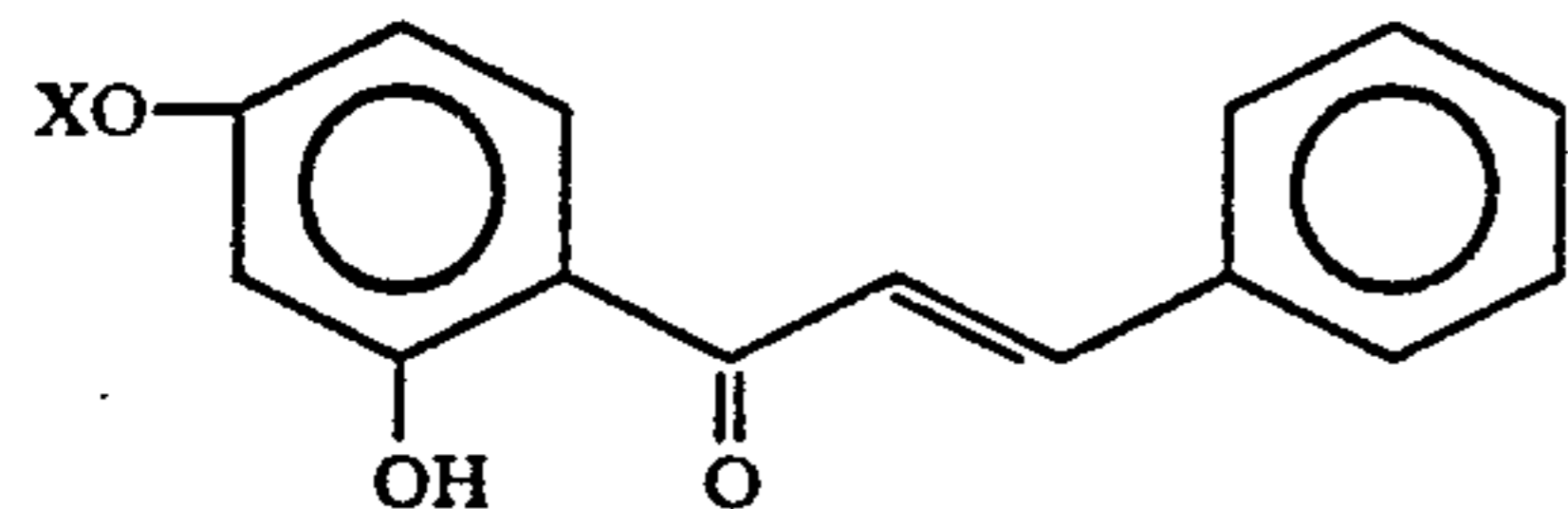
2'-Hydroxy-4,4-bis(tetrahydropyranyloxy)chalcone
