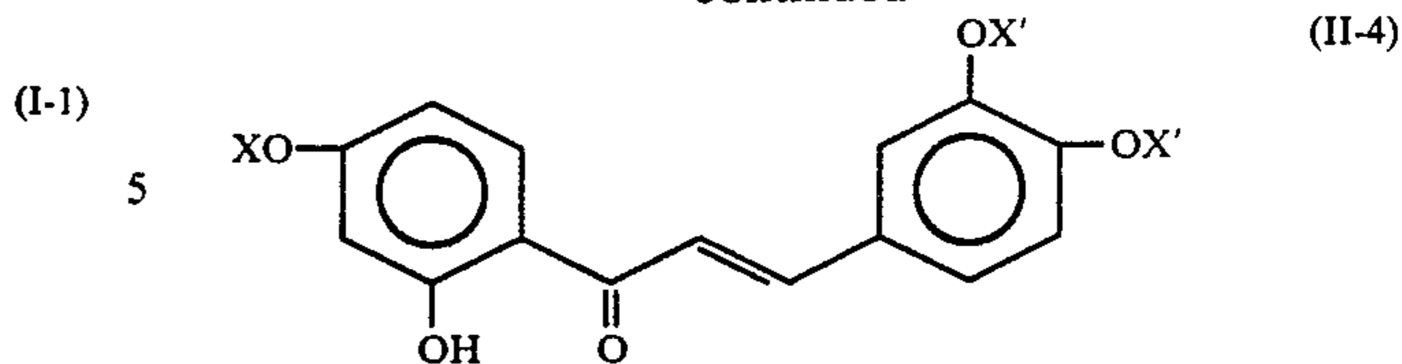
2'-Hydroxy-3-methoxy-4,4'-bis(tetrahydropyranyloxy)chalcone
