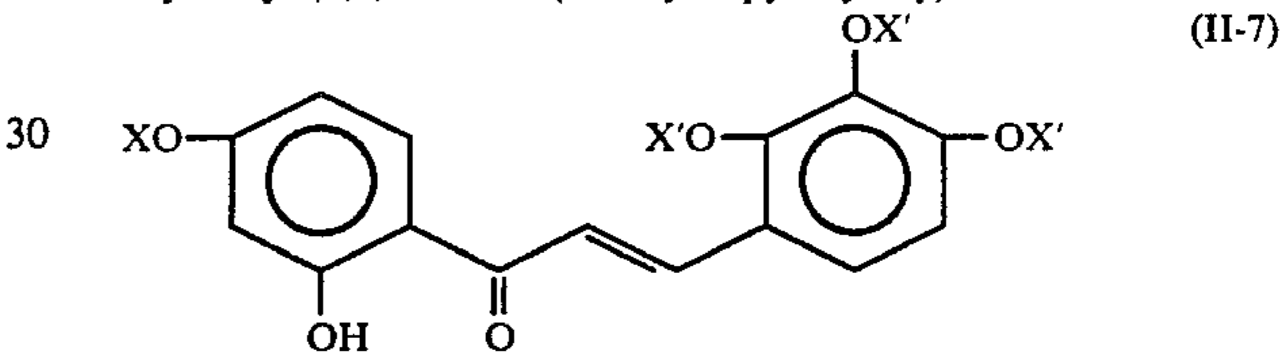
2'-Hydroxy-3,4,5,4'-tetrakis(tetrahydropyranyloxy)chalcone
