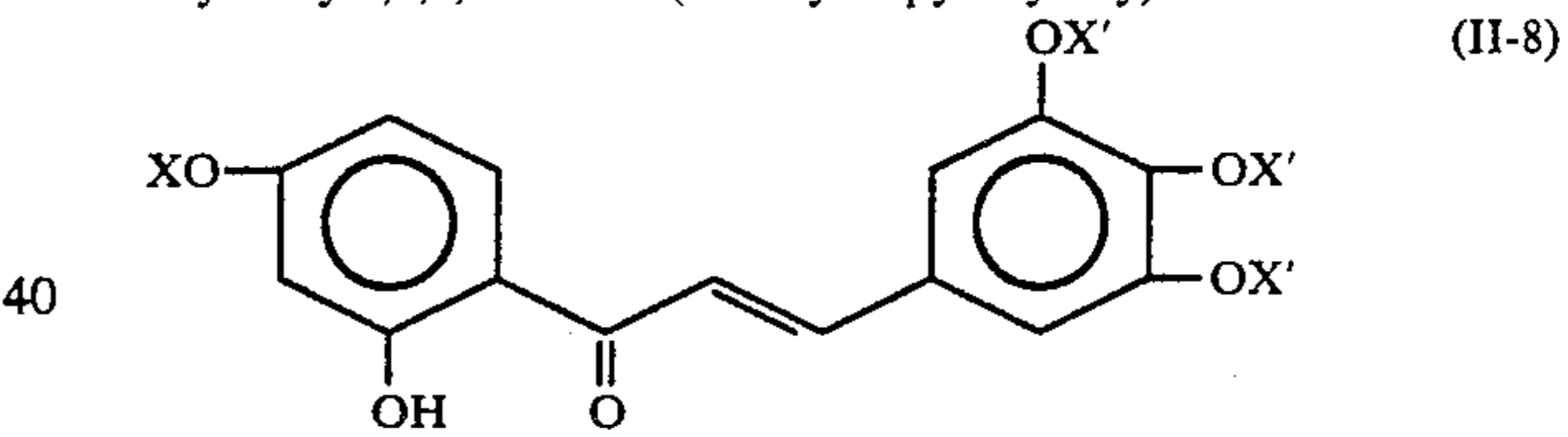
2'-Hydroxy-4',6'-bis(tetrahydropyranyloxy)chalcone
