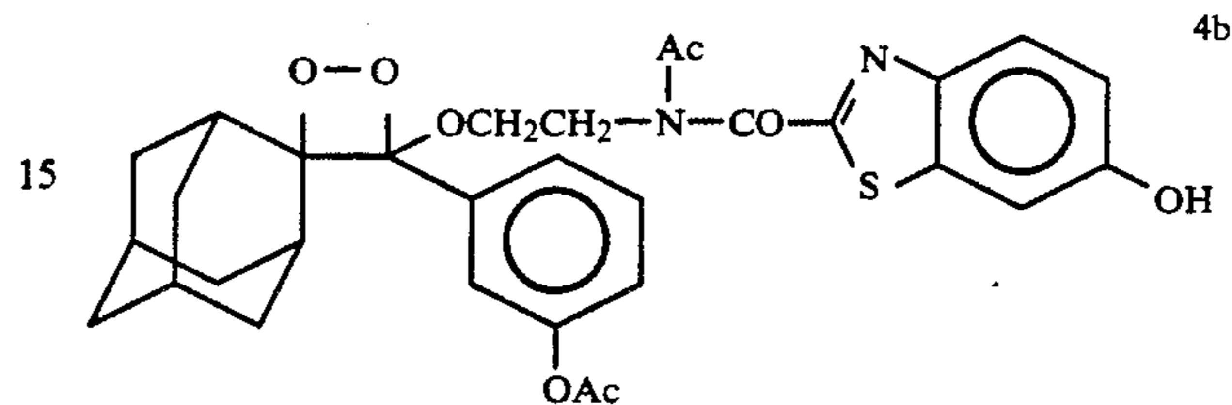
4-(3-Acetoxyphenyl)-4-(2-(O-fluorescein)ethoxy)spiro[1,2-dioxetane-3,2'-adamantane] (6)
