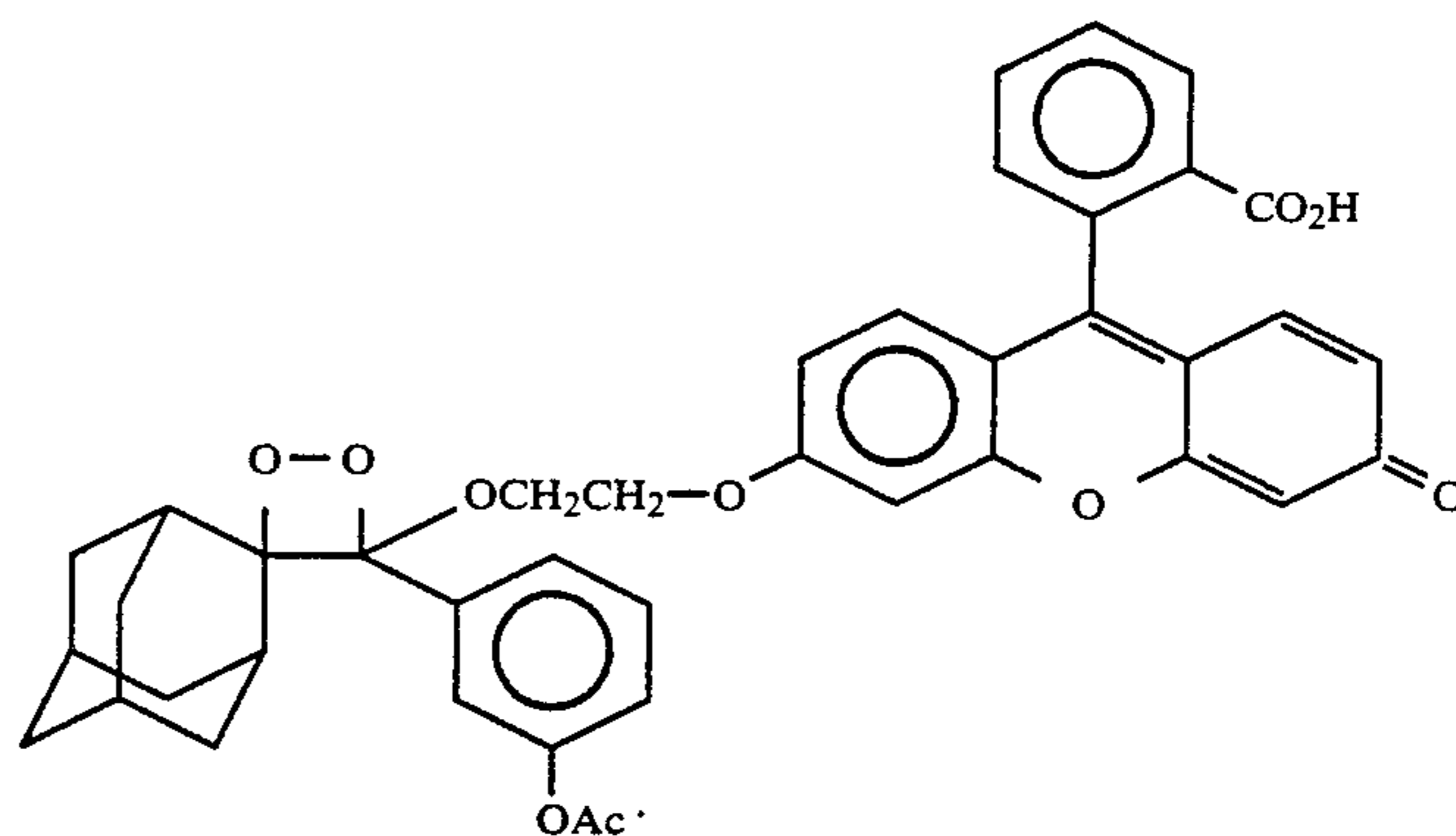
4-(2-(N-(6-hydroxybenzothiazole-2-carbonyl)amino)ethoxy)-4-(3-β-D-galactopyranosylphenyl)spiro[1,2-dioxetane-3,2'-adamantane] (8)
