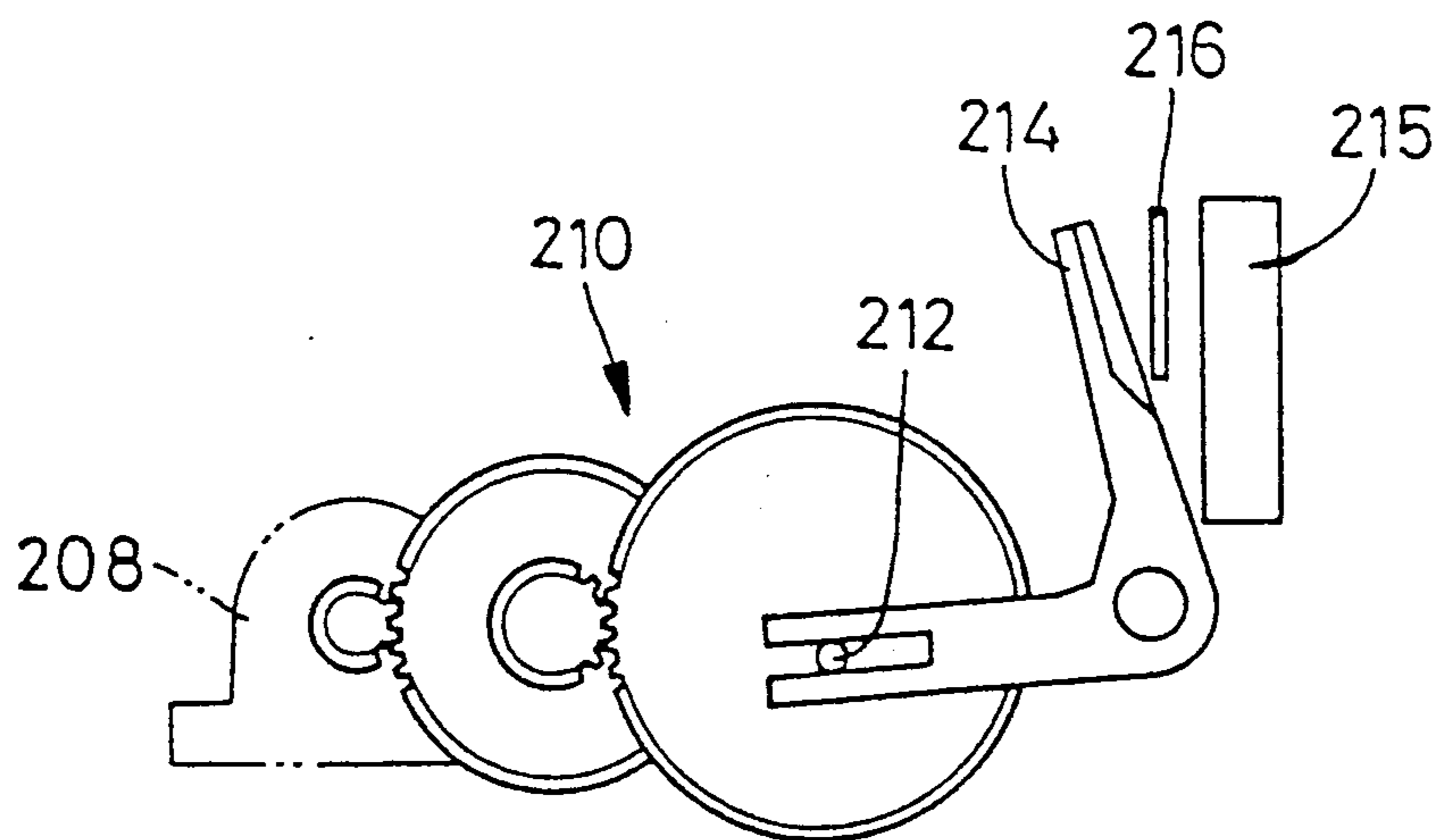
FIG. 16 PRIOR ART
