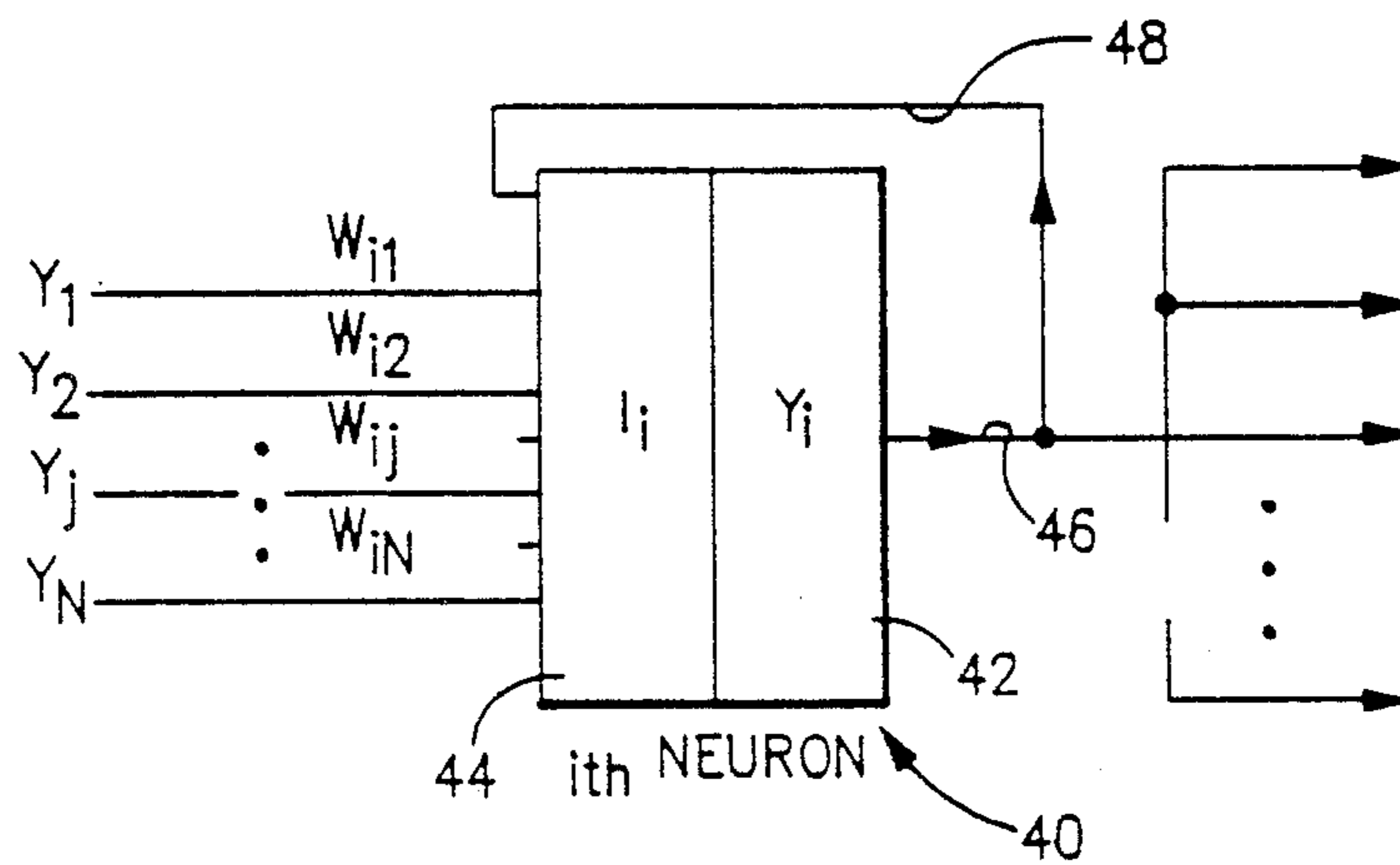
FIG.1 Prior Art
