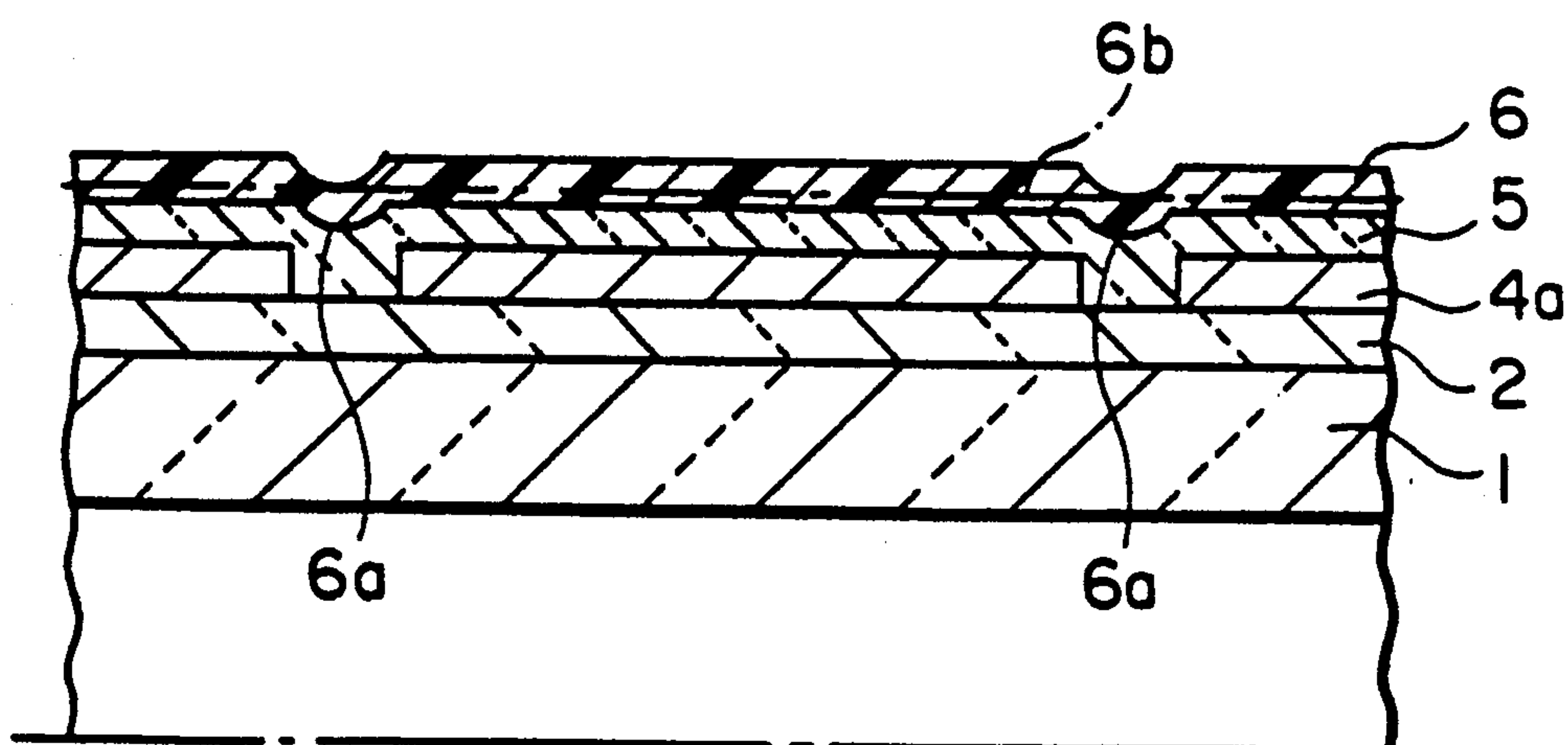
FIG. 9 (PRIOR ART)
