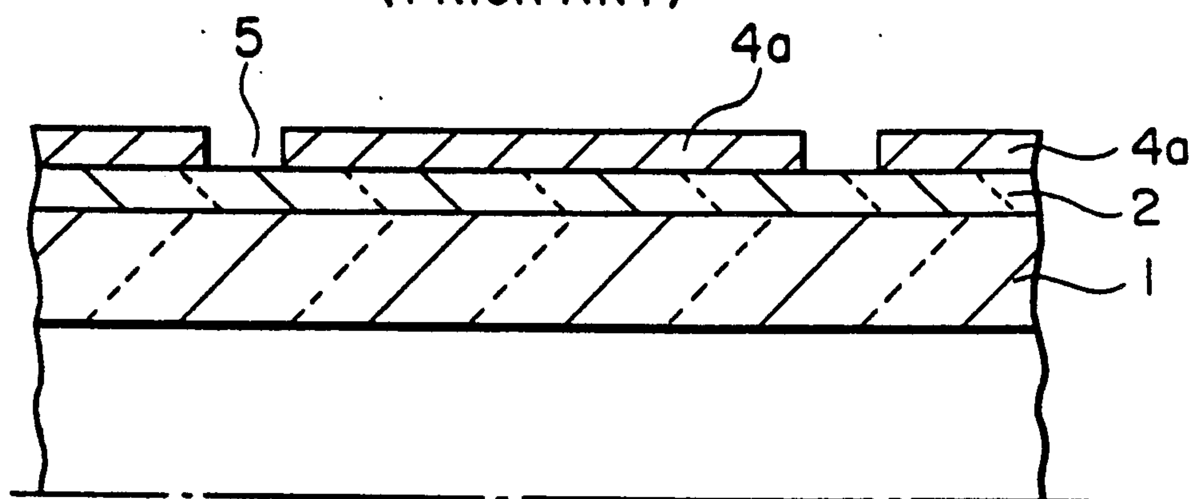
FIG. 8 (PRIOR ART)
