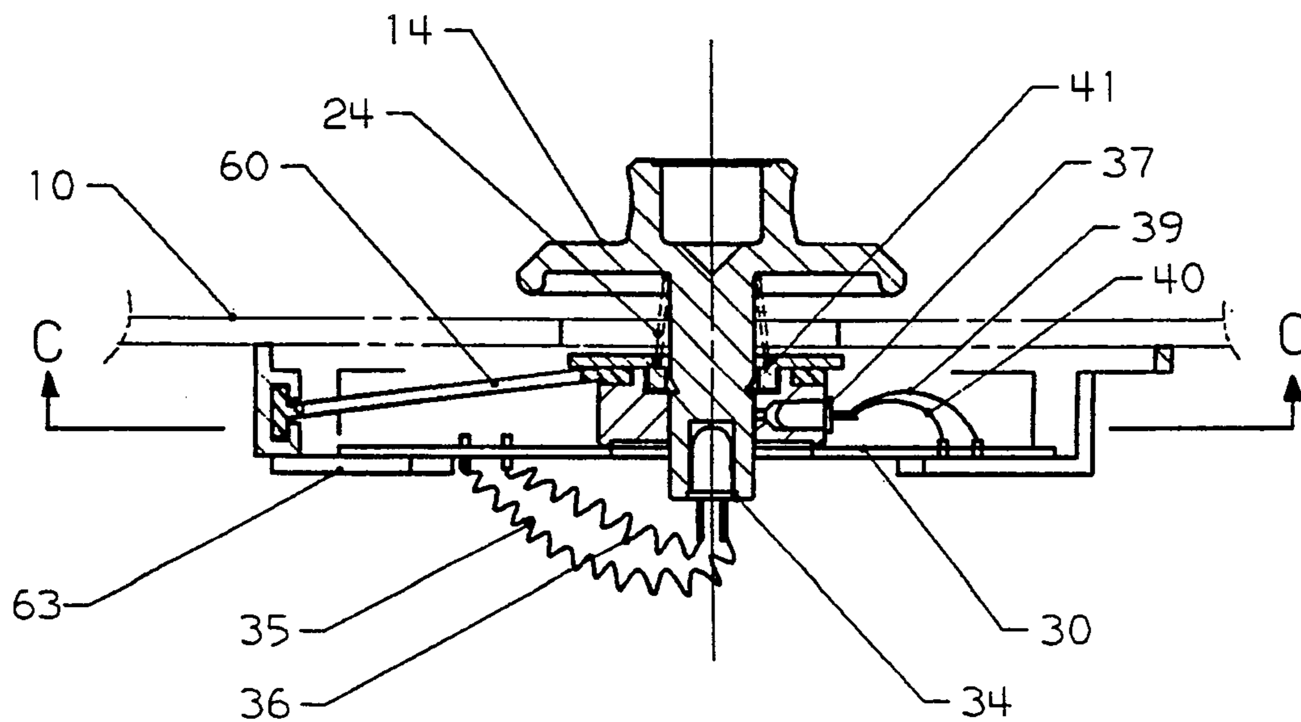
SECTION B-B - FIG 8
