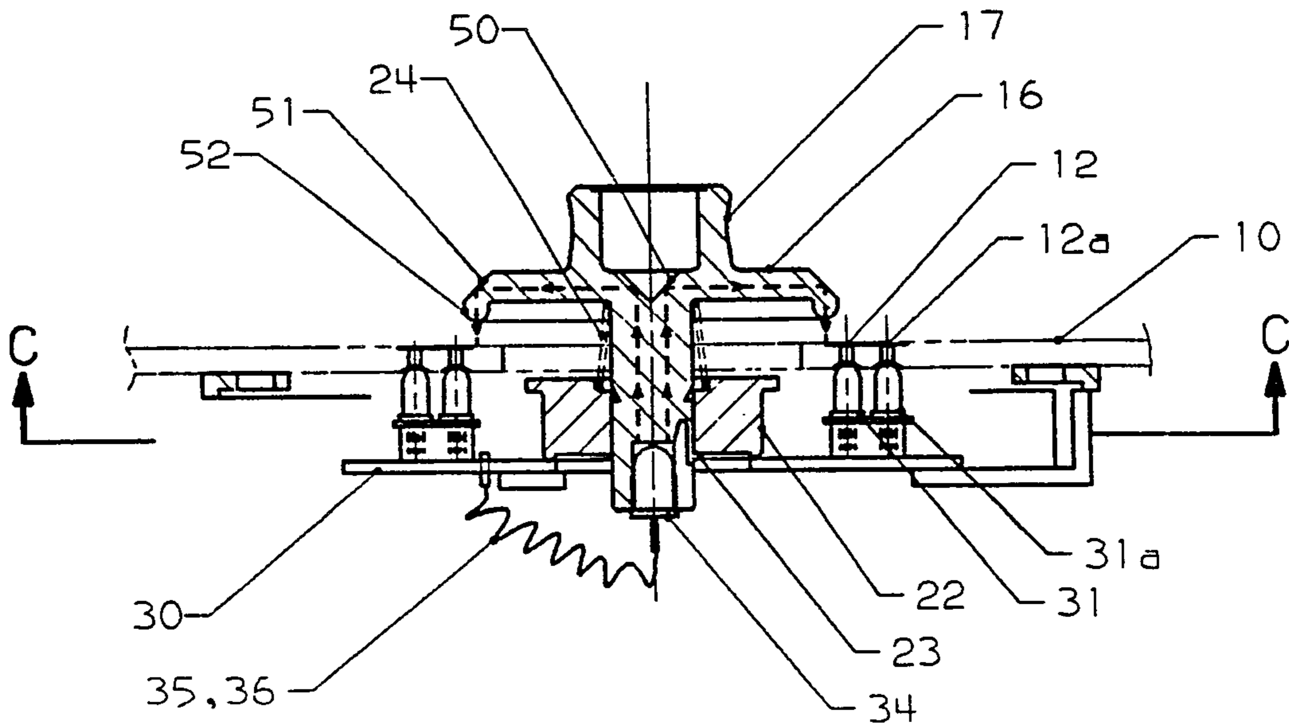
SECTION A-A - FIG 3
