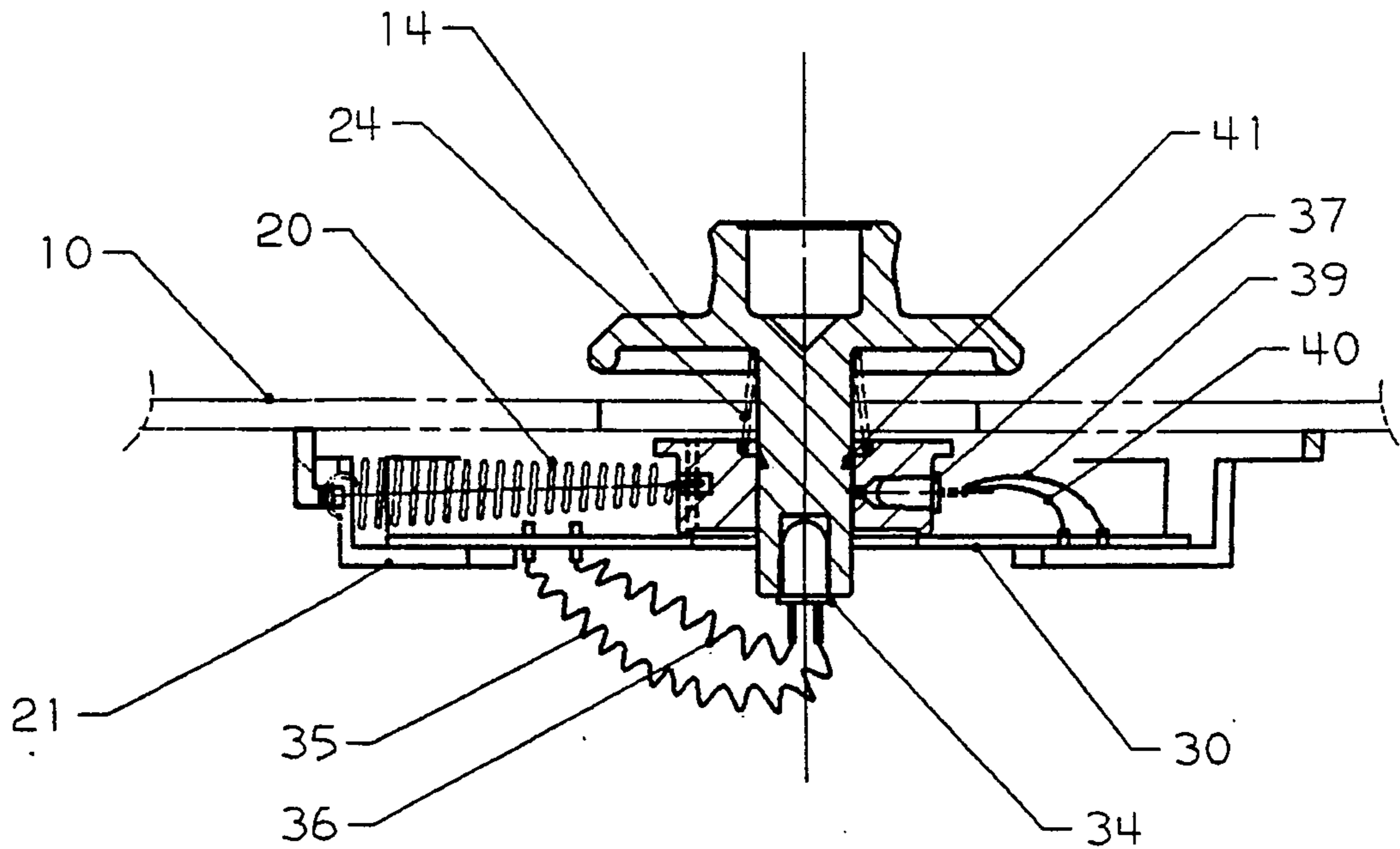
SECTION B-B - FIG 4
