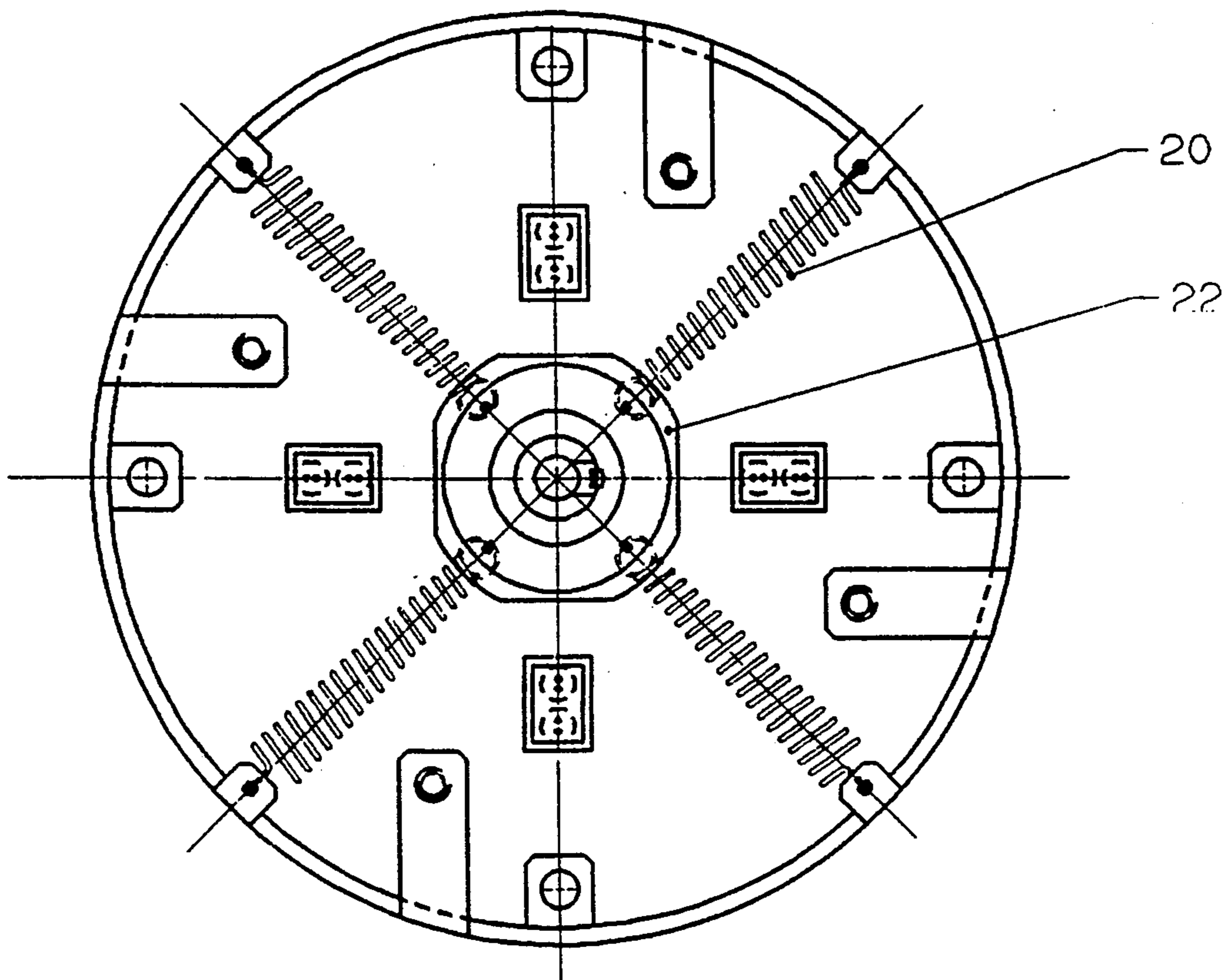
SECTION C-C - FIG 5
