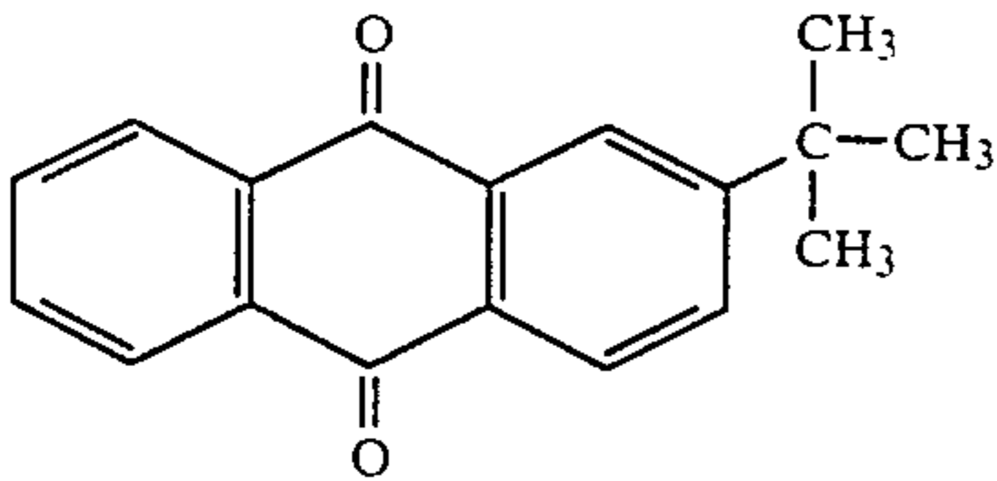
2-t-butyl anthraquinone
