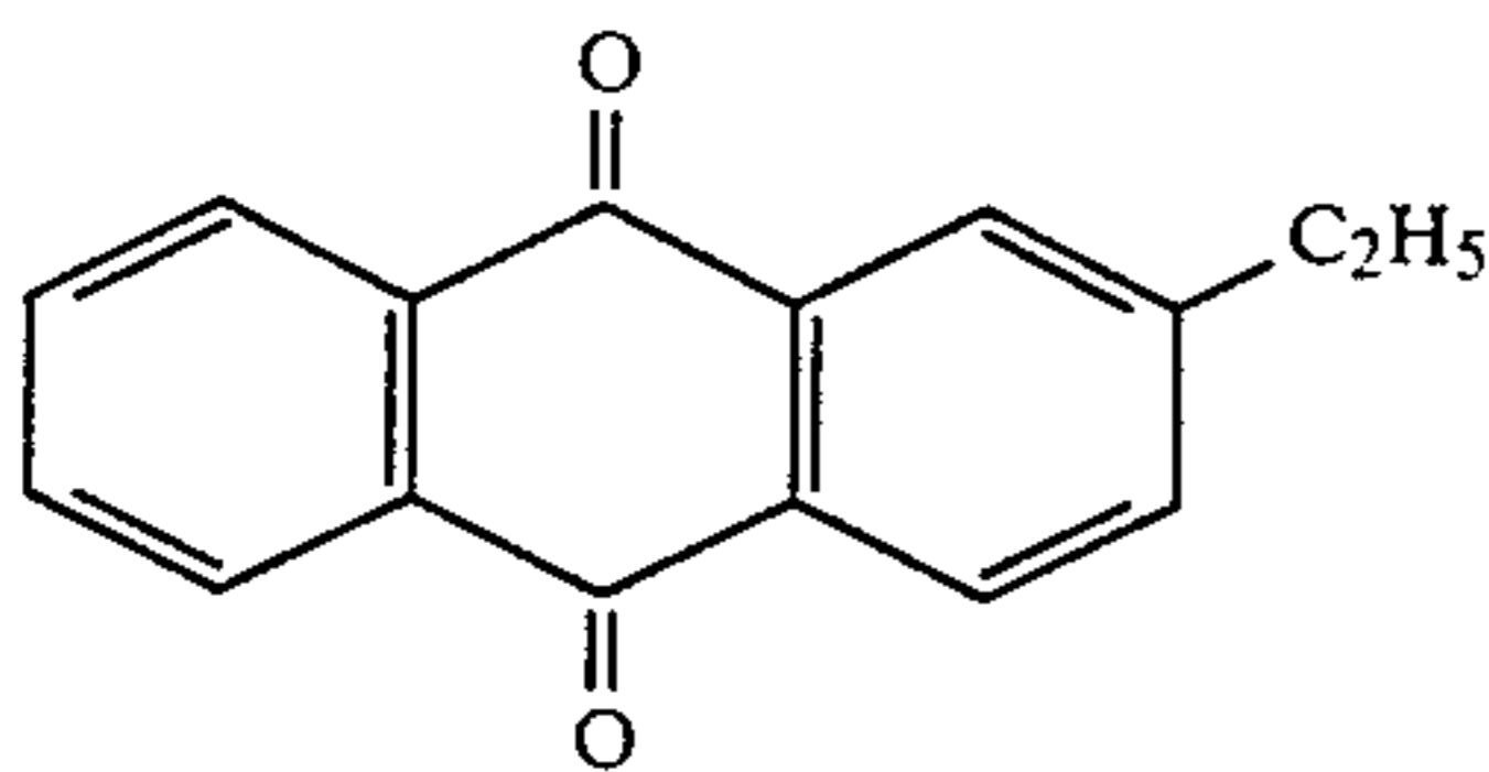
2-ethyl anthraquinone
