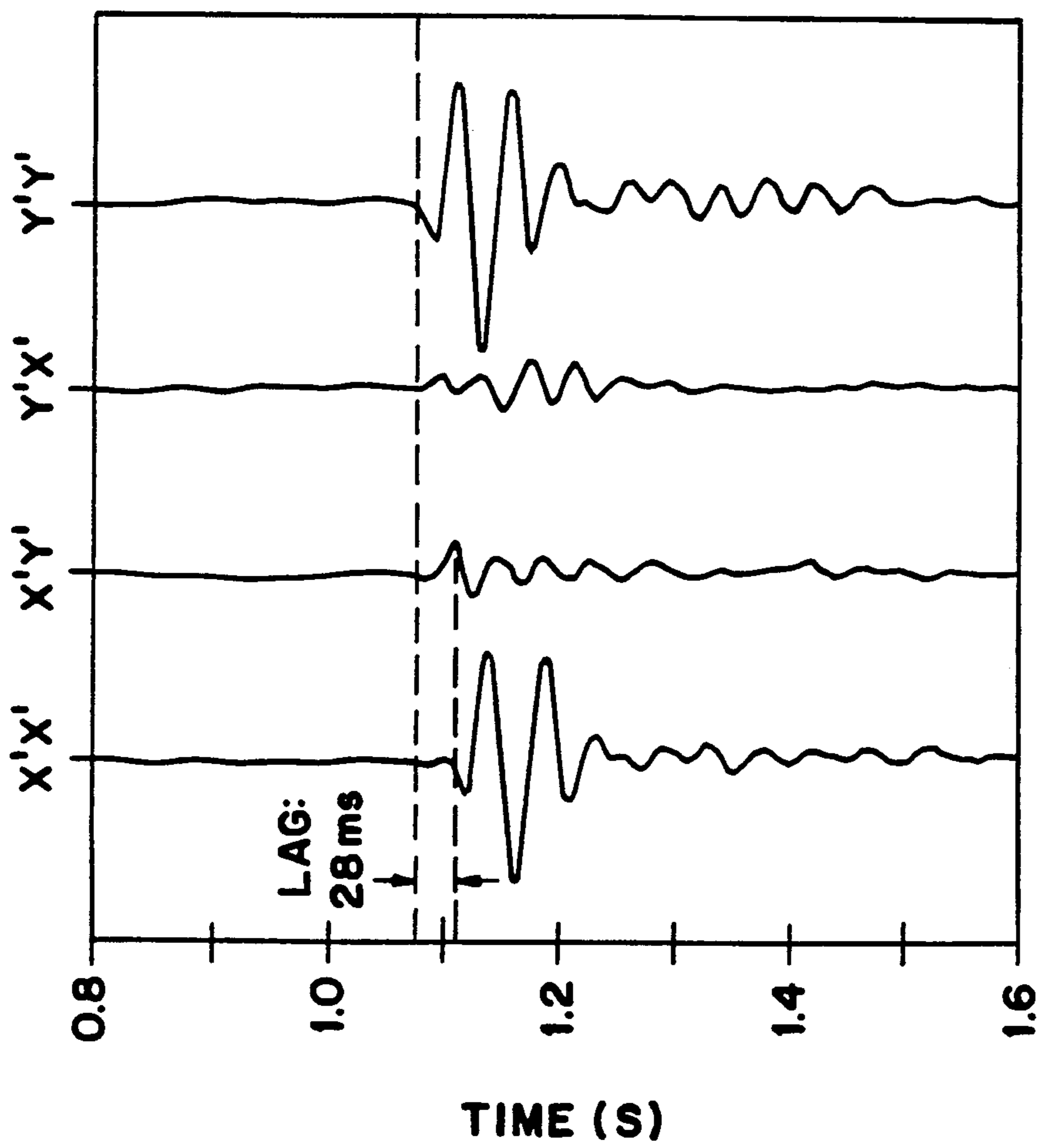
TRACES OF FIGURE 4 AFTER ROTATION
