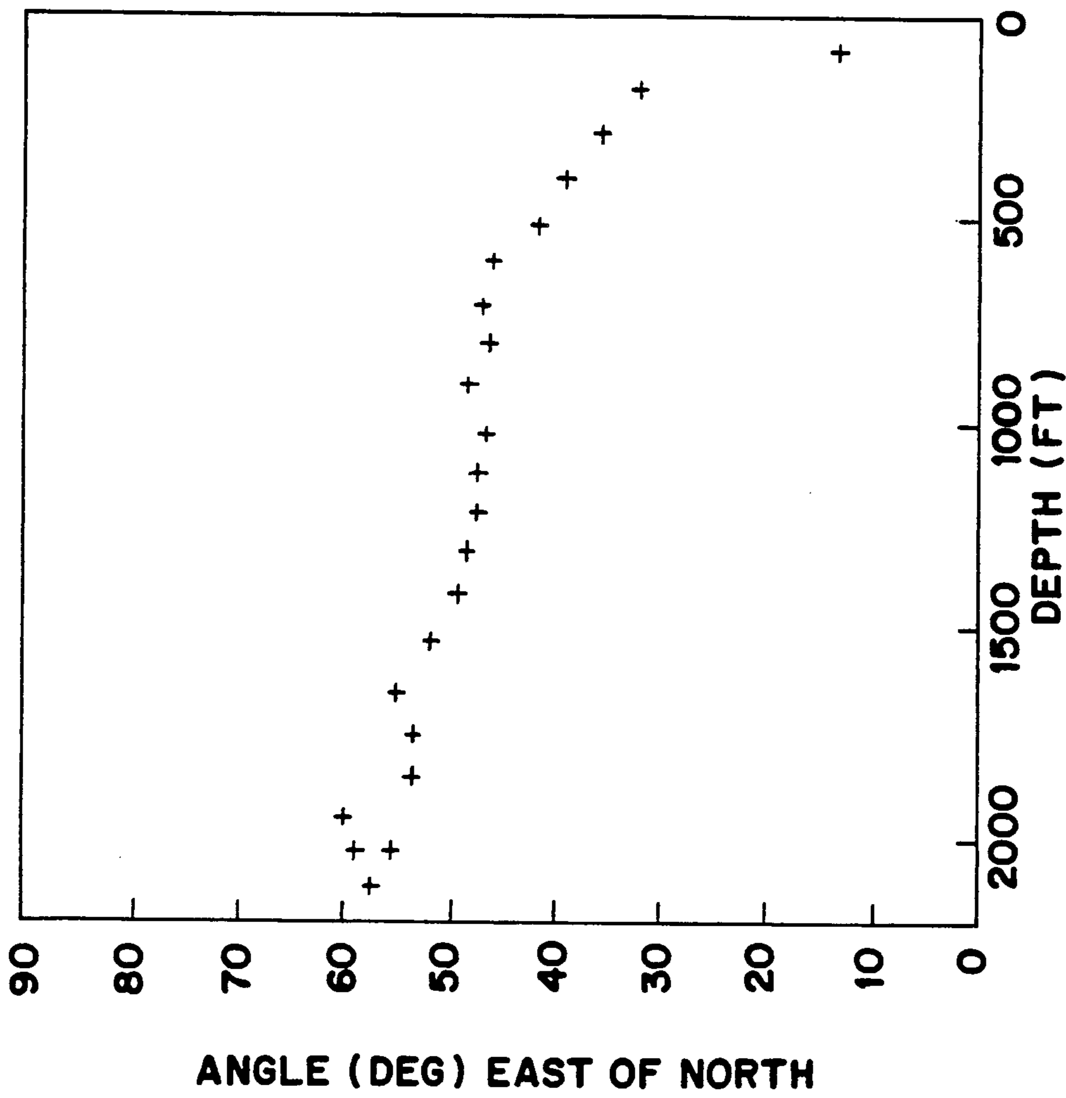
POLARIZATION AZIMUTHS OF THE FAST S-WAVE BEFORE LAYER STRIPPING FIG-7
