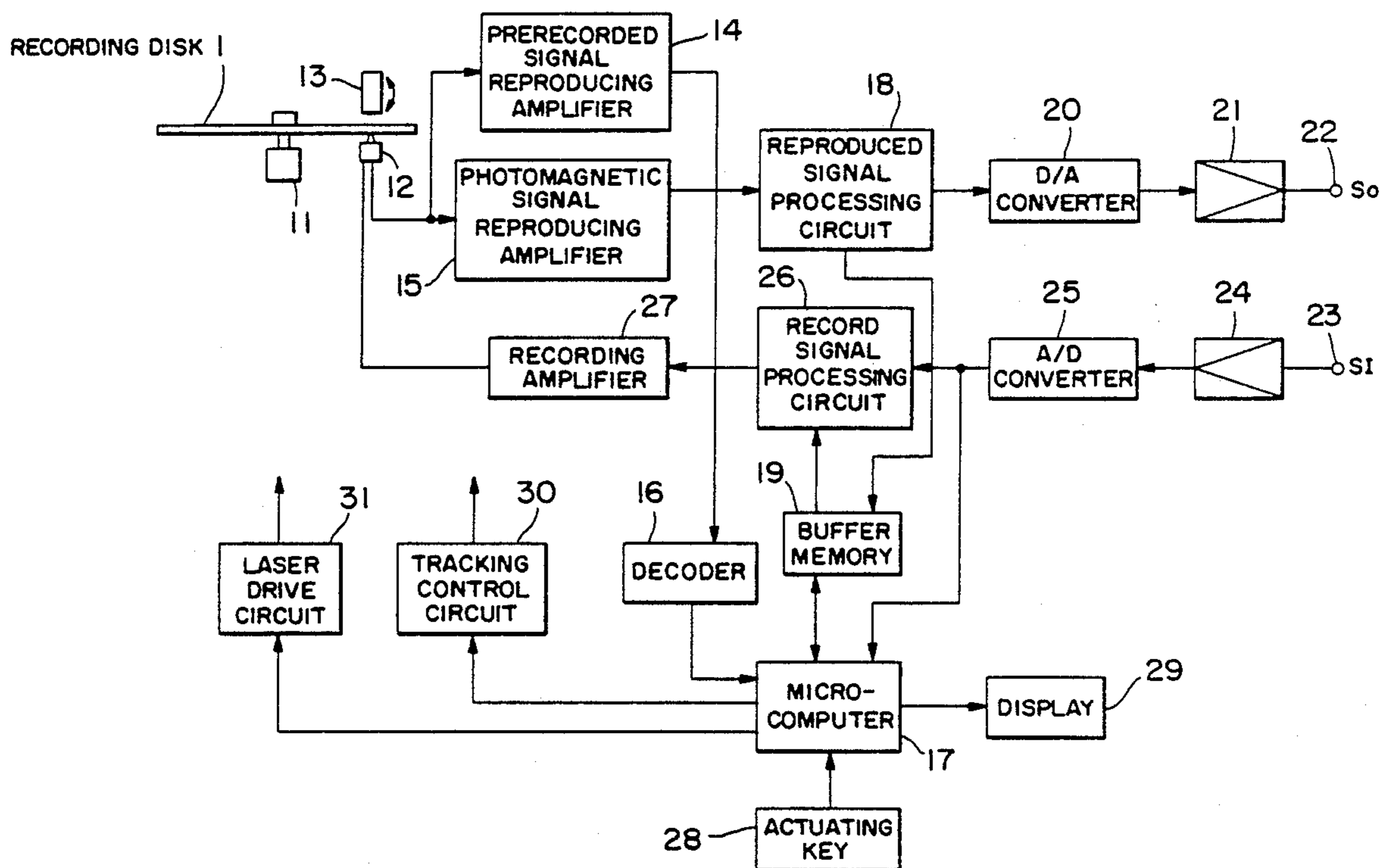
CONSTRUCTION OF A DISK RECORDING/REPRODUCING APPARATUS
