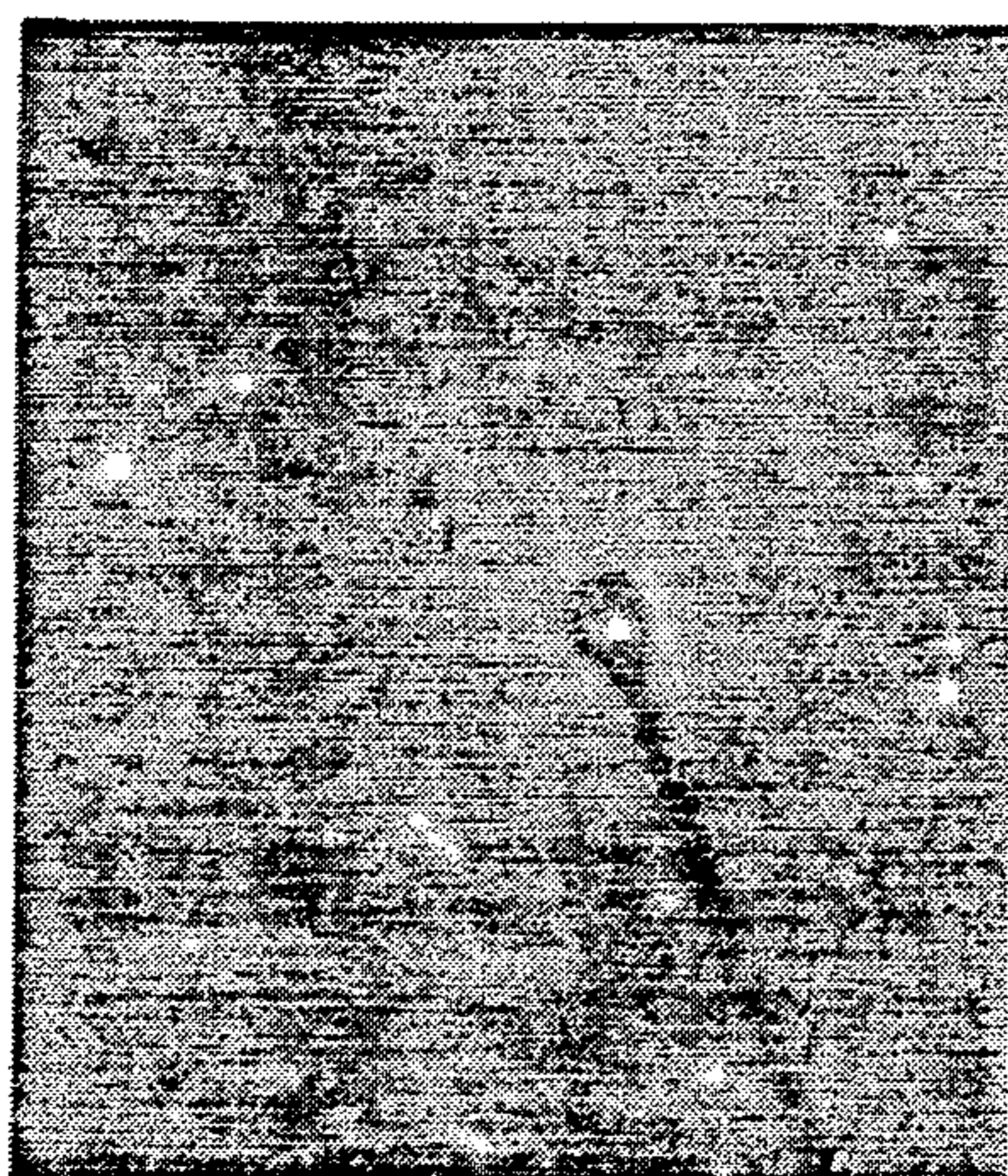
DIFFRACTION PATTERN
