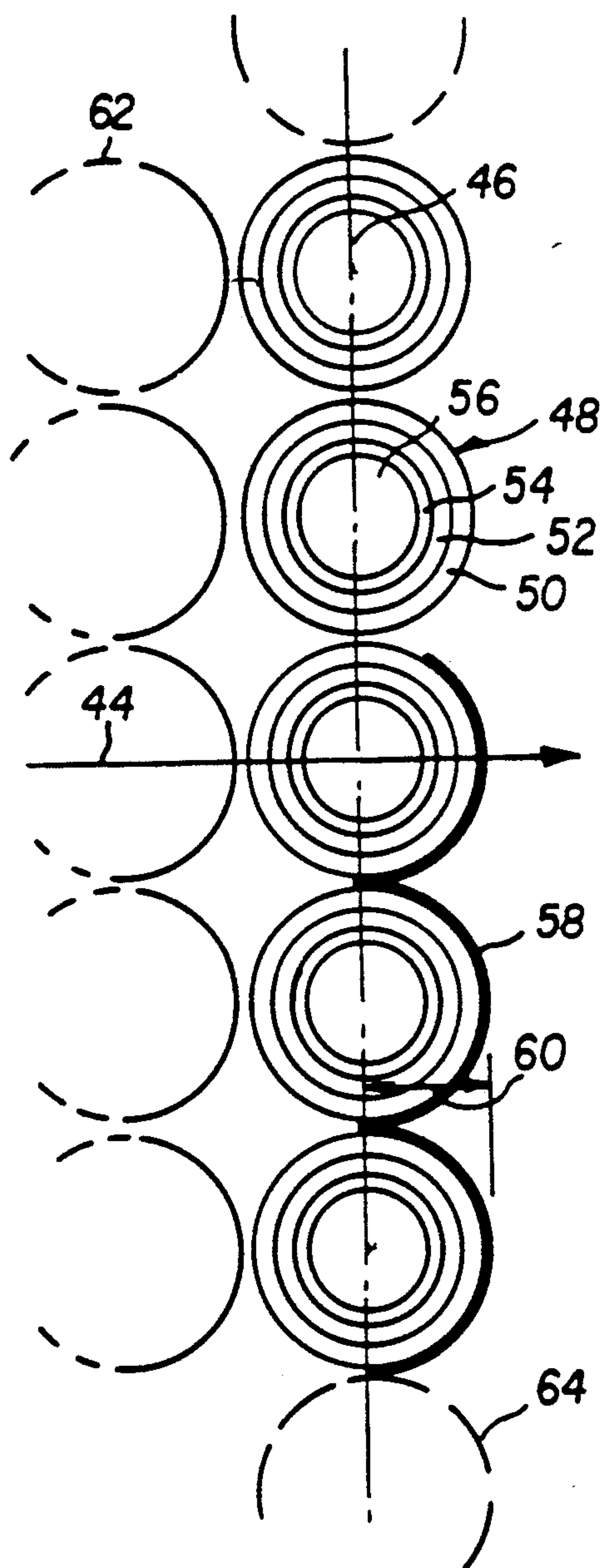
FIG. 3 (prior art)
