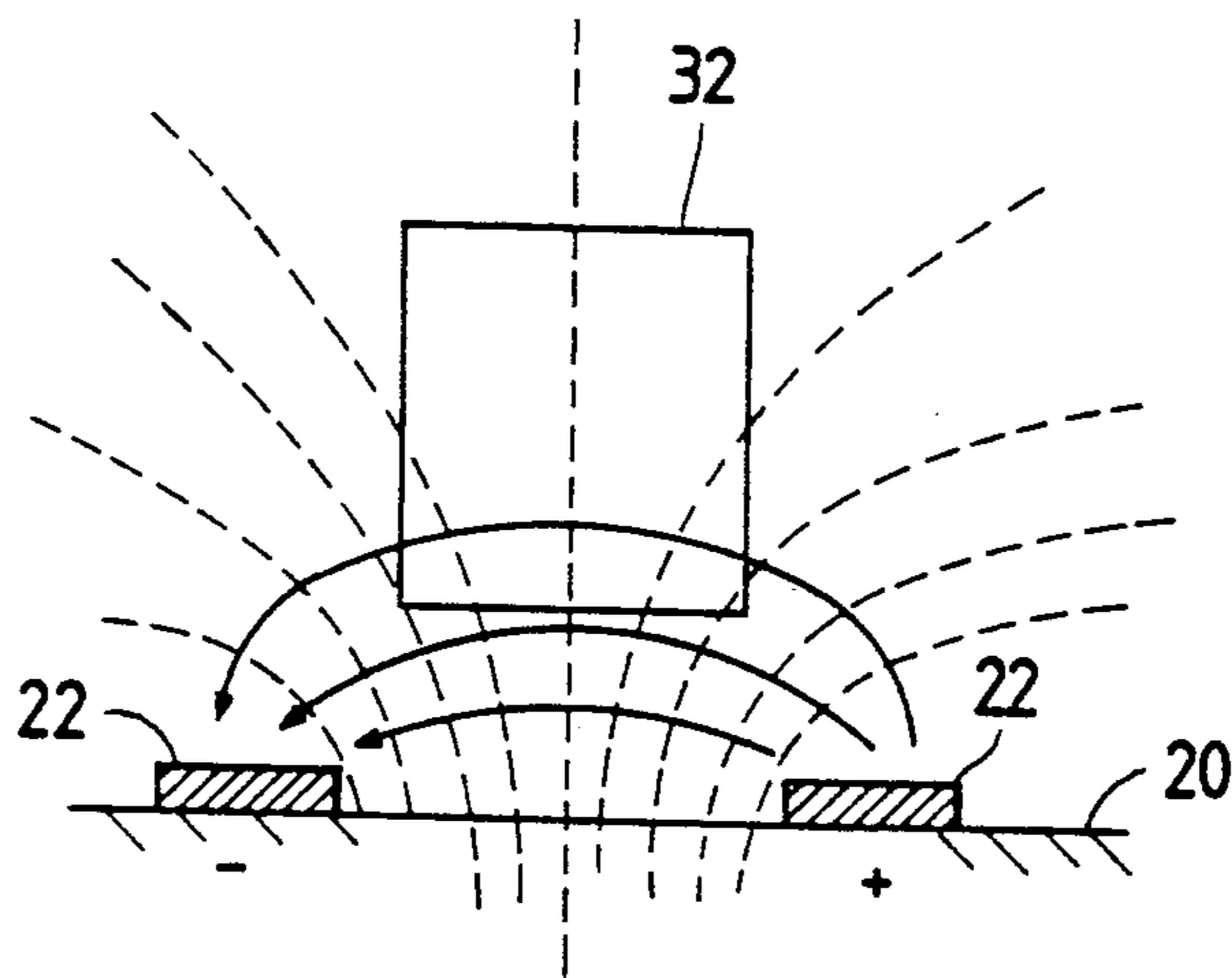
FIG. 15 PRIOR ART
