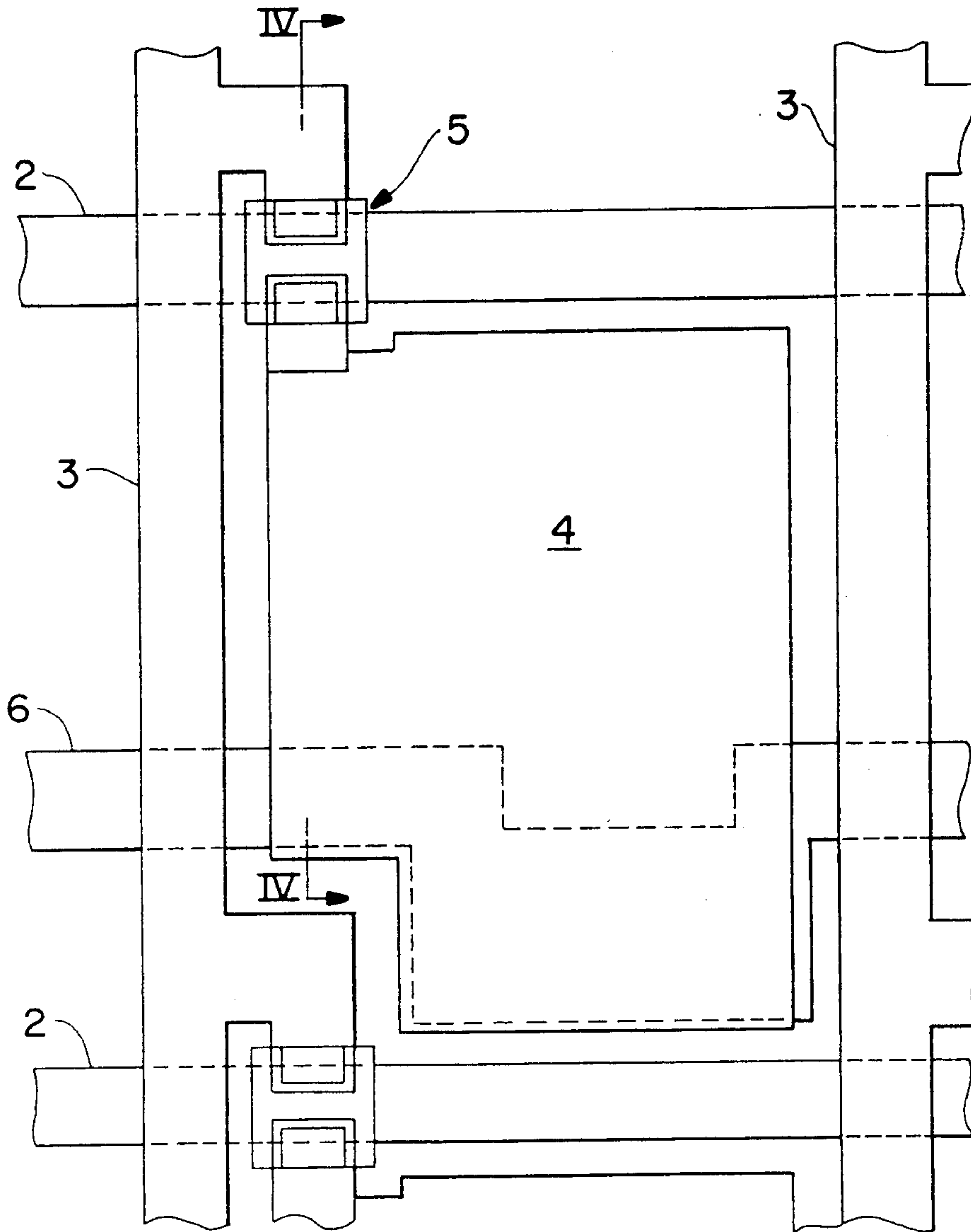
FIG. 3 PRIOR ART
