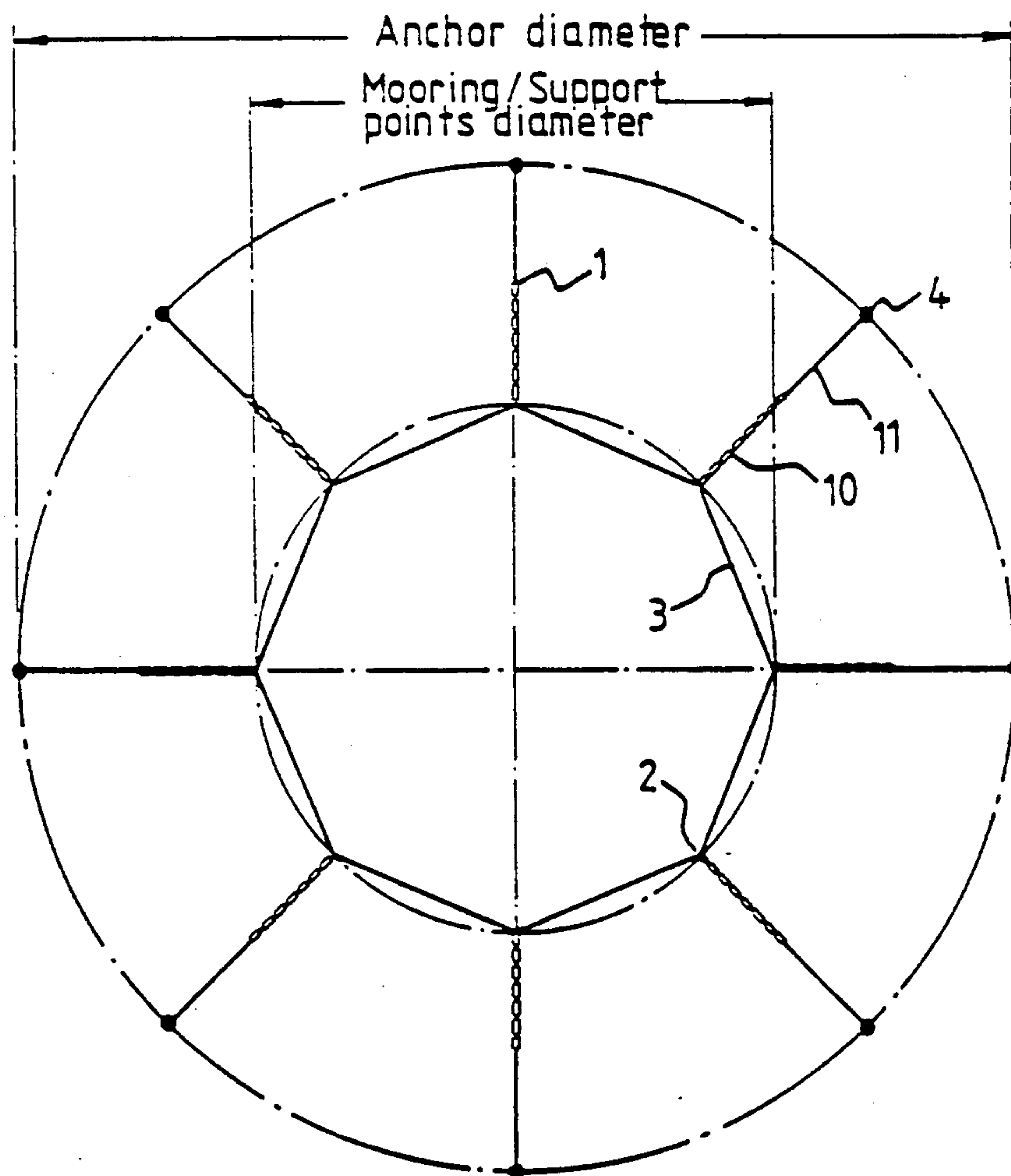
FIG. 3. PLAN OF MOORING/SUPPORT SYSTEM
