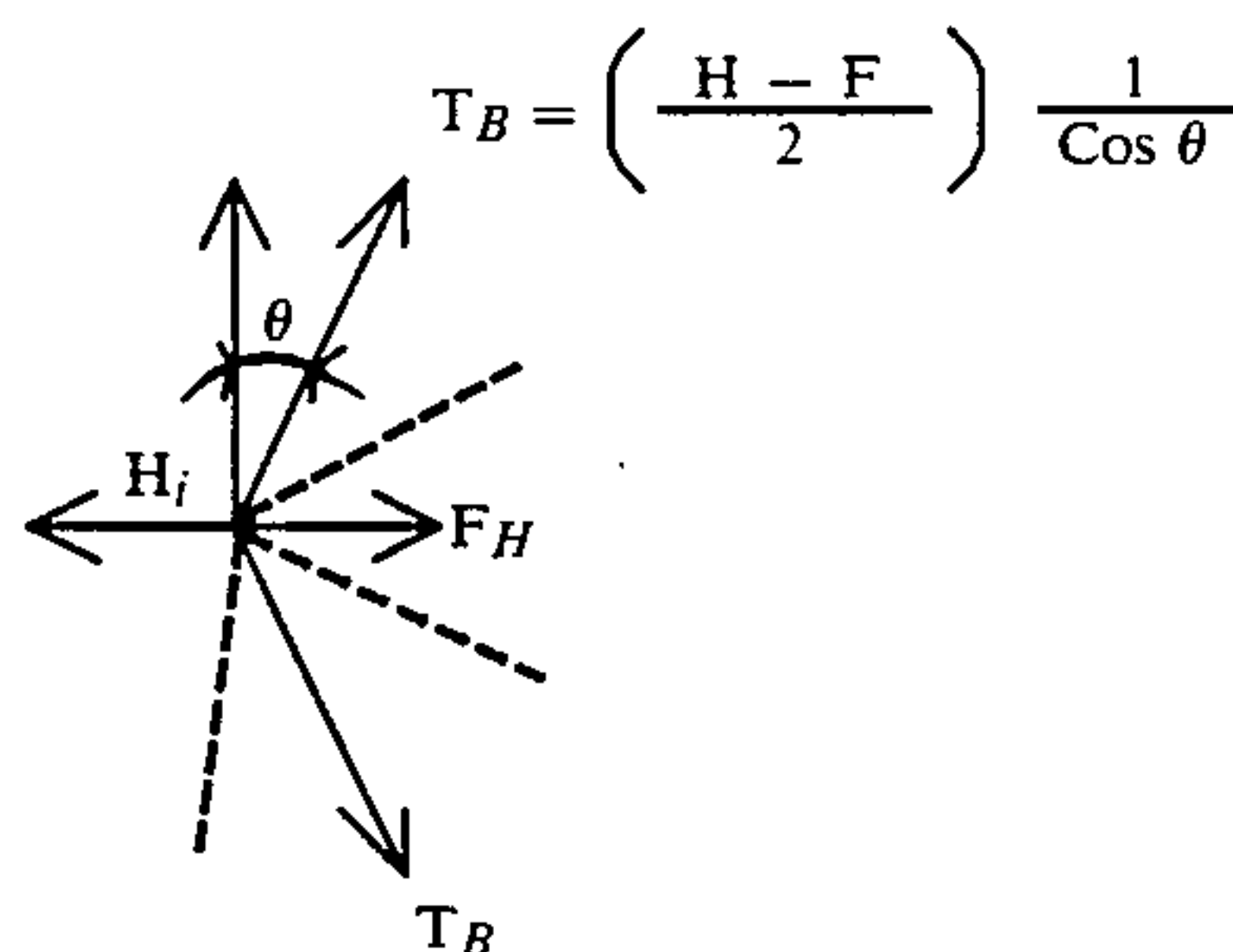
Stress in Bridle Element During operation
