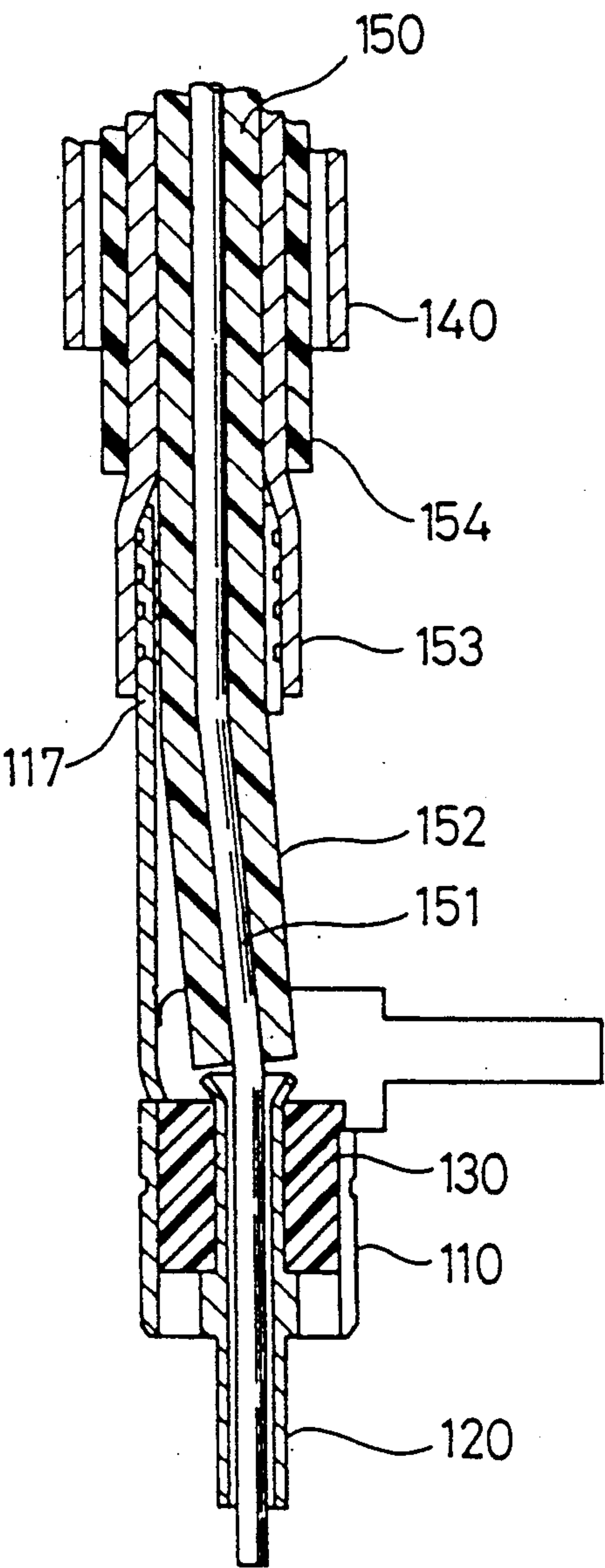
FIG. 8 PRIOR ART
