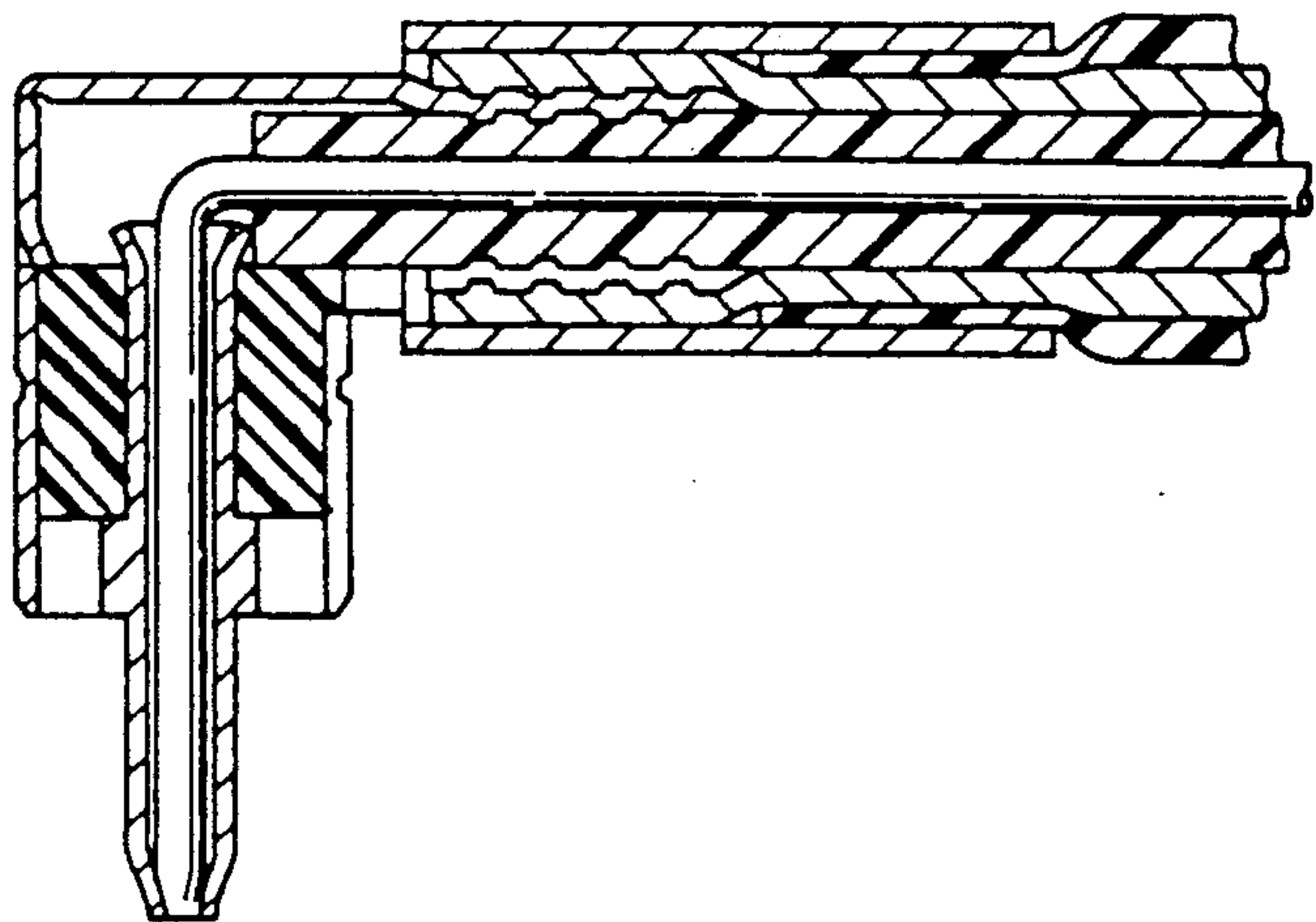
FIG. 9 PRIOR ART
