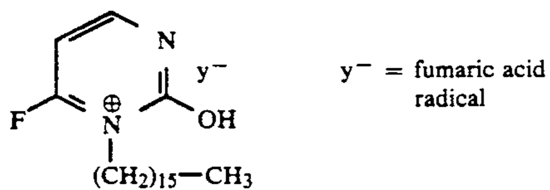
(2-hydroxy-5-fluoro-hexadecylpyrimidinium fumarate)
