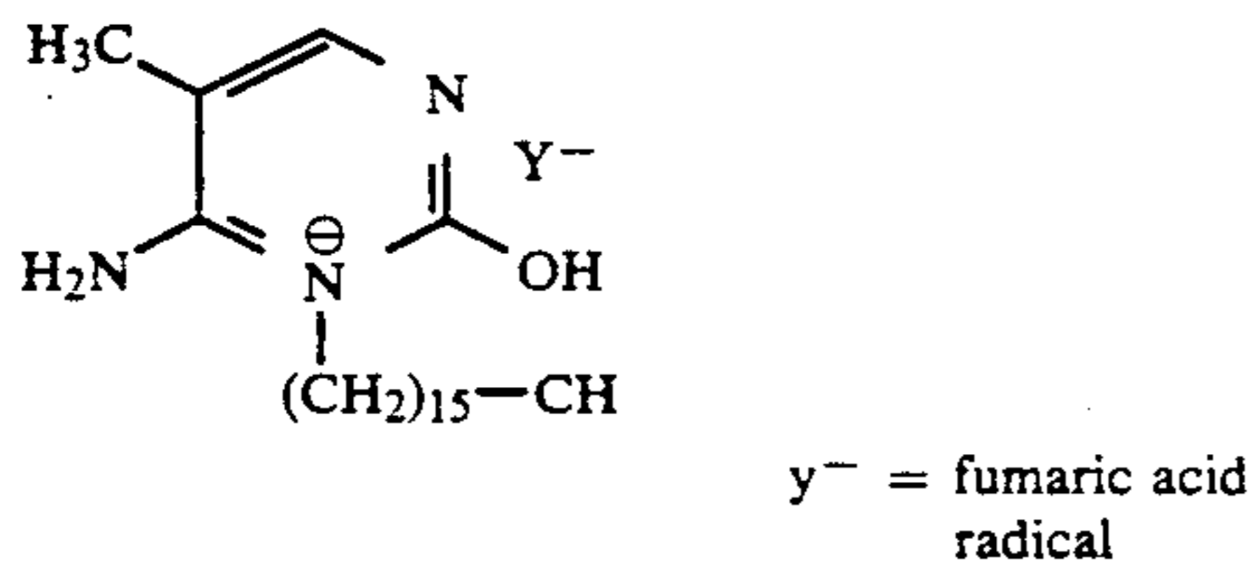
(2-hydroxy-5-methyl-6-amino-hexadecylpyrimidinium fumarate)
