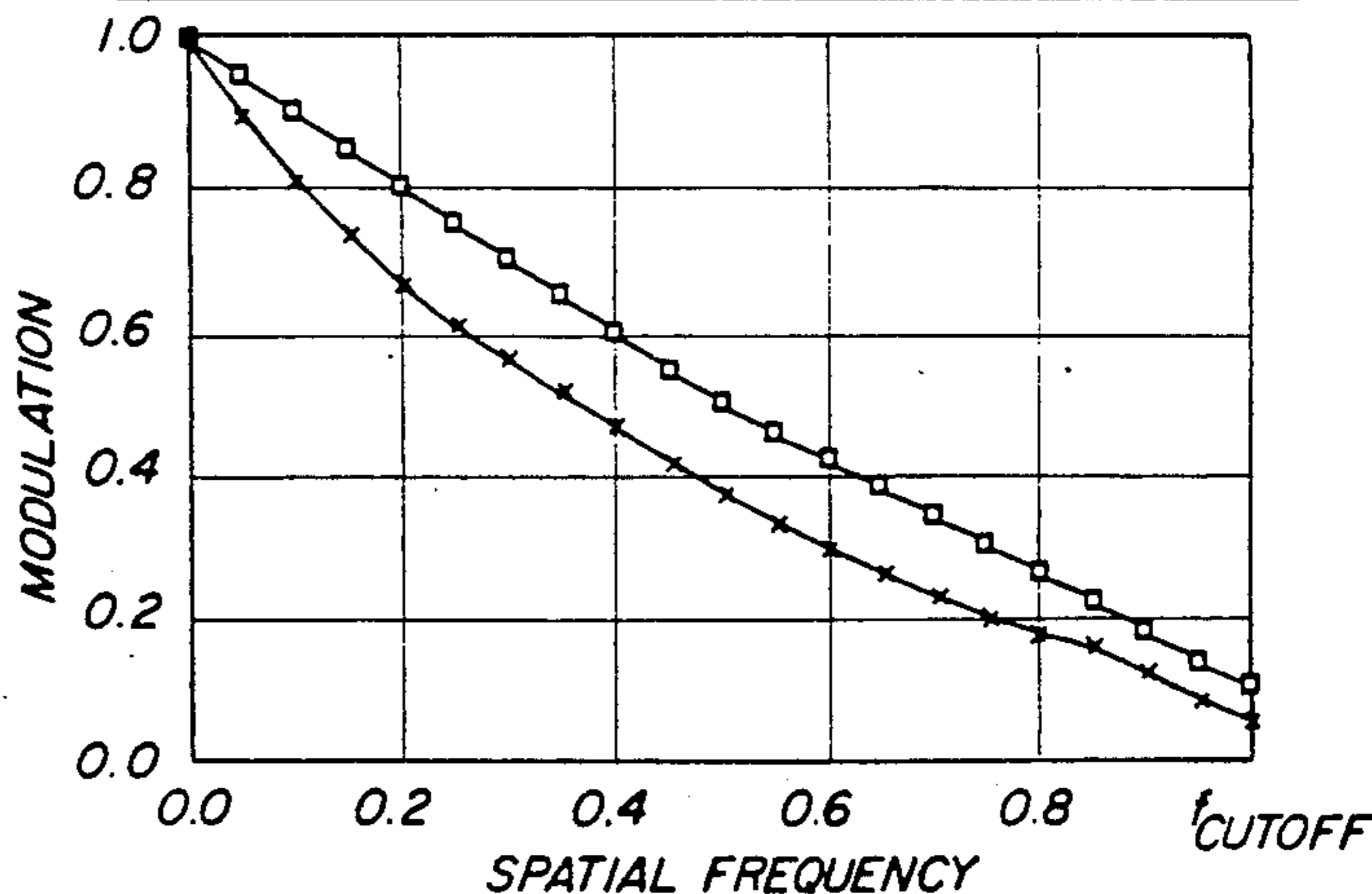
HYPERBOLA -1.6858 MODULATION TRANSFER FUNCTION | × LENS PERFORMANCE □ DIFFRACTION LIMIT
