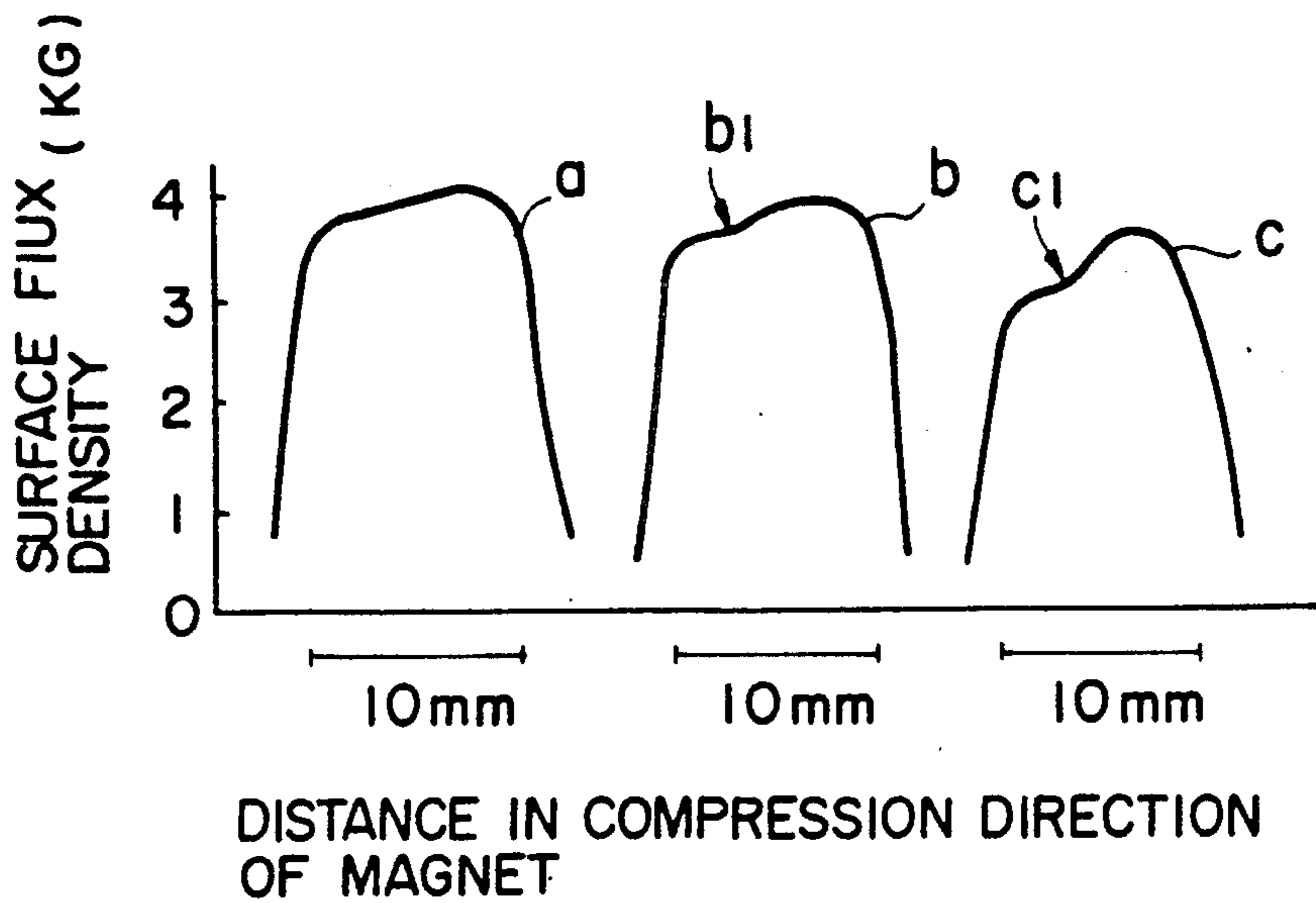
FIG. 6 (PRIOR ART)
