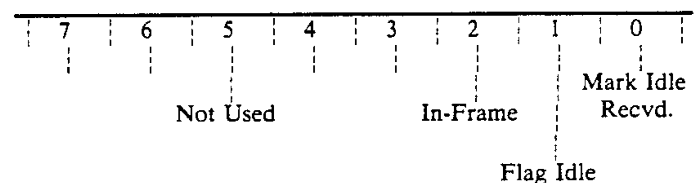
RECEIVE LINK STATUS REGISTER
