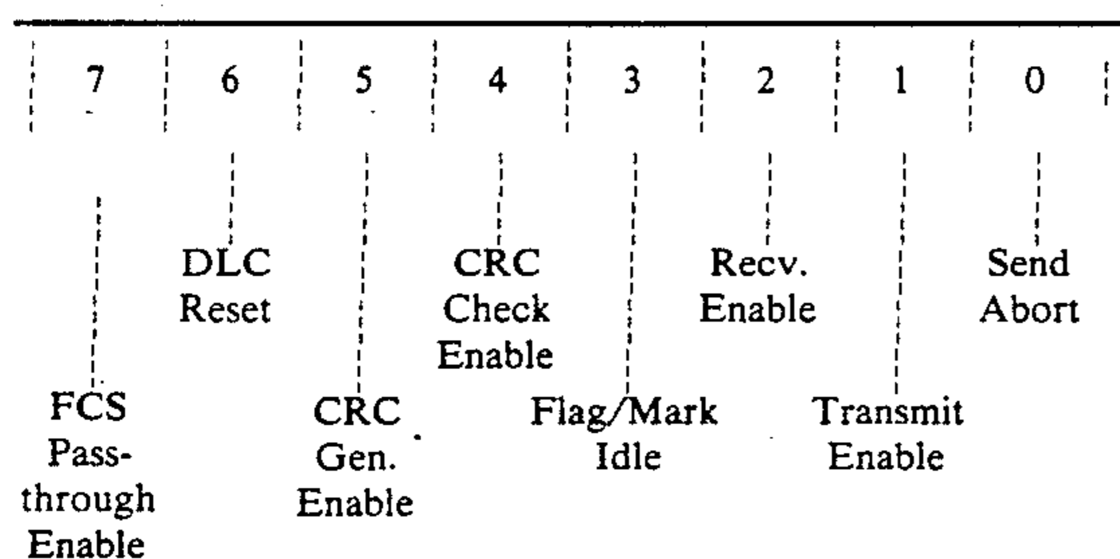
DLC COMMAND/CONTROL REGISTER
