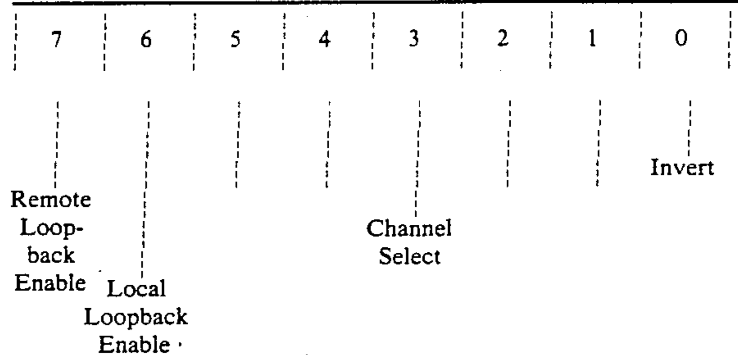
SERIAL BUS PORT CONTROL REGISTER
