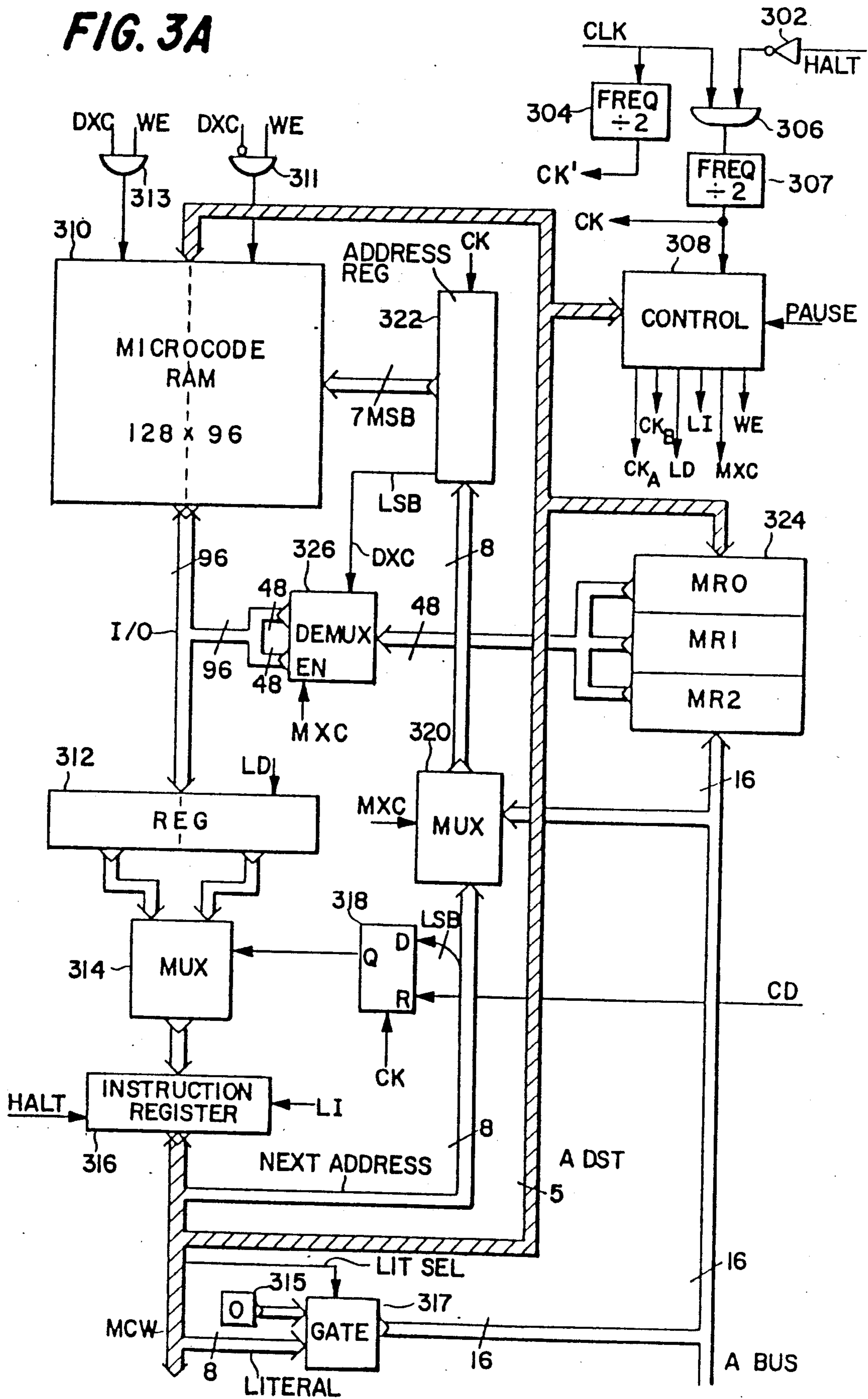
MICROCODE RAM AND SEQUENCER
