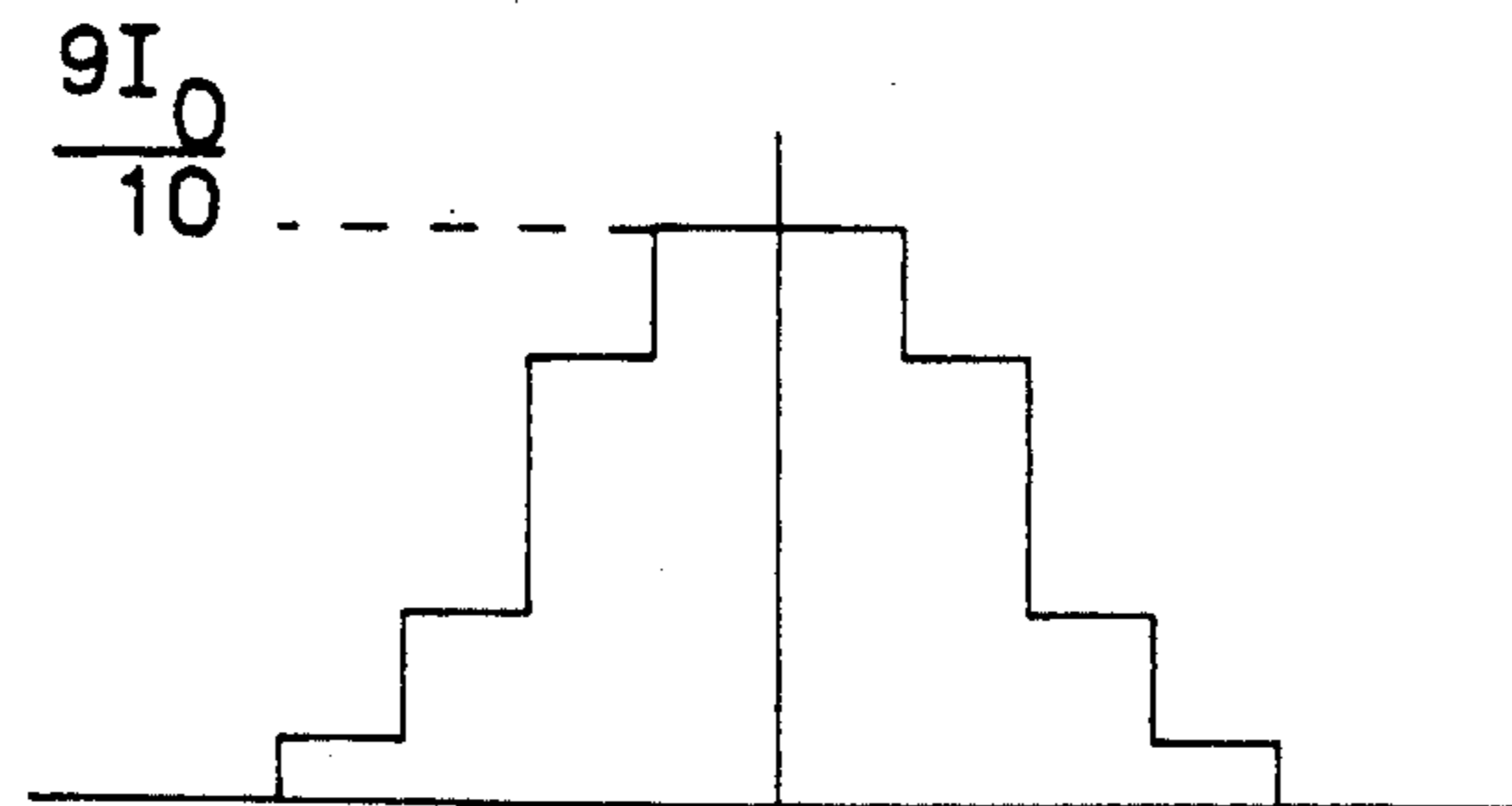
DIFFRACTED PIXEL LUMINANCE PROFILE
