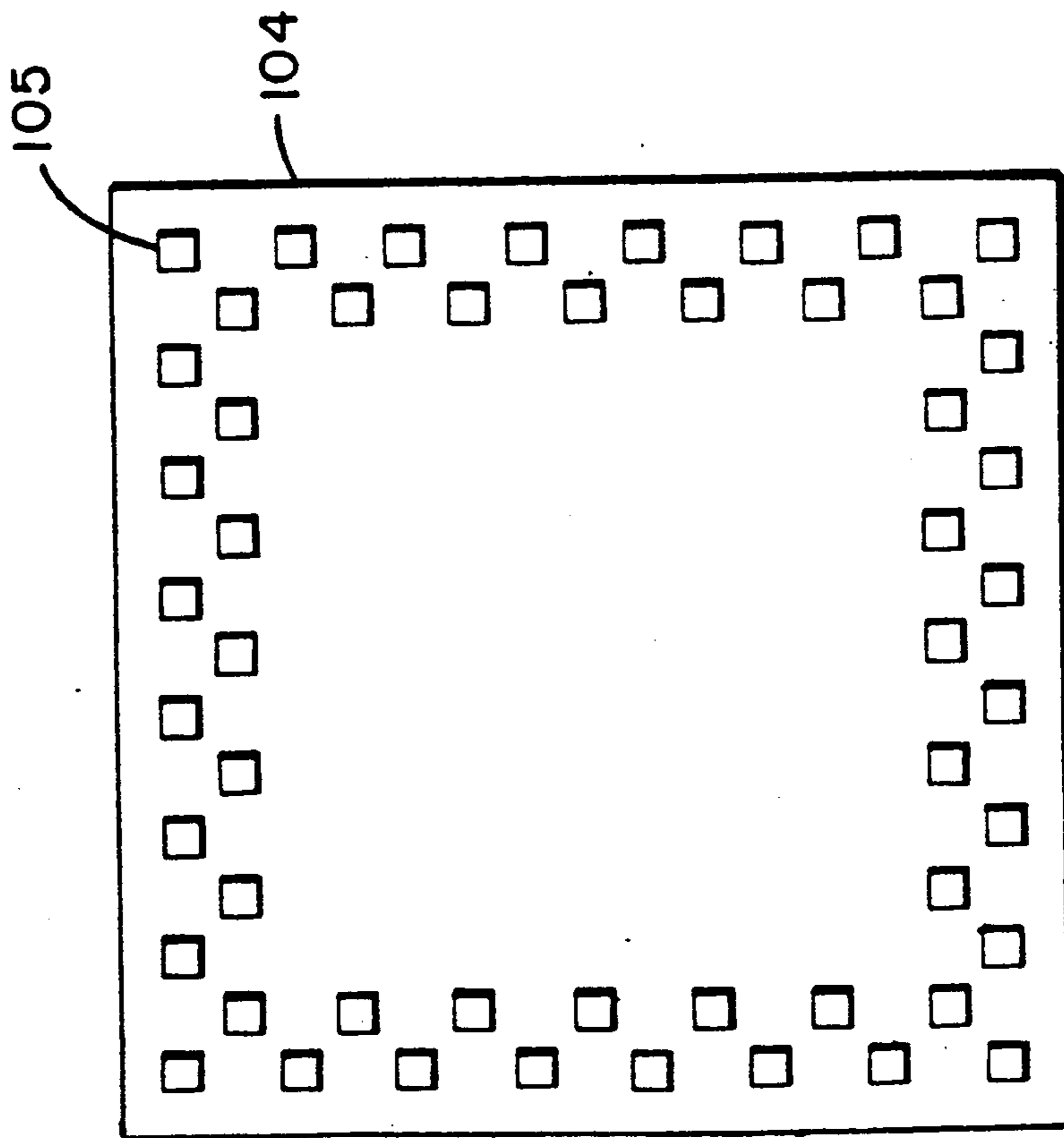
Bonding Pad Pattern On Chip
