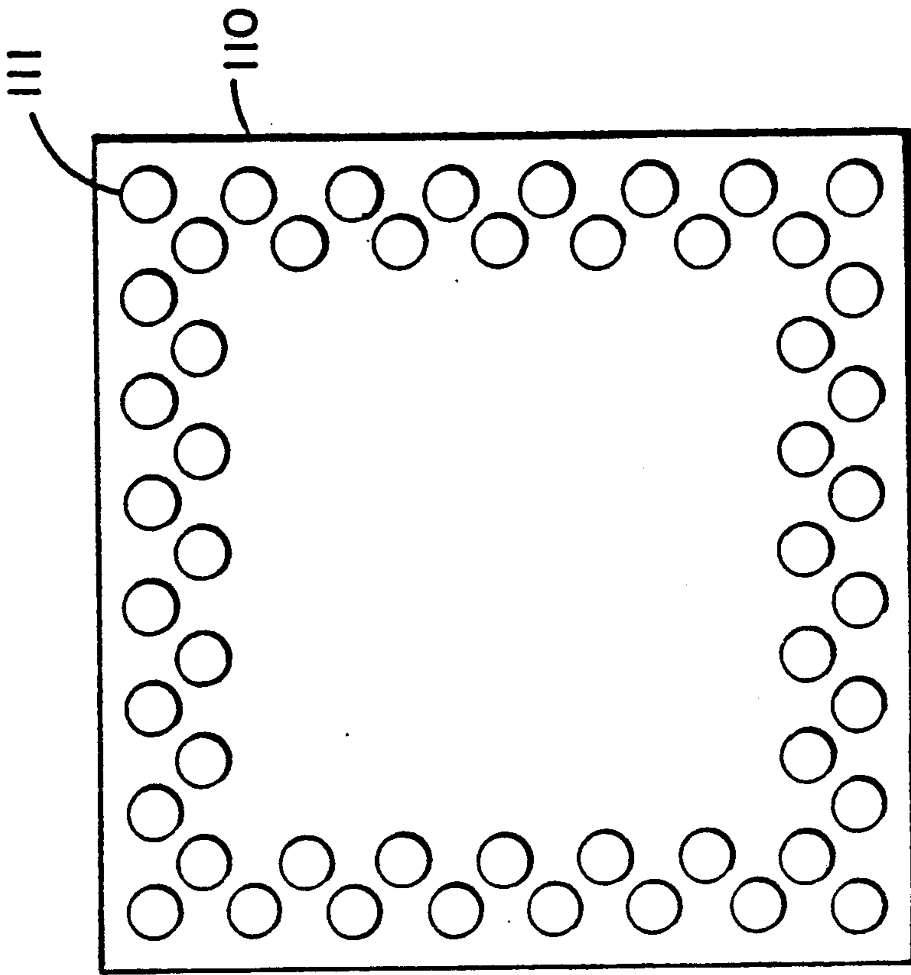
Plated Hole Pattern On Circuit Board
