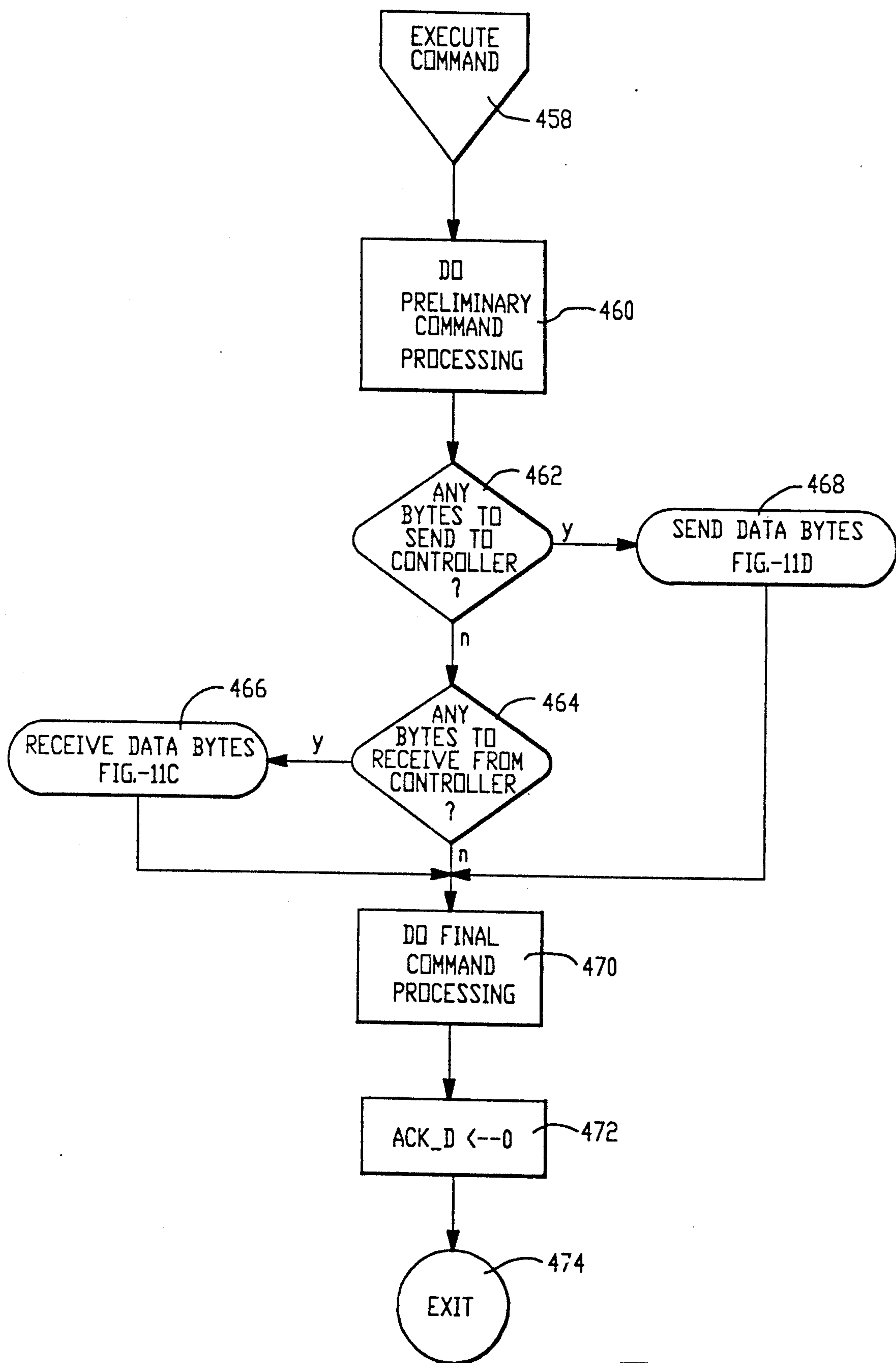
FIG.-11B EXECUTE COMMAND 448
