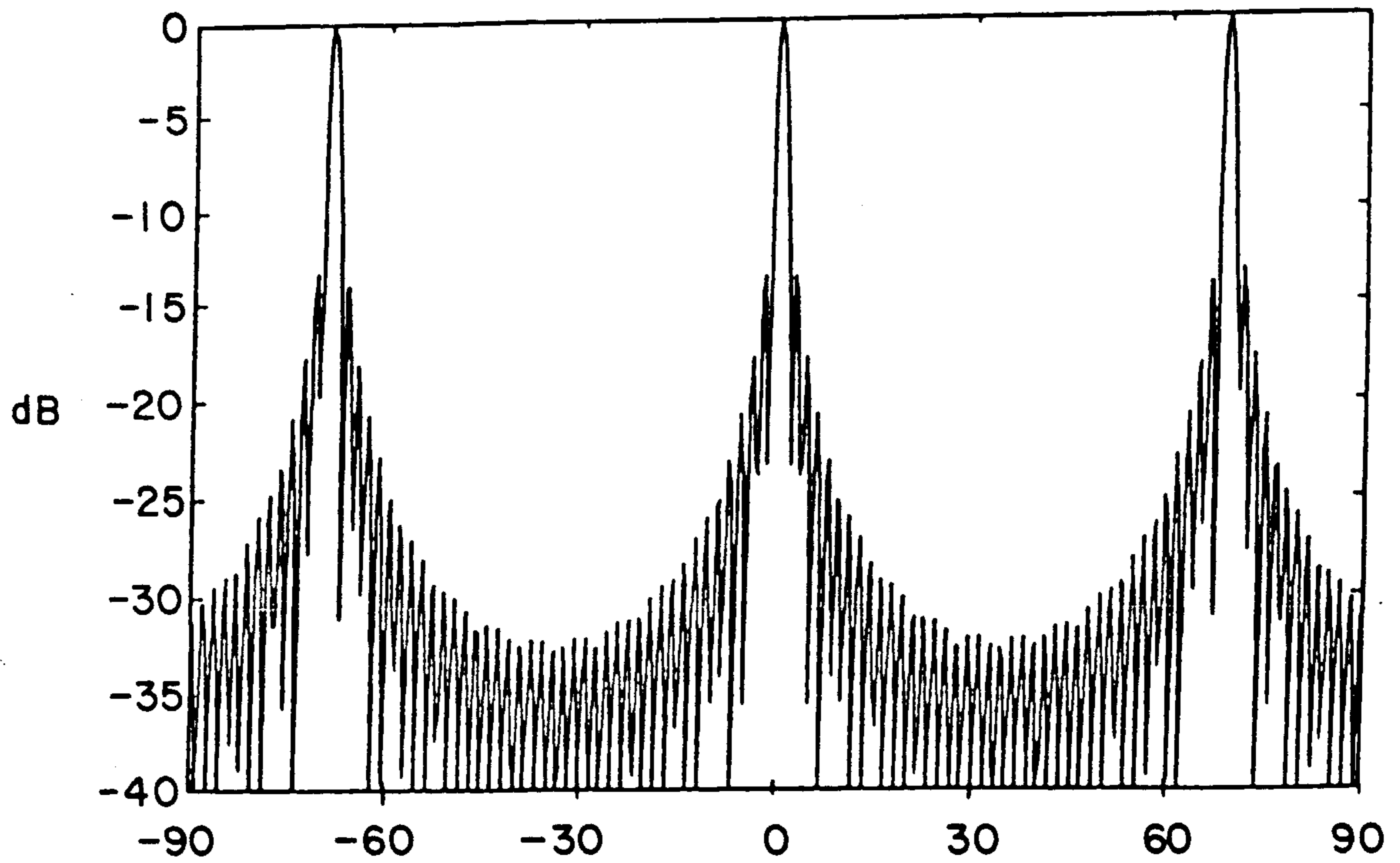
Angle theta in degrees Pattern of a thinned array antenna with uniform spacing containing grating lobes
