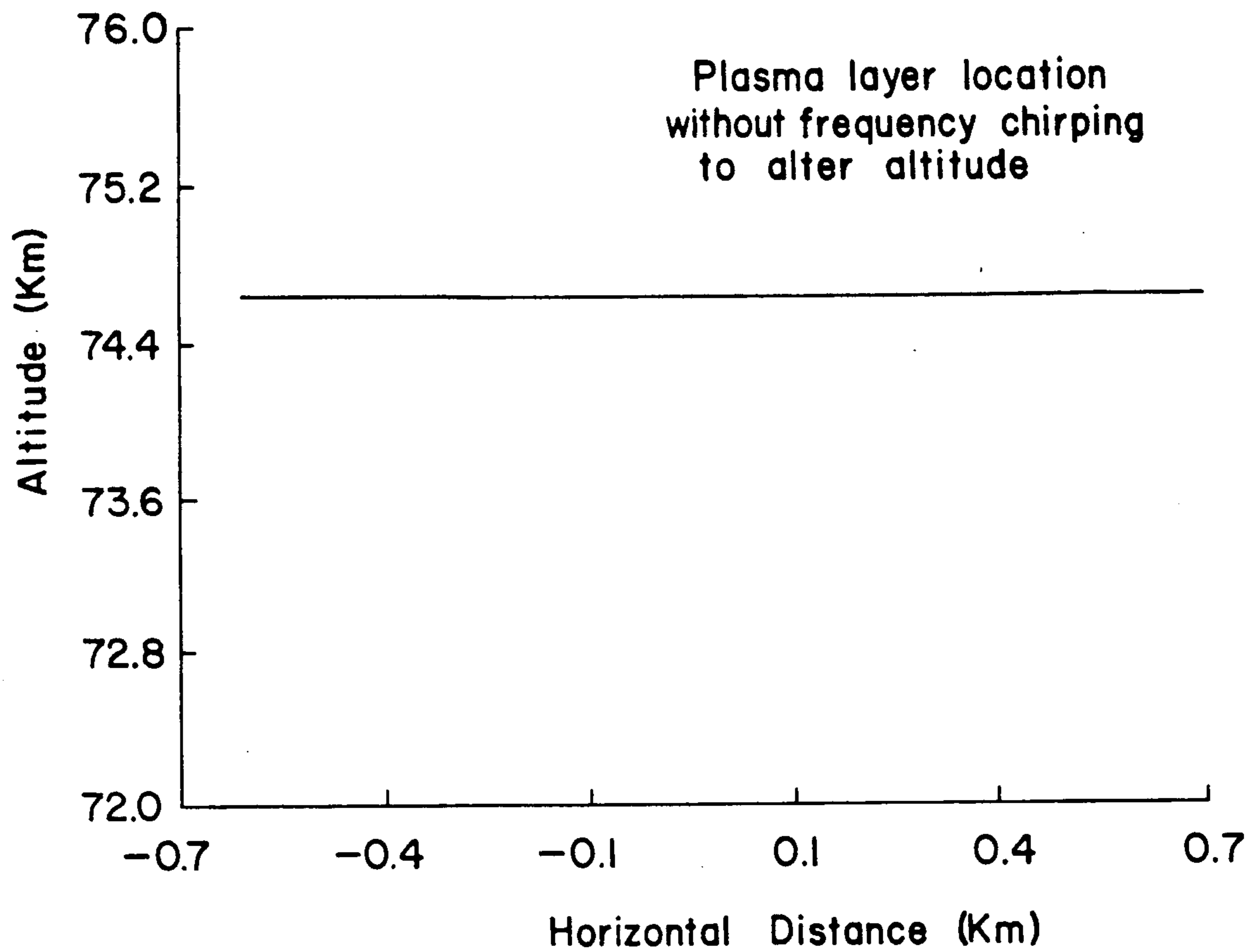
Heater focusing at 75Km with 550 MHz frequency and 154 dBW
