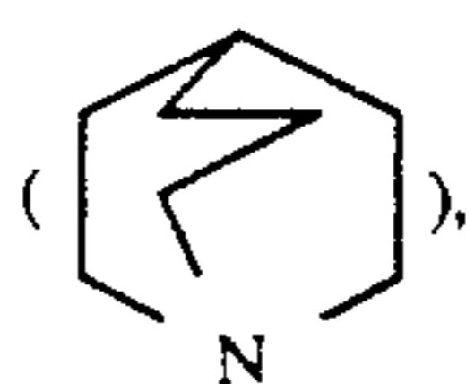
1-azabicyclo[3,1,1]heptane ring
