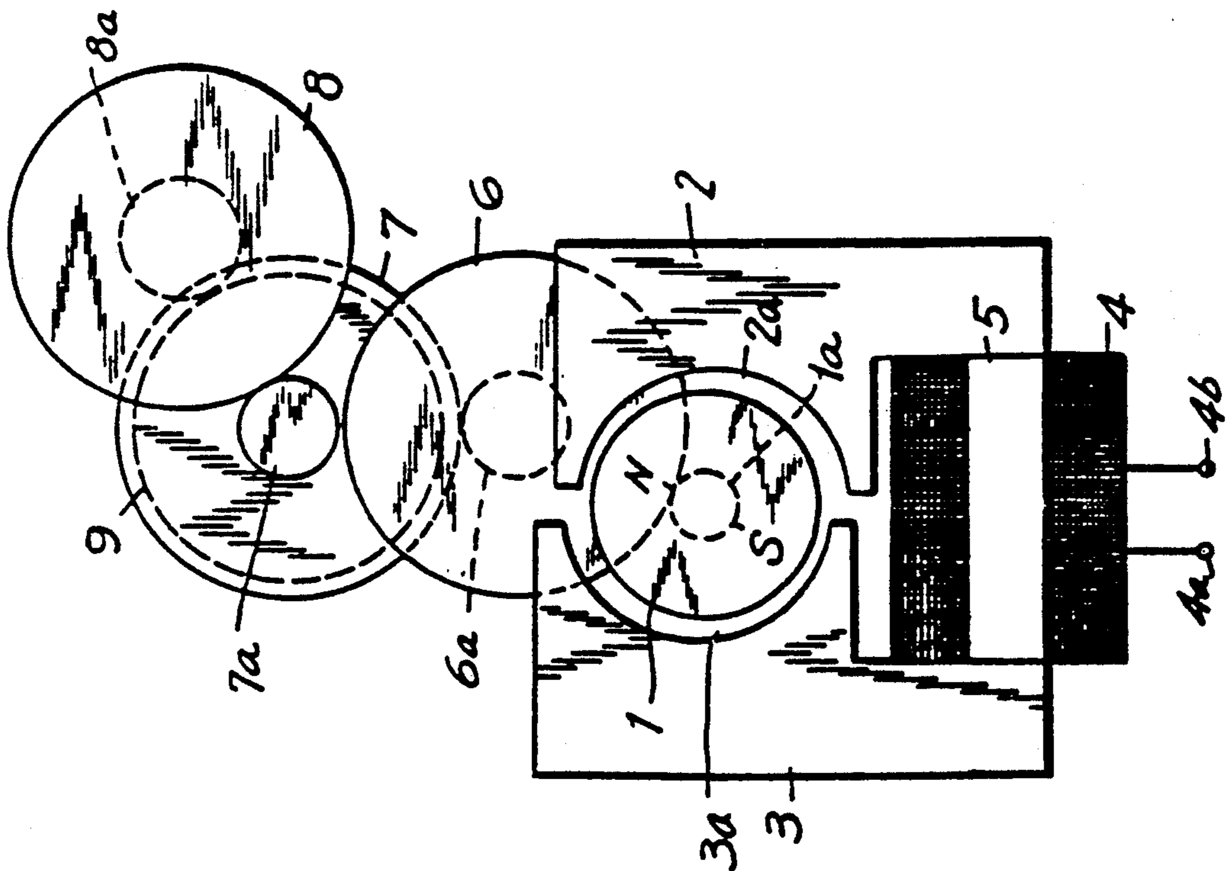
FIG. 1 PRIOR ART
