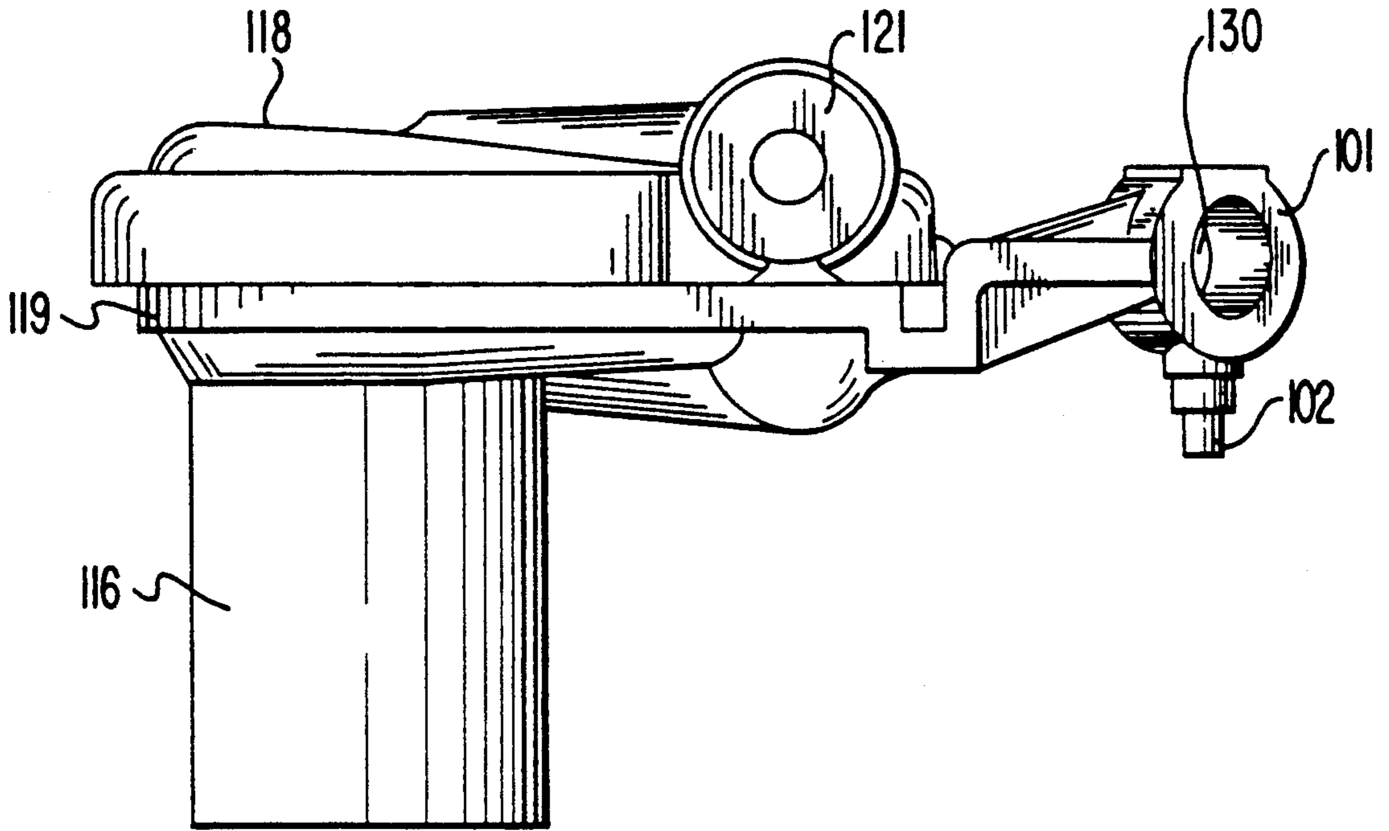
FIG. 9 (PRIOR ART)
