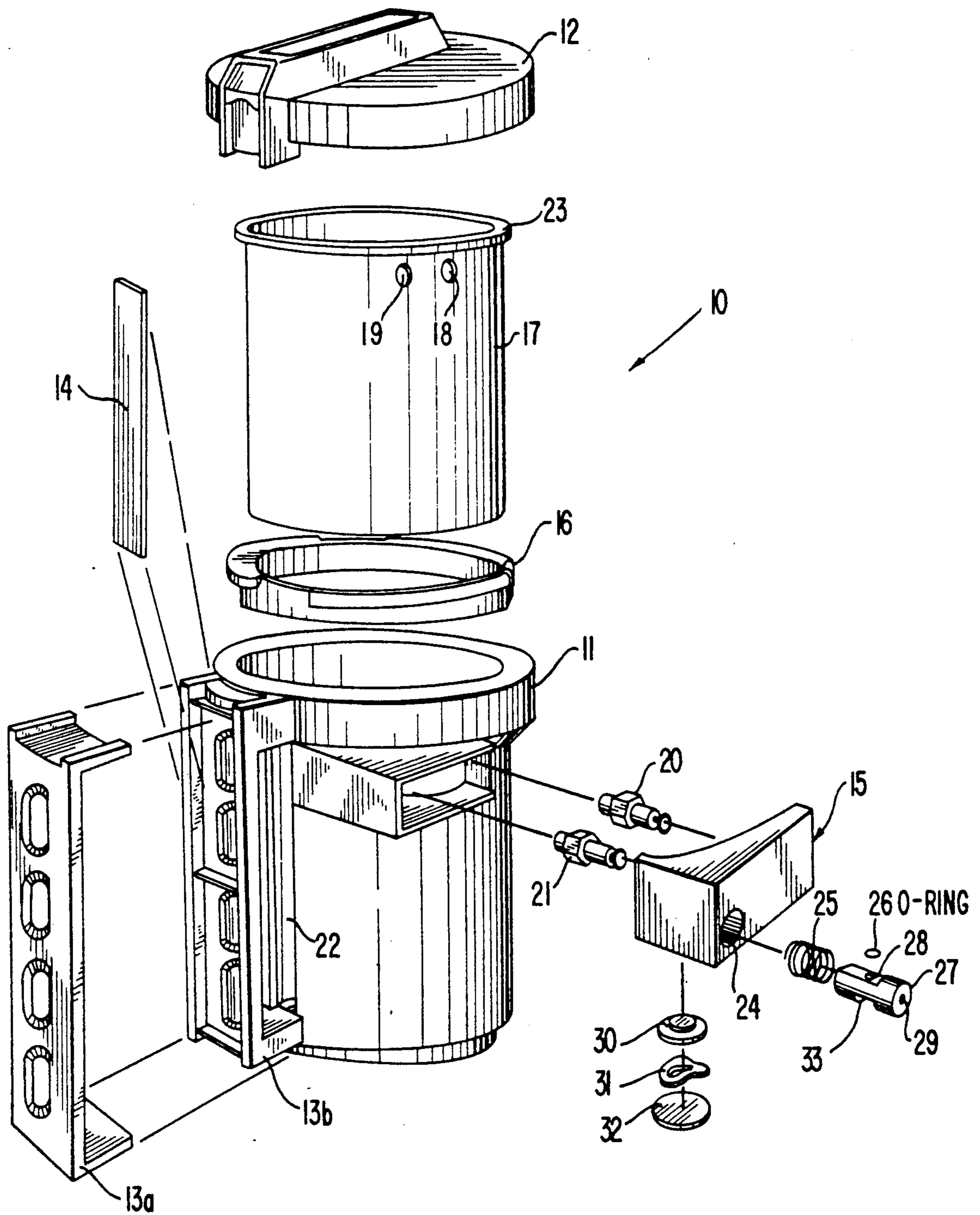
FIG. 1 (PRIOR ART)
