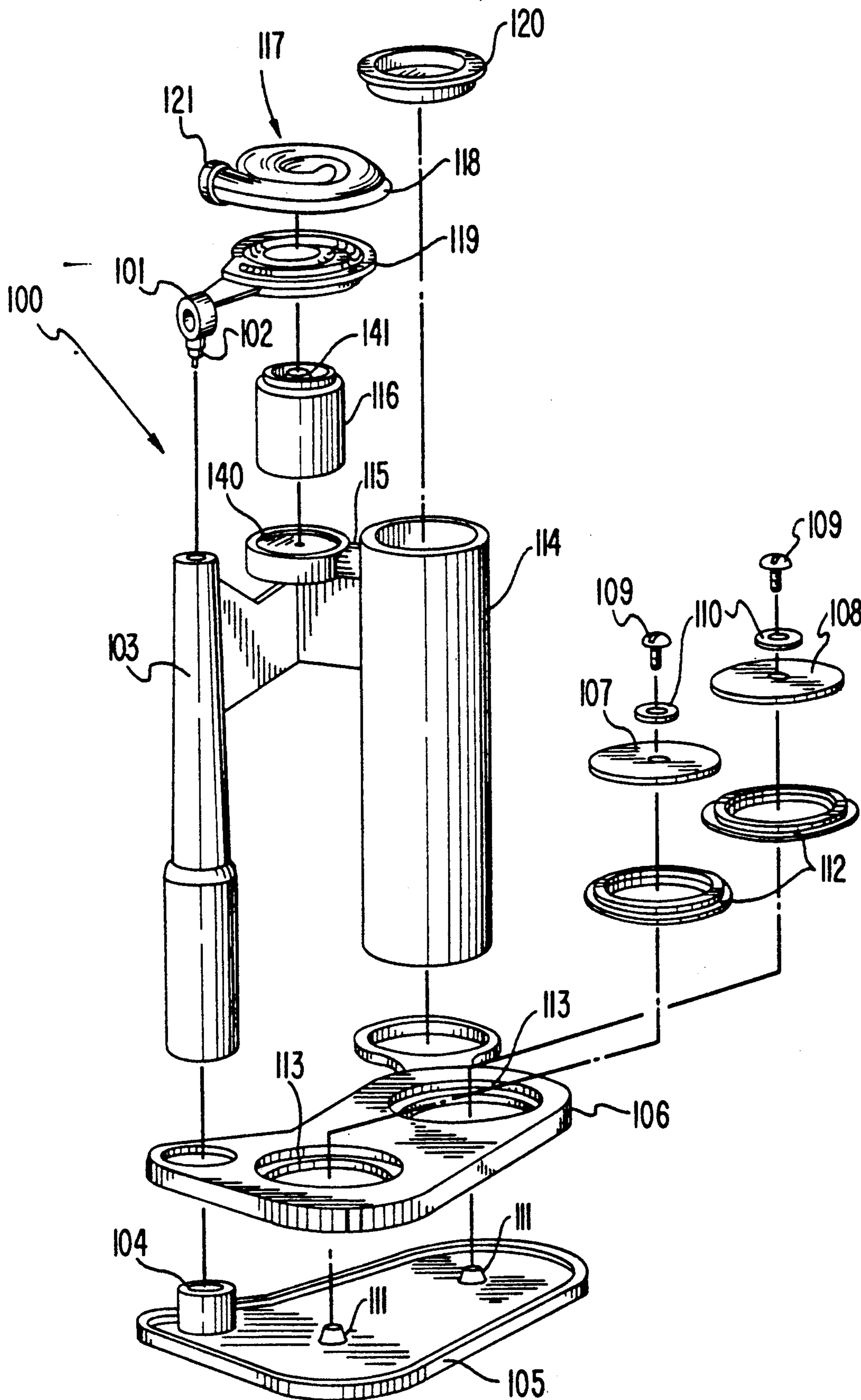
FIG. 2 (PRIOR ART)
