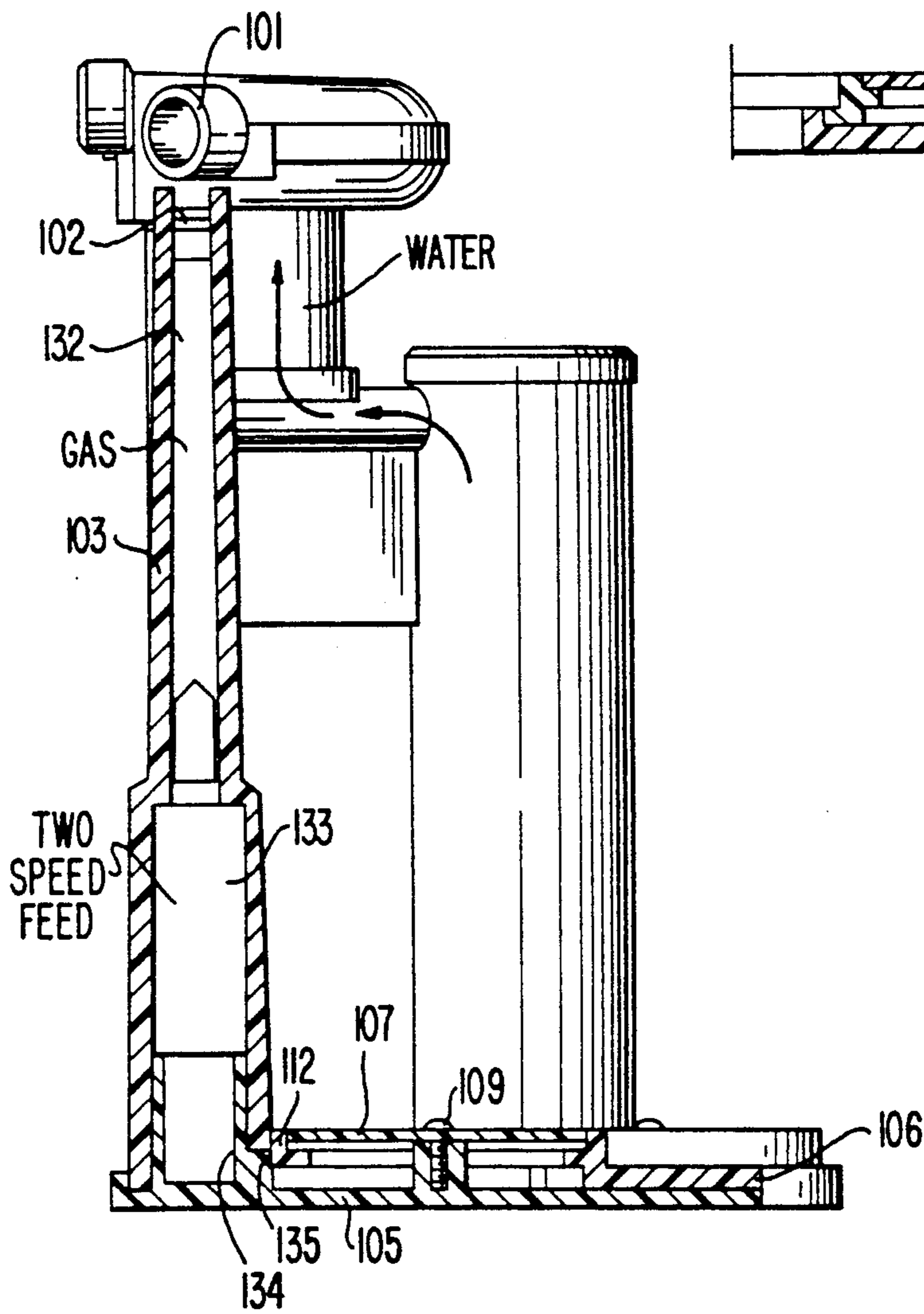
FIG. 11 (PRIOR ART)
