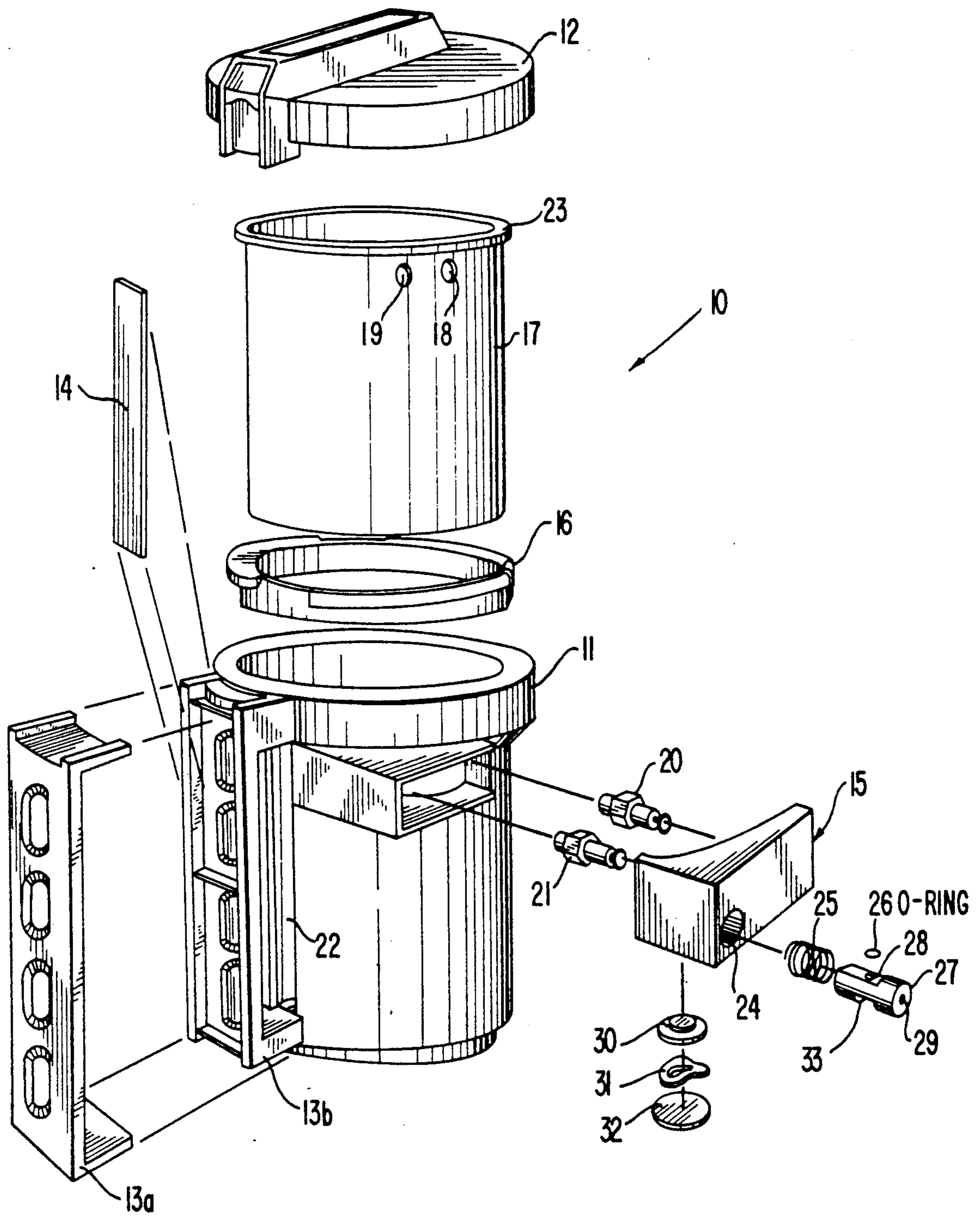
FIG. 1 (PRIOR ART)
