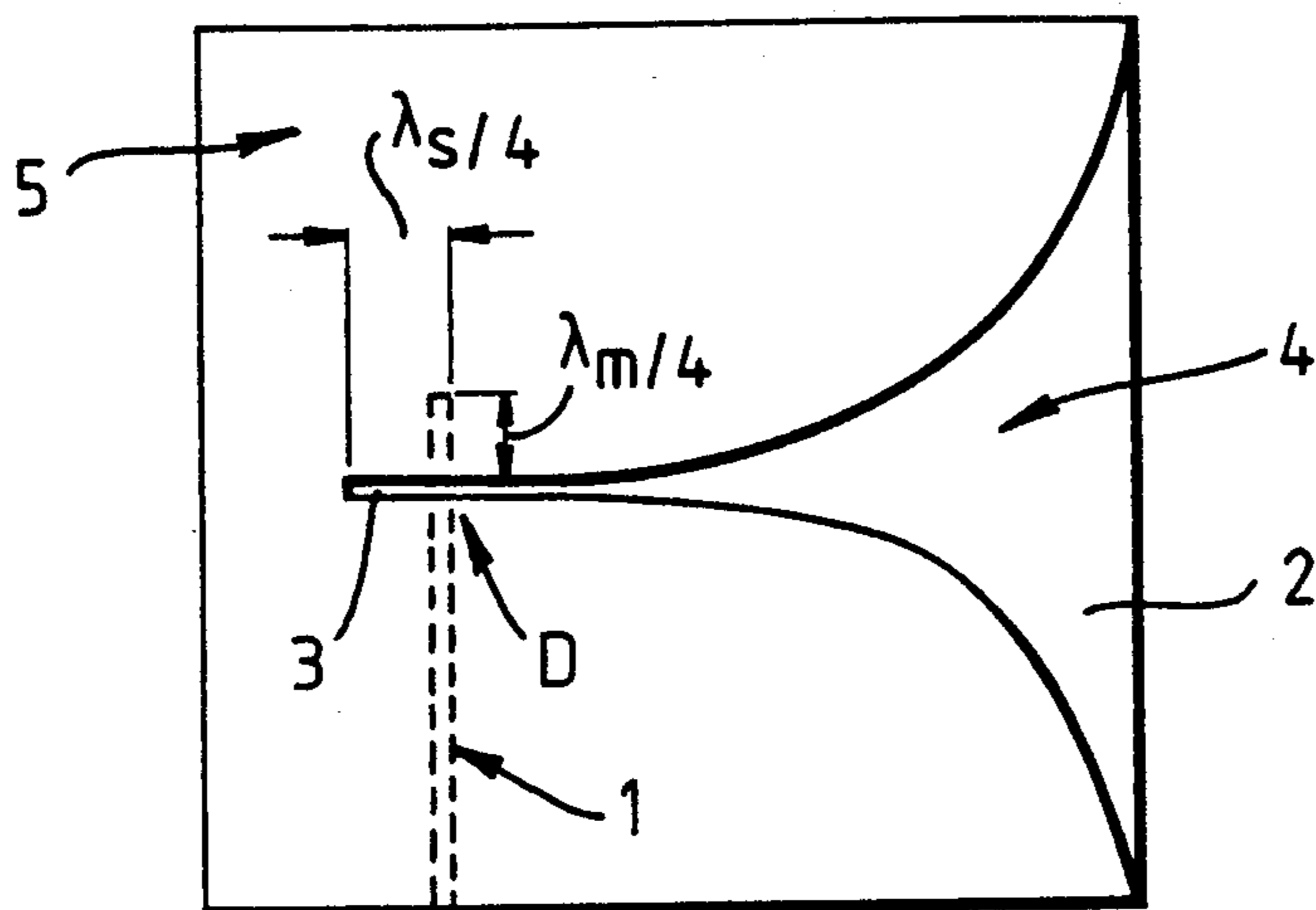
Fig. 1. PRIOR ART
