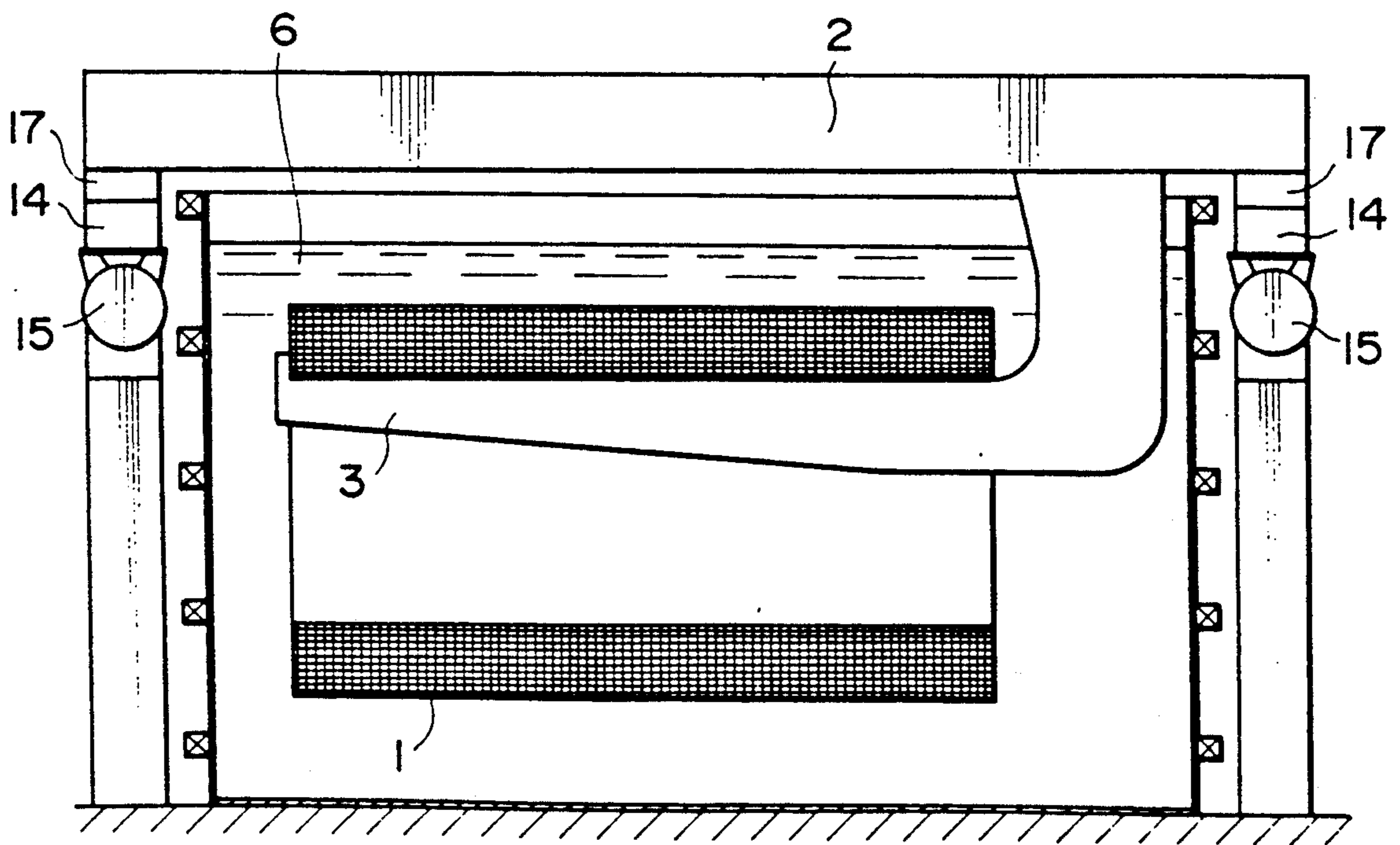
FIG. 12 (PRIOR ART)
