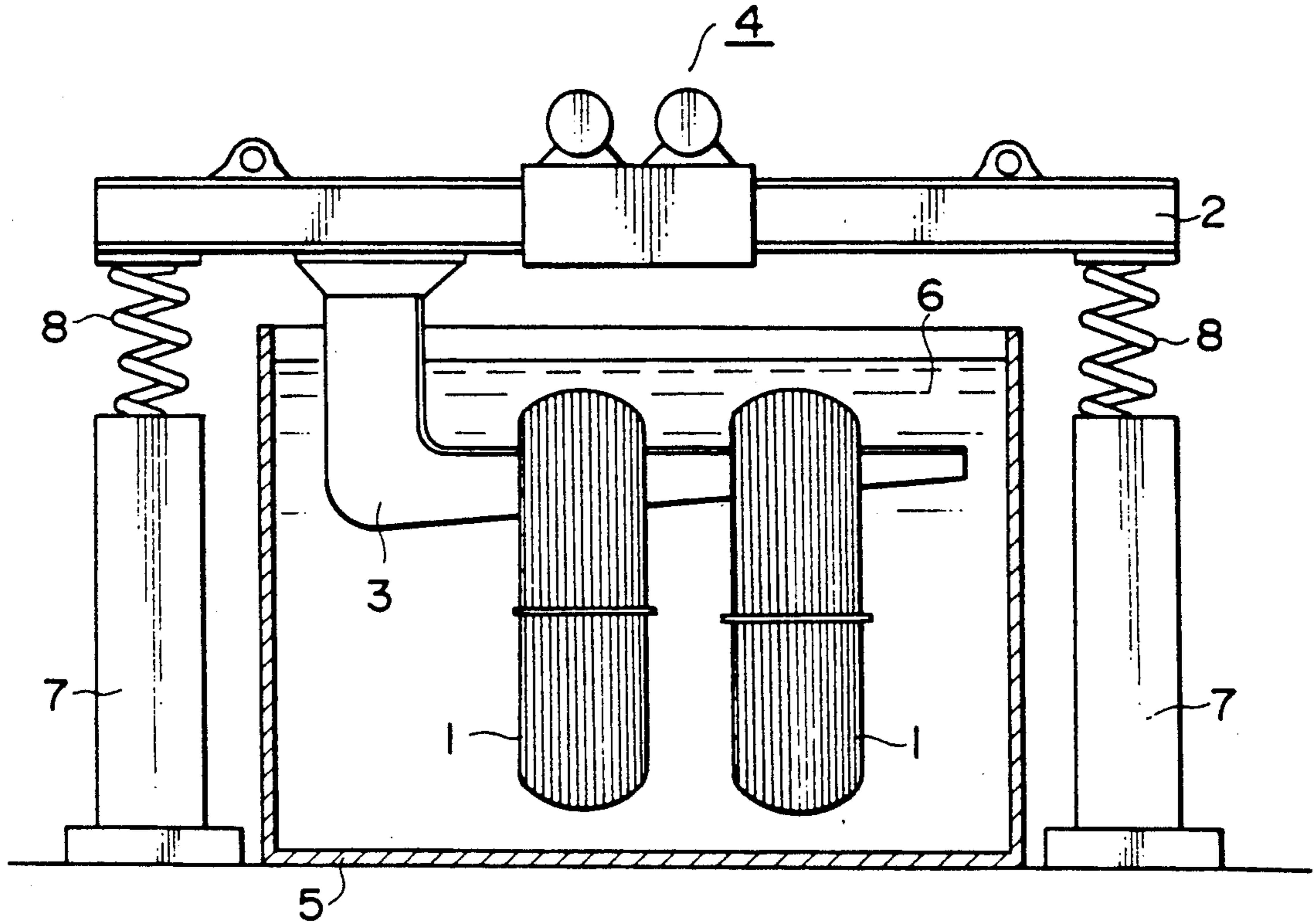
FIG. 11 (PRIOR ART)
