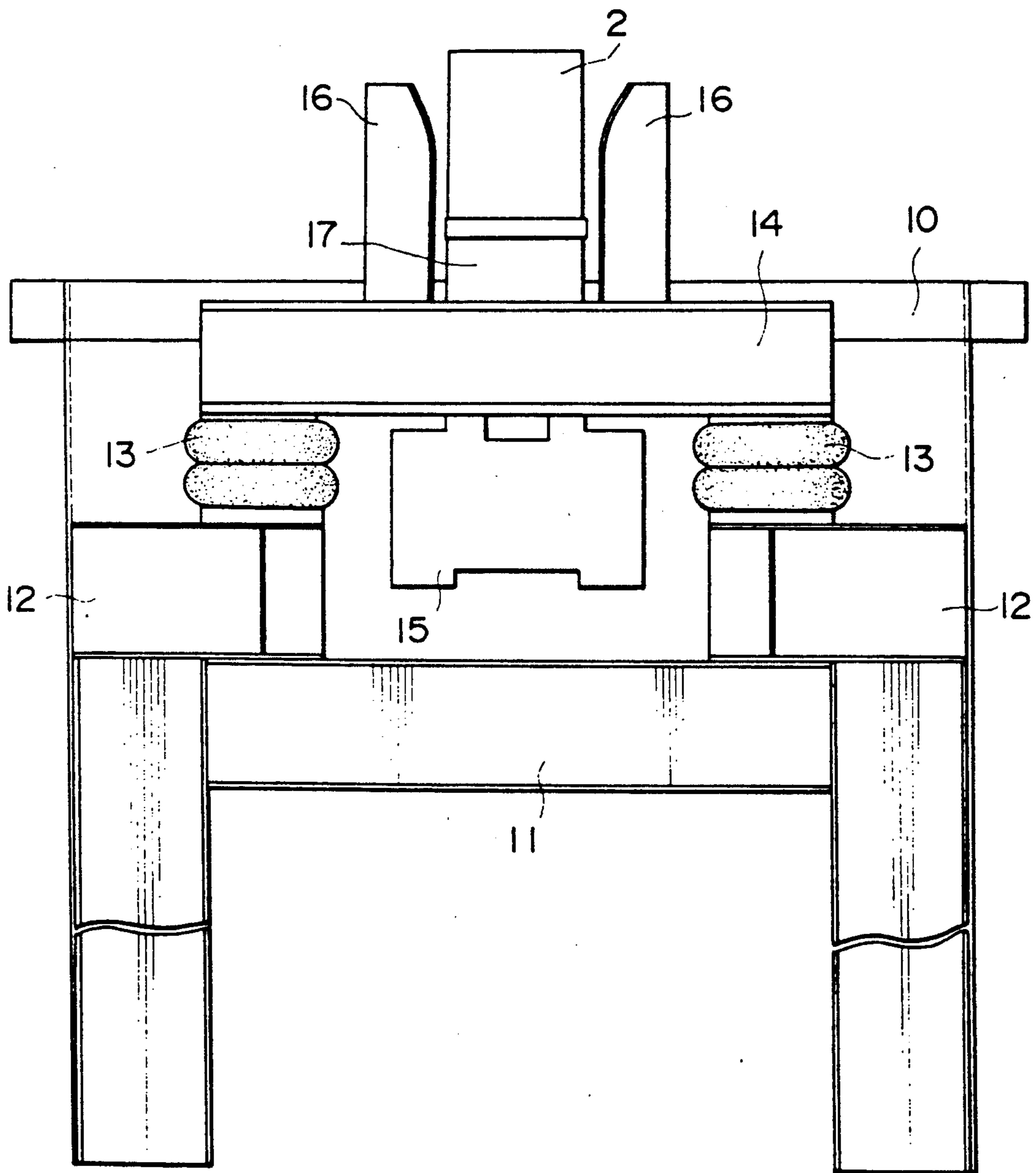
FIG. 13 (PRIOR ART)
