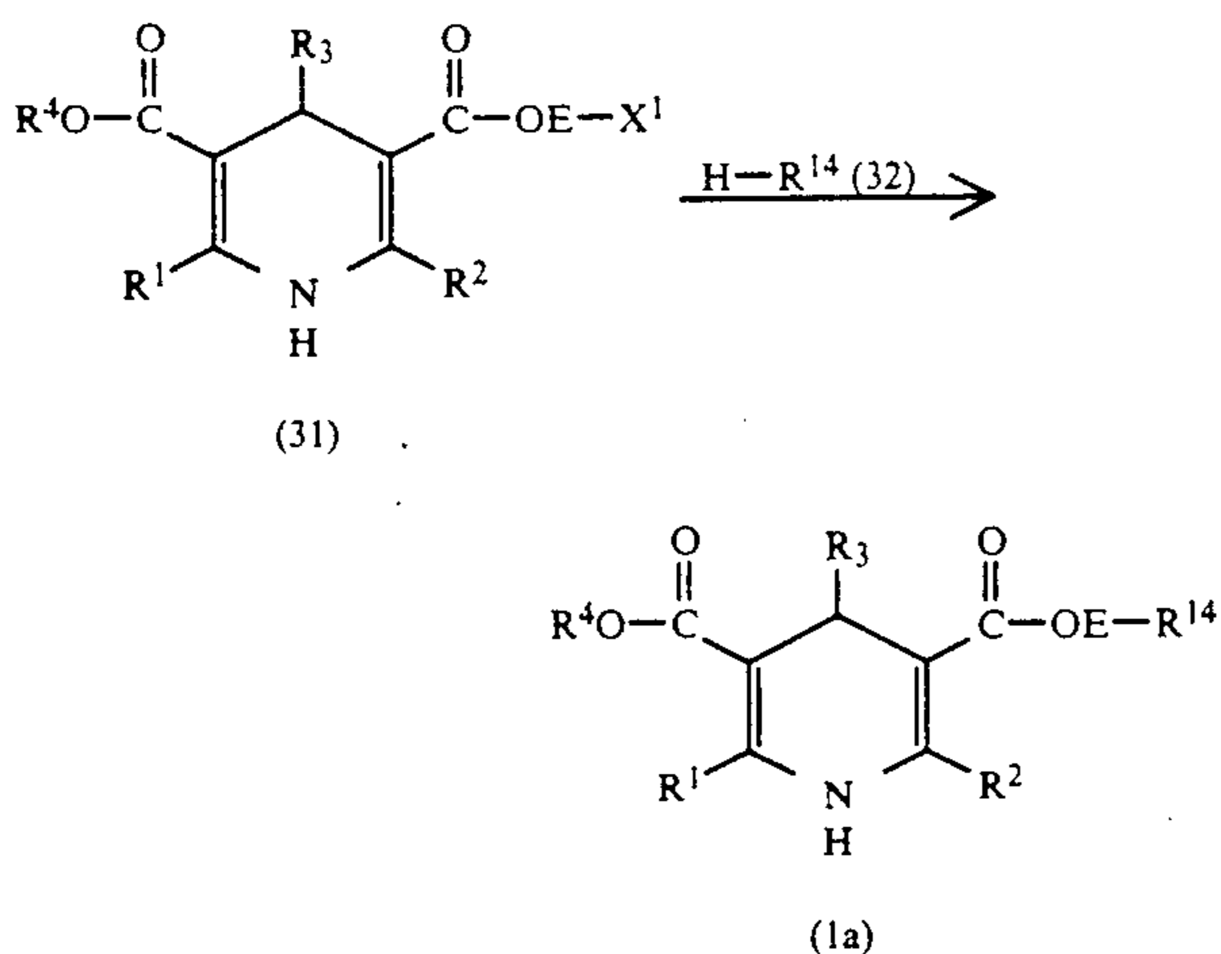
Reaction process formula-16
