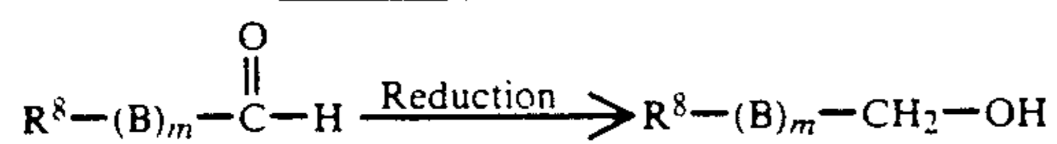
Reaction process formula-11
