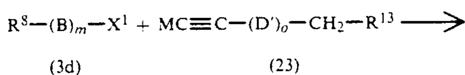
Reaction process formula-10
