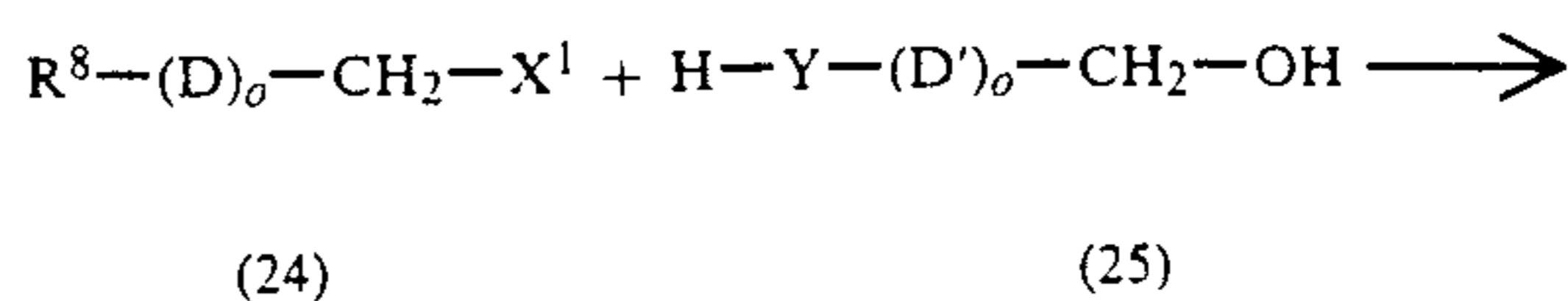
Reaction process formula-12
