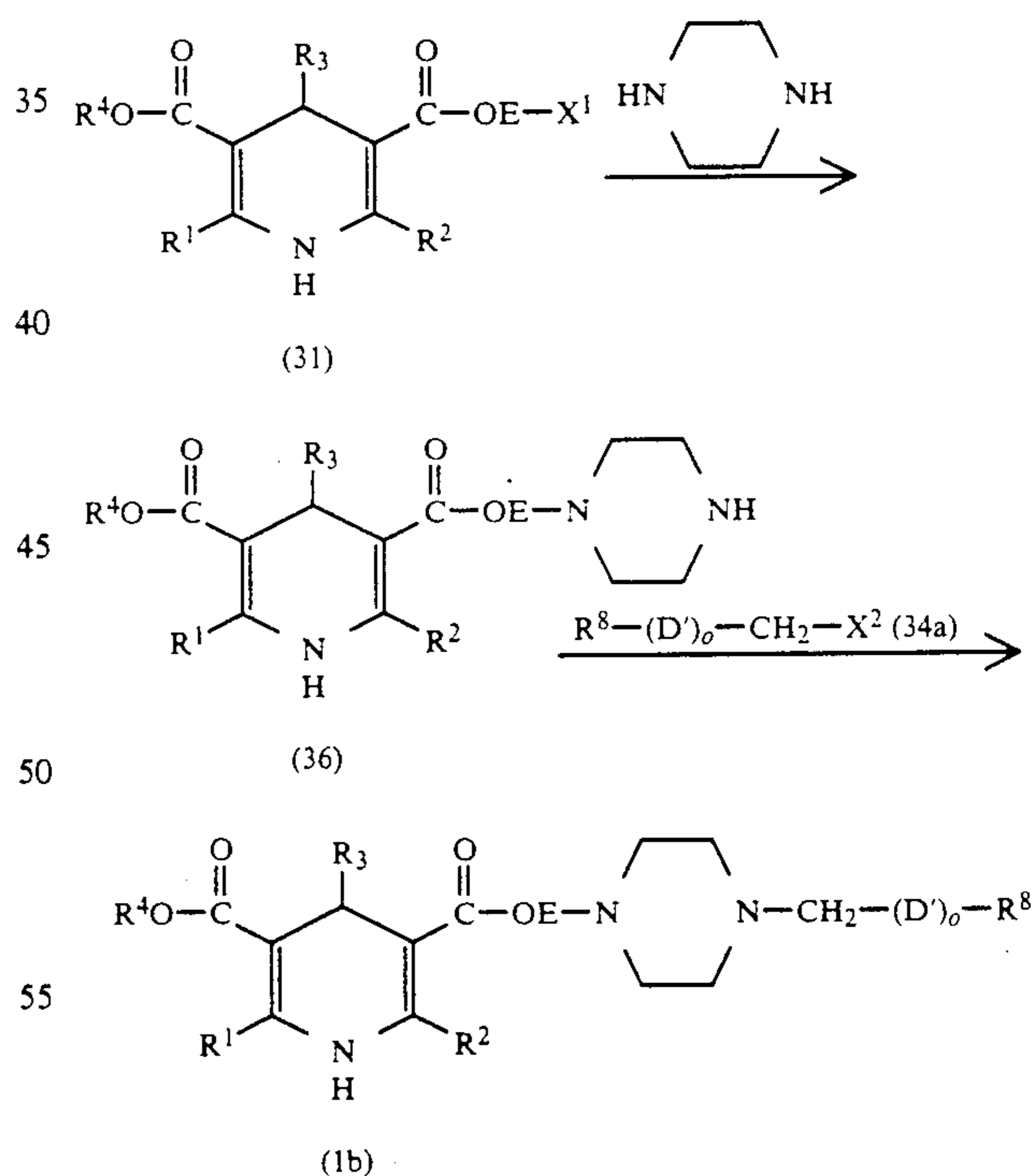
Reaction process formula-18
