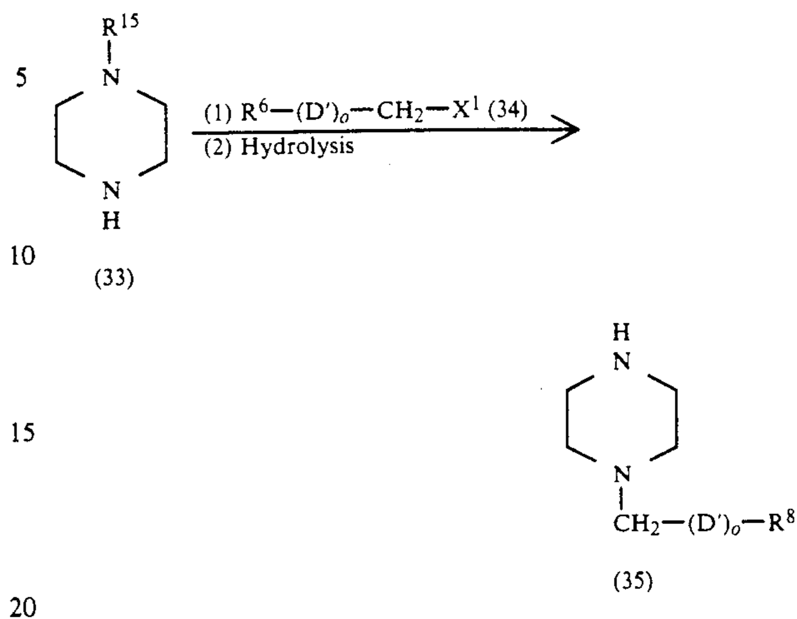
Reaction process formula-17
