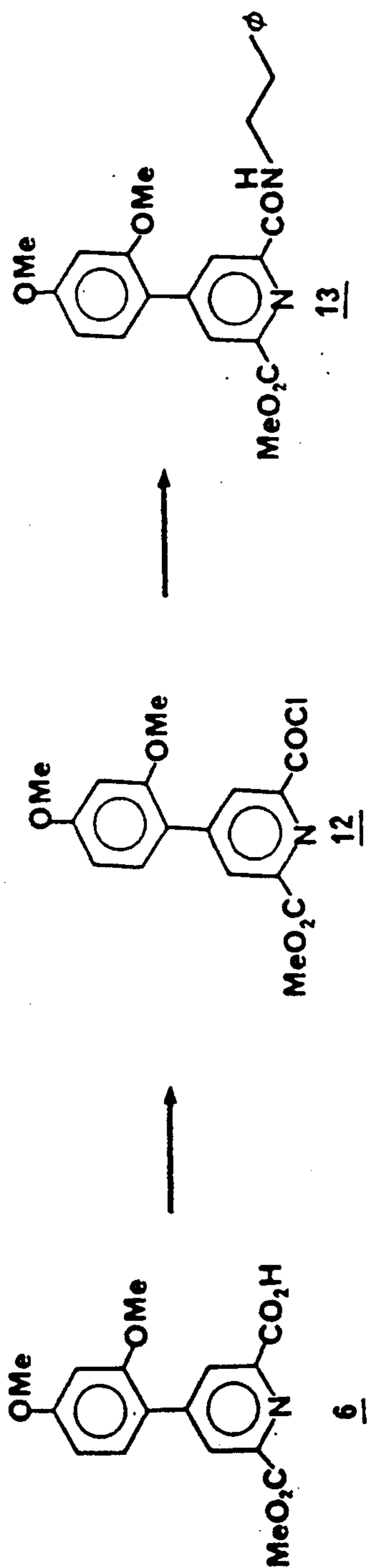
SCHEME III
