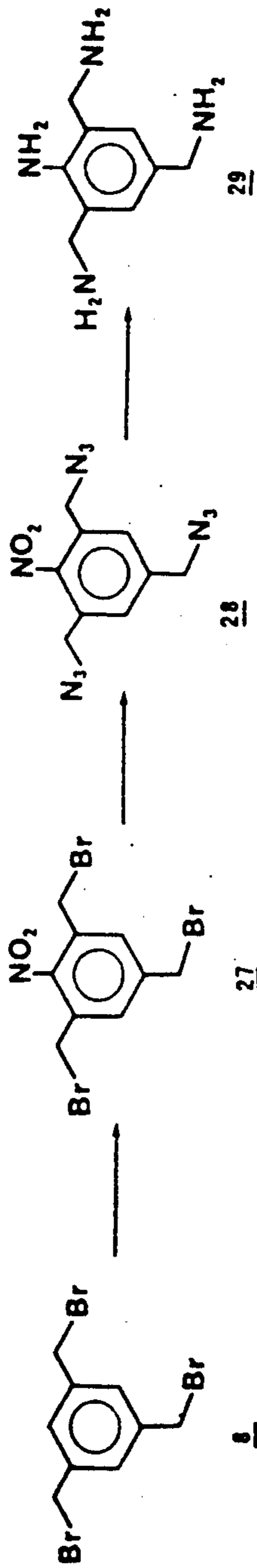
SCHEME VII
