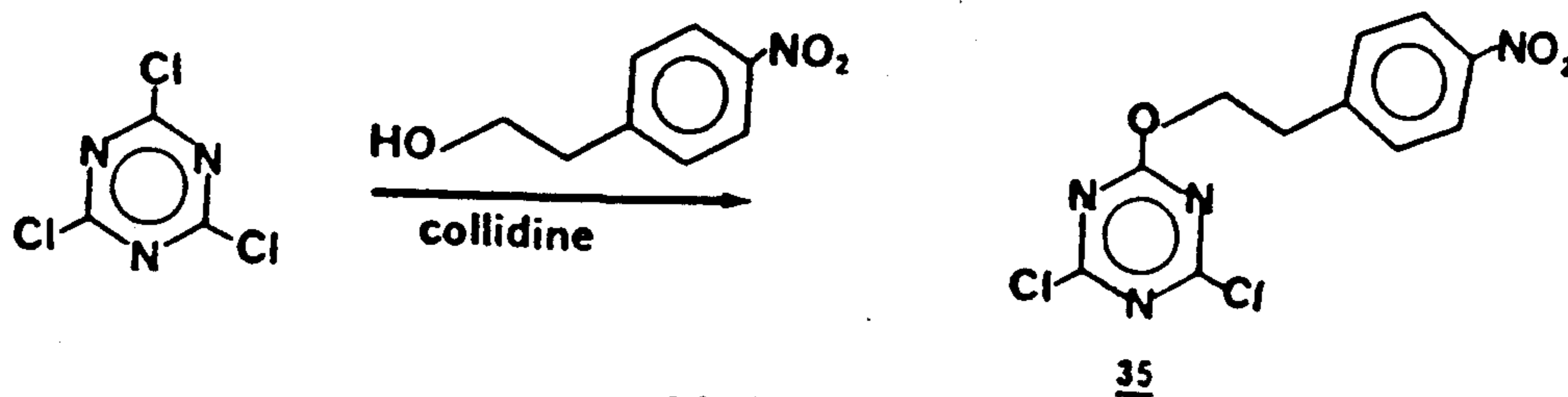
SCHEME IX
