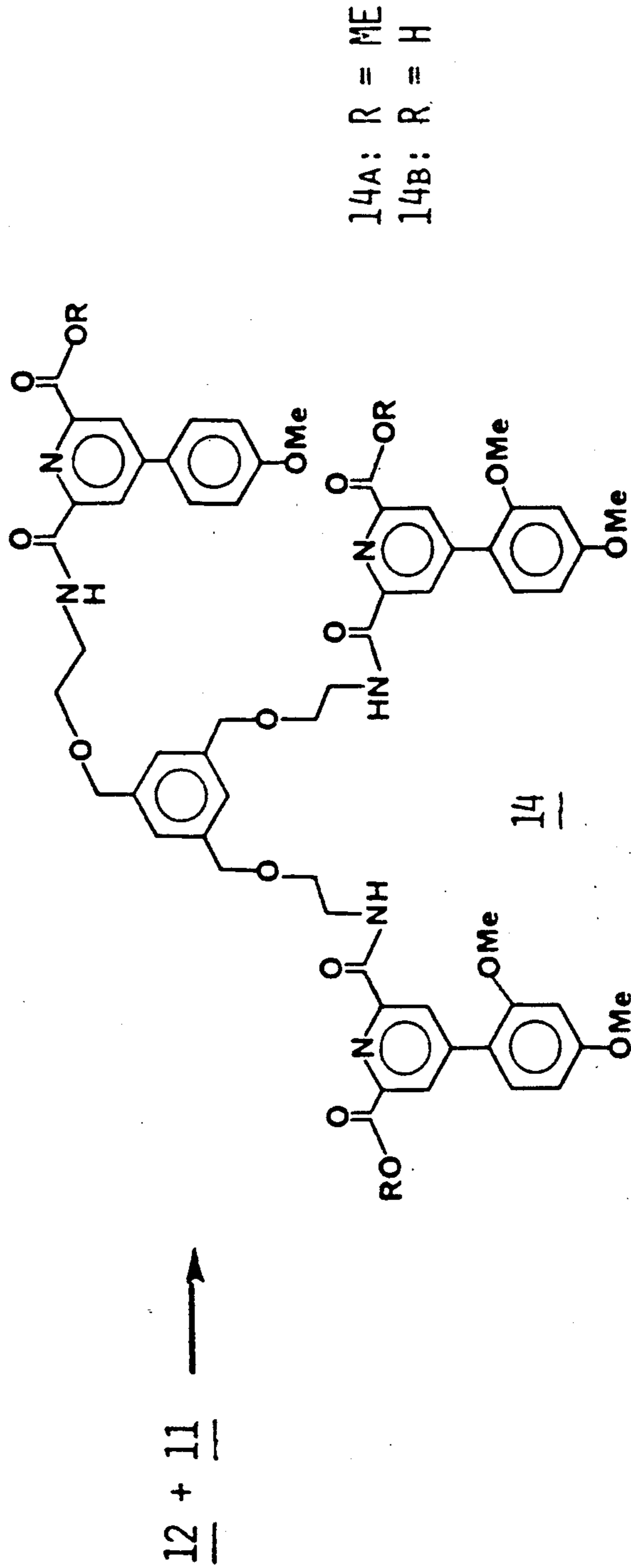
SCHEME IV
