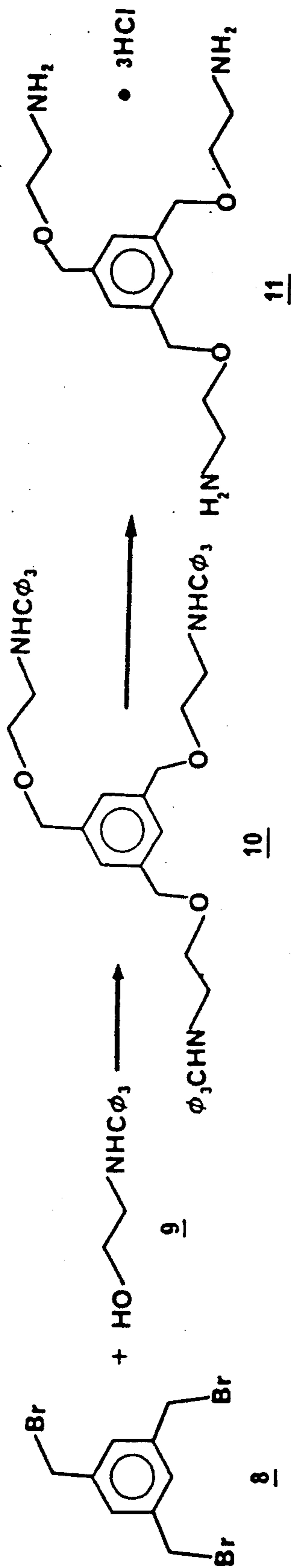
SCHEME II
