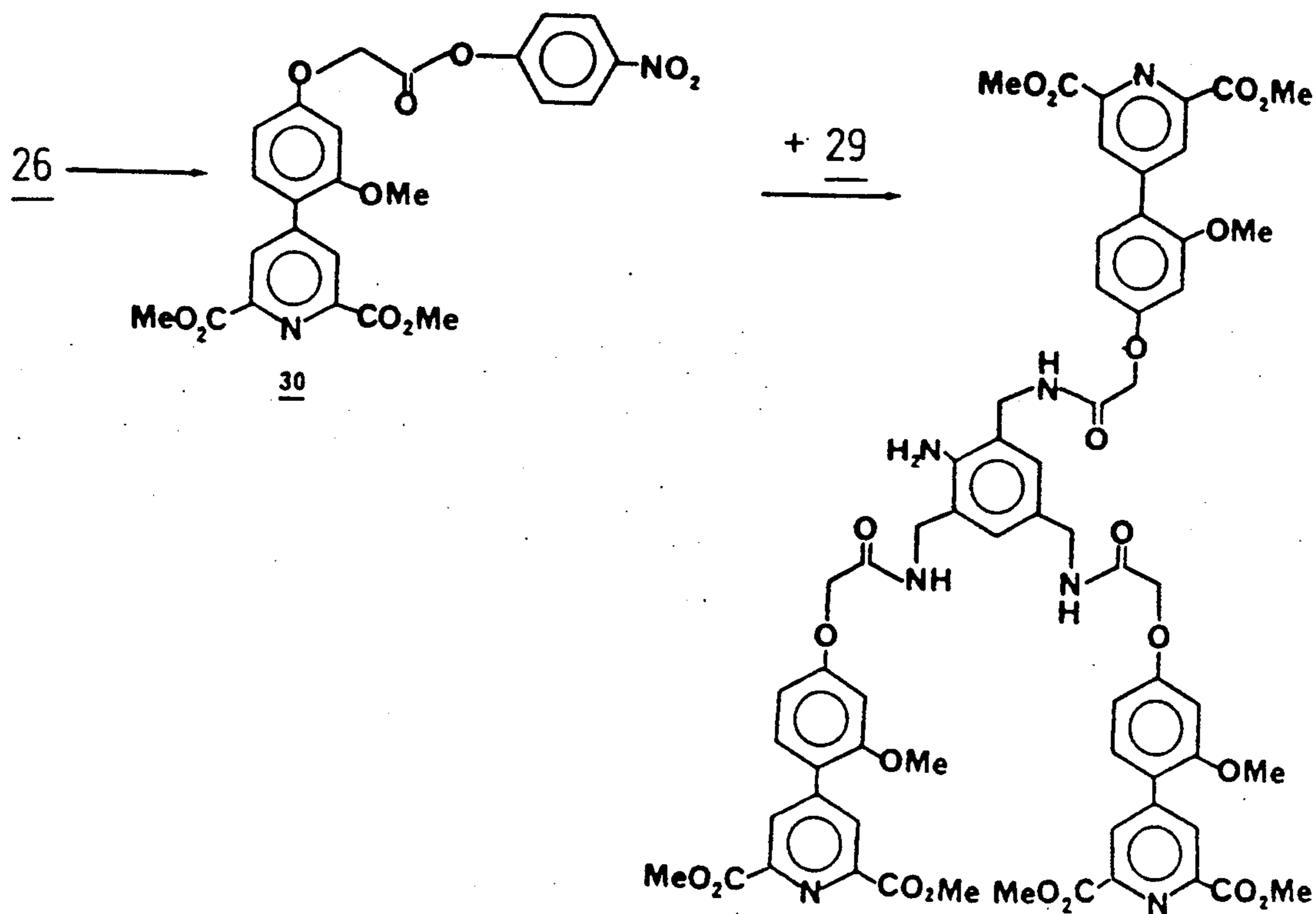
SCHEME VIII
