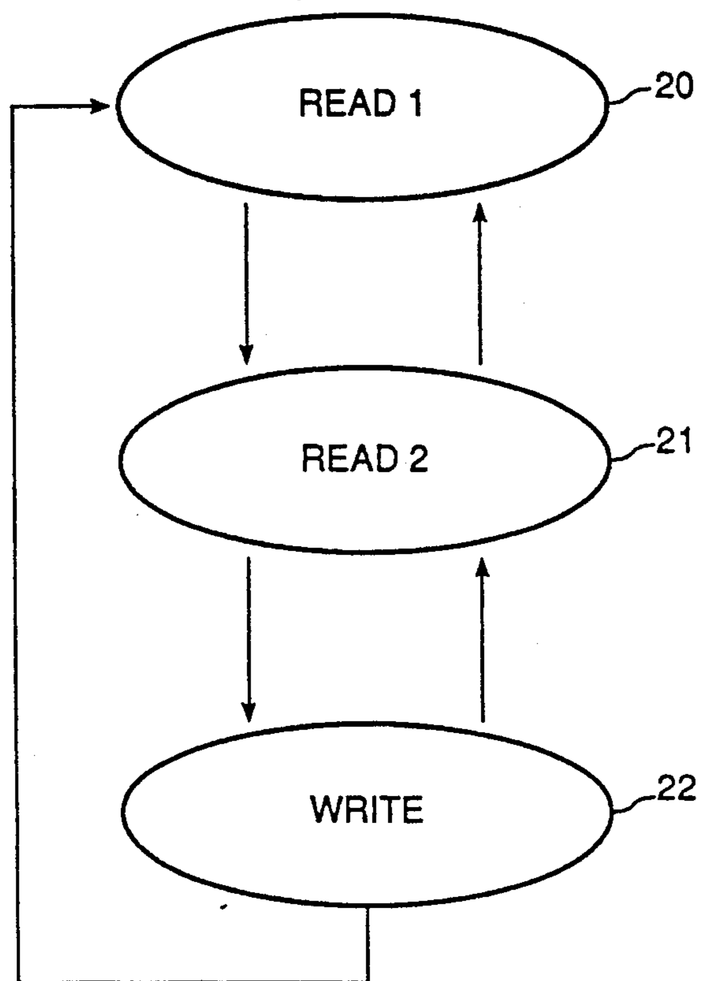
STATE DIAGRAM
