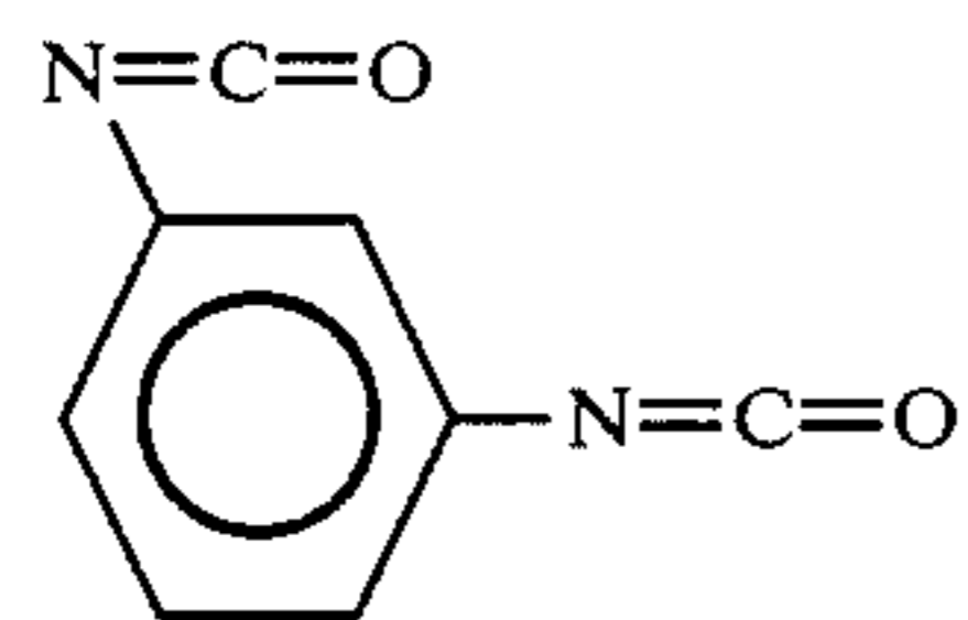
1,3-phenylene diisocyanate
