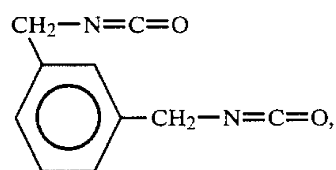
m-xylylene diisocyanate
