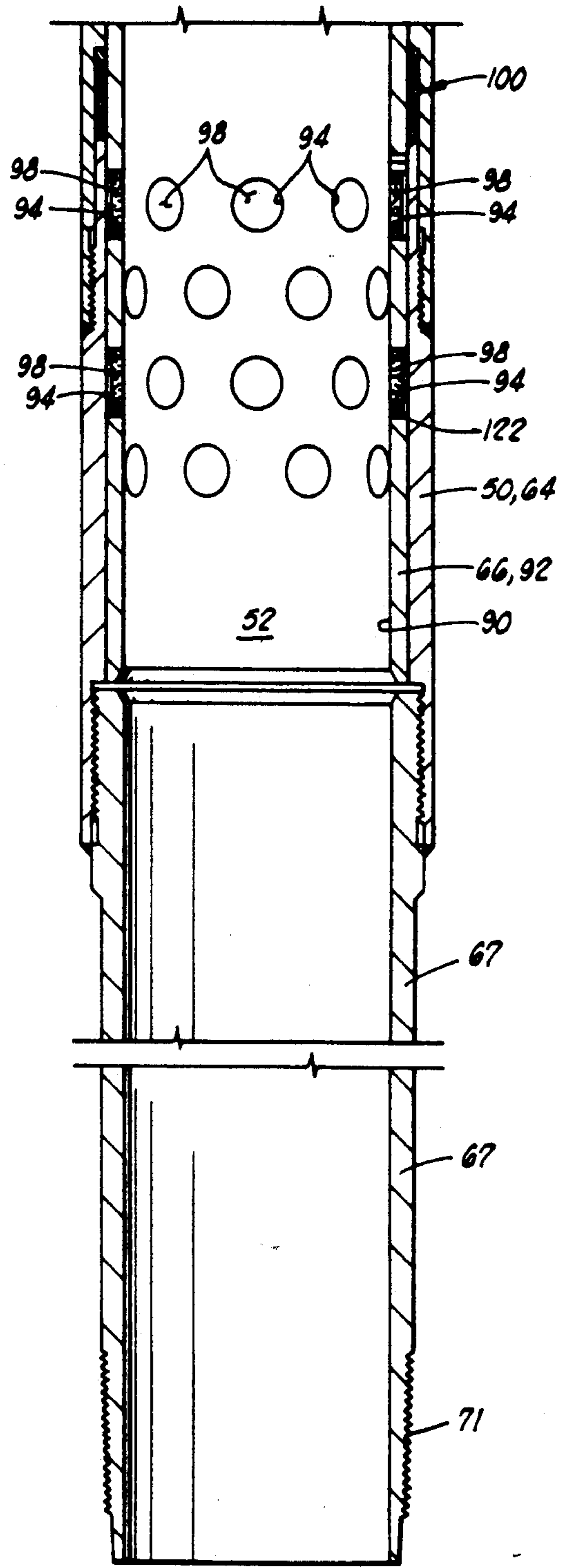
FIG. 2D
