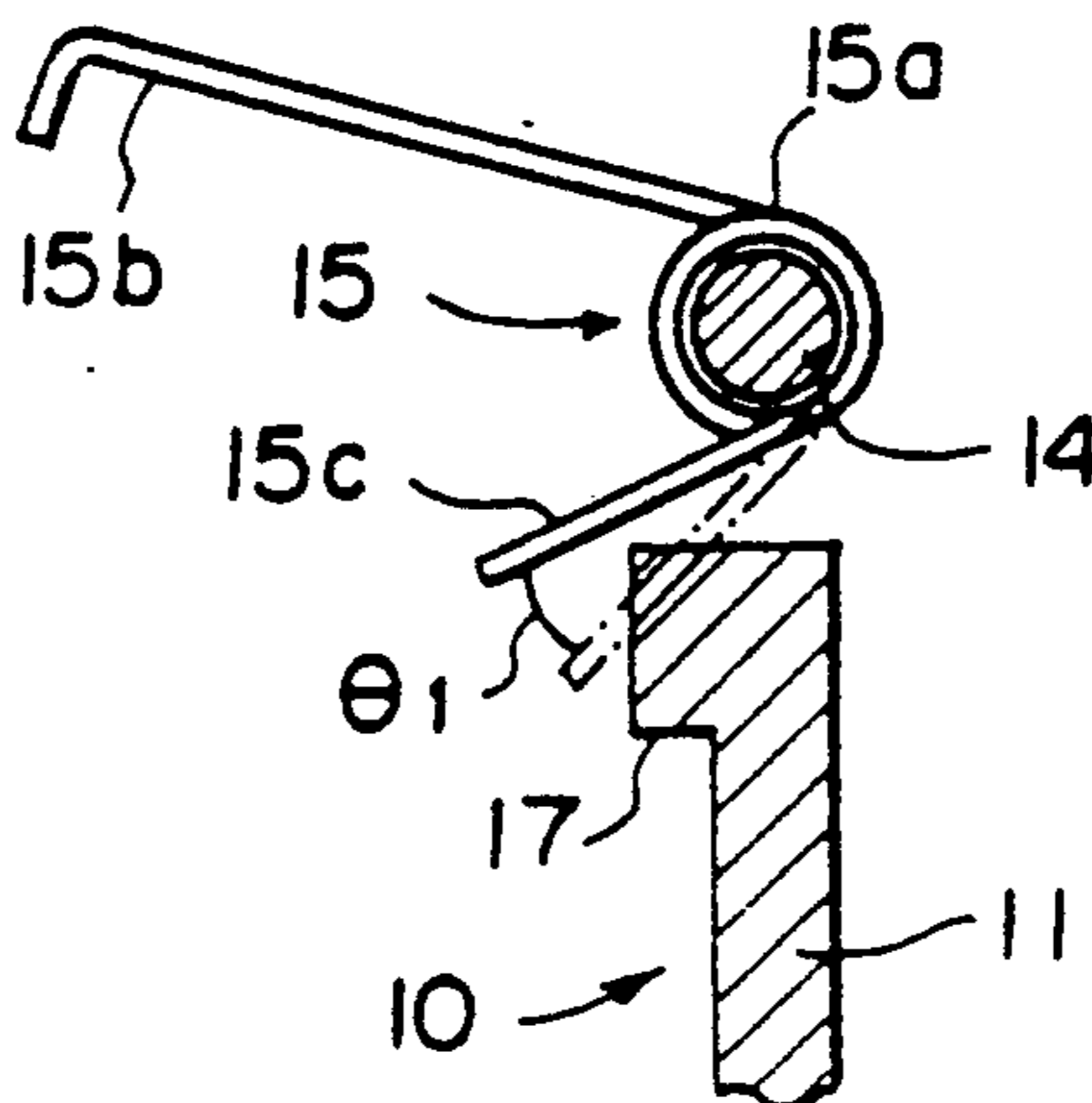
FIG. 14 PRIOR ART
