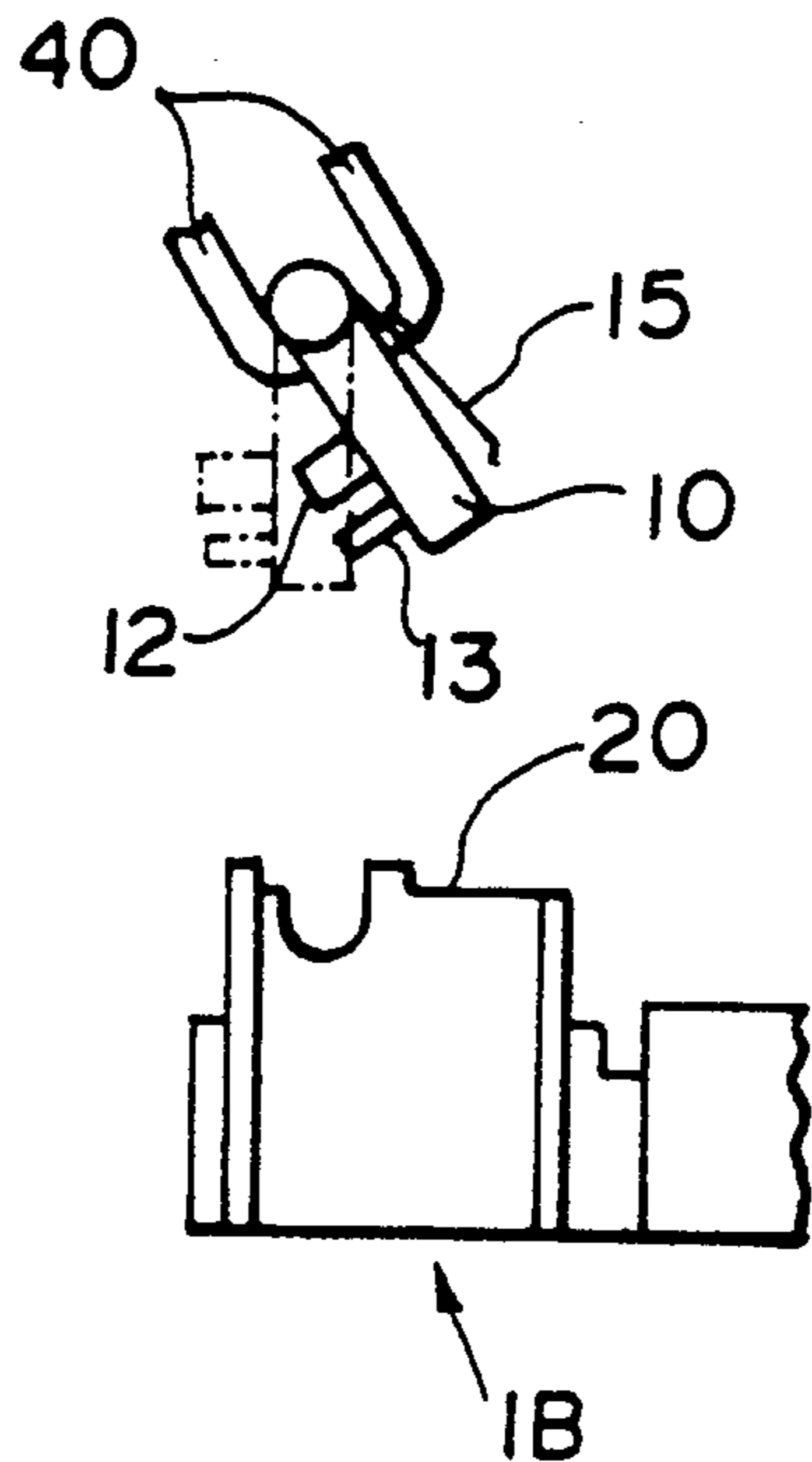
FIG. 7 PRIOR ART
