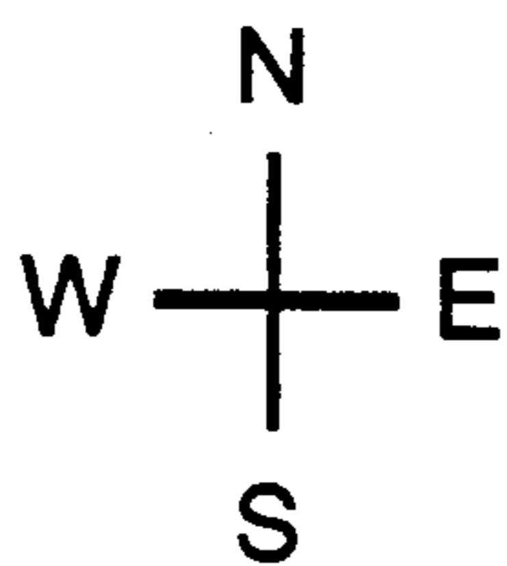
bitmap pattern
