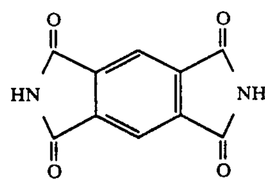
Pyromellitic diimide
