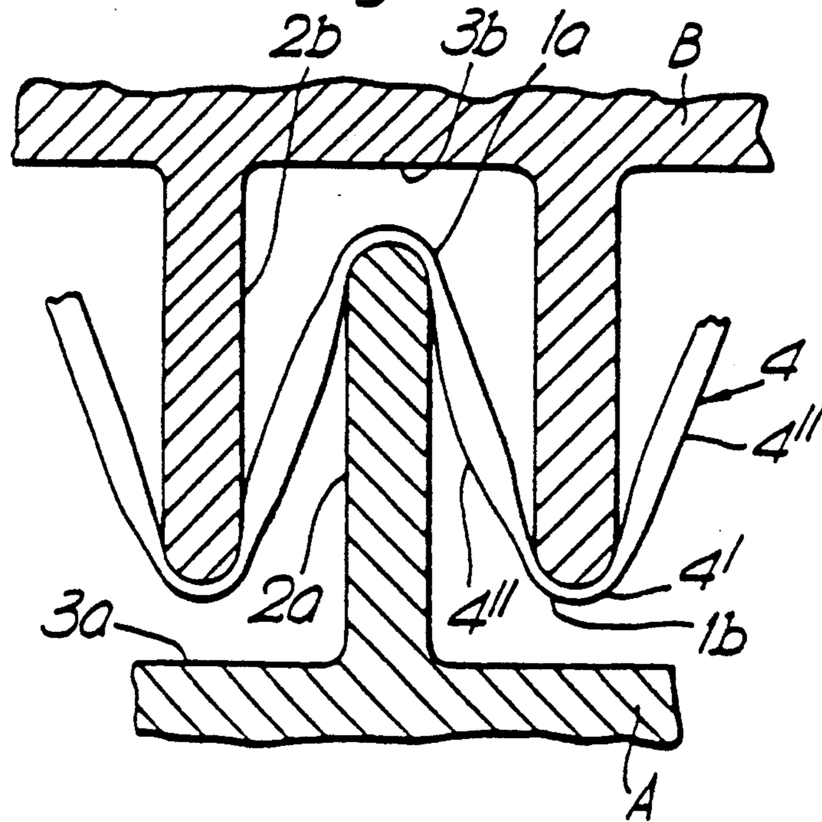
Fig. 1. PRIOR ART
