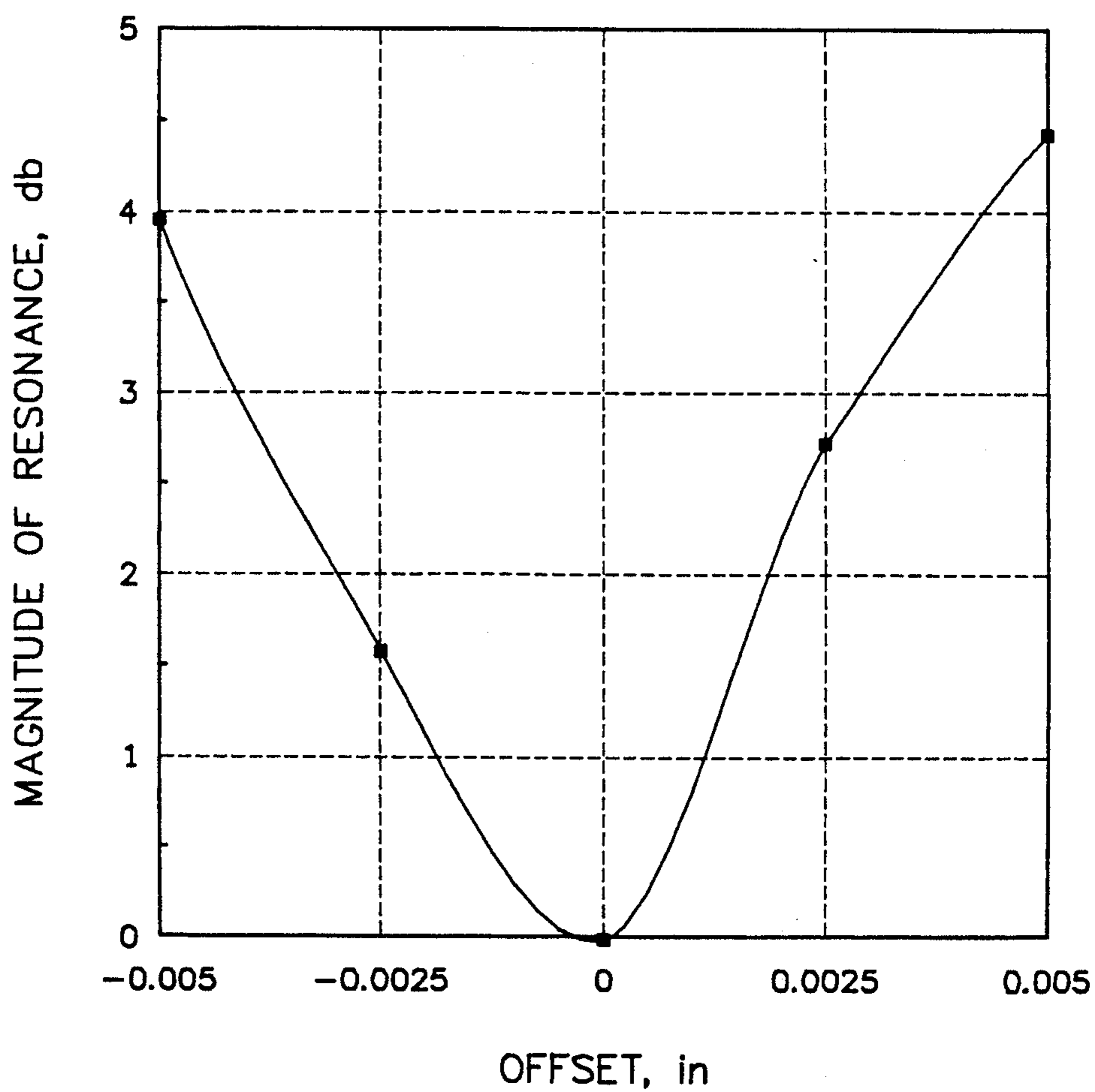
RESONANT AMPLITUDE VERSUS OFFSET — FIRST TORSION SUSPENSION WITHOUT CROSS-BRACE
