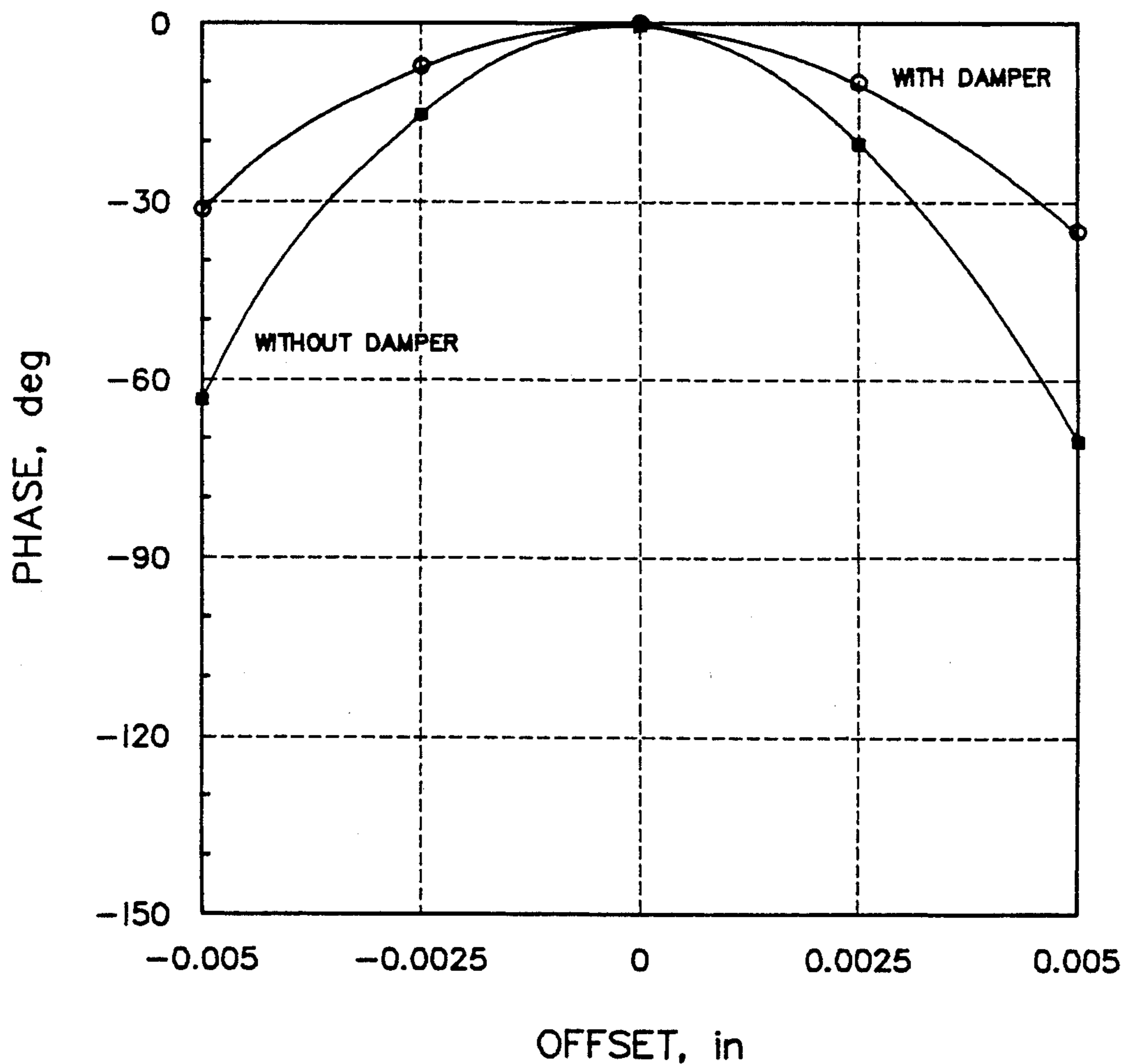
PHASE LOSS VERSUS OFFSET — FIRST TORSION MODE SUSPENSION WITHOUT CROSS-BRACE
