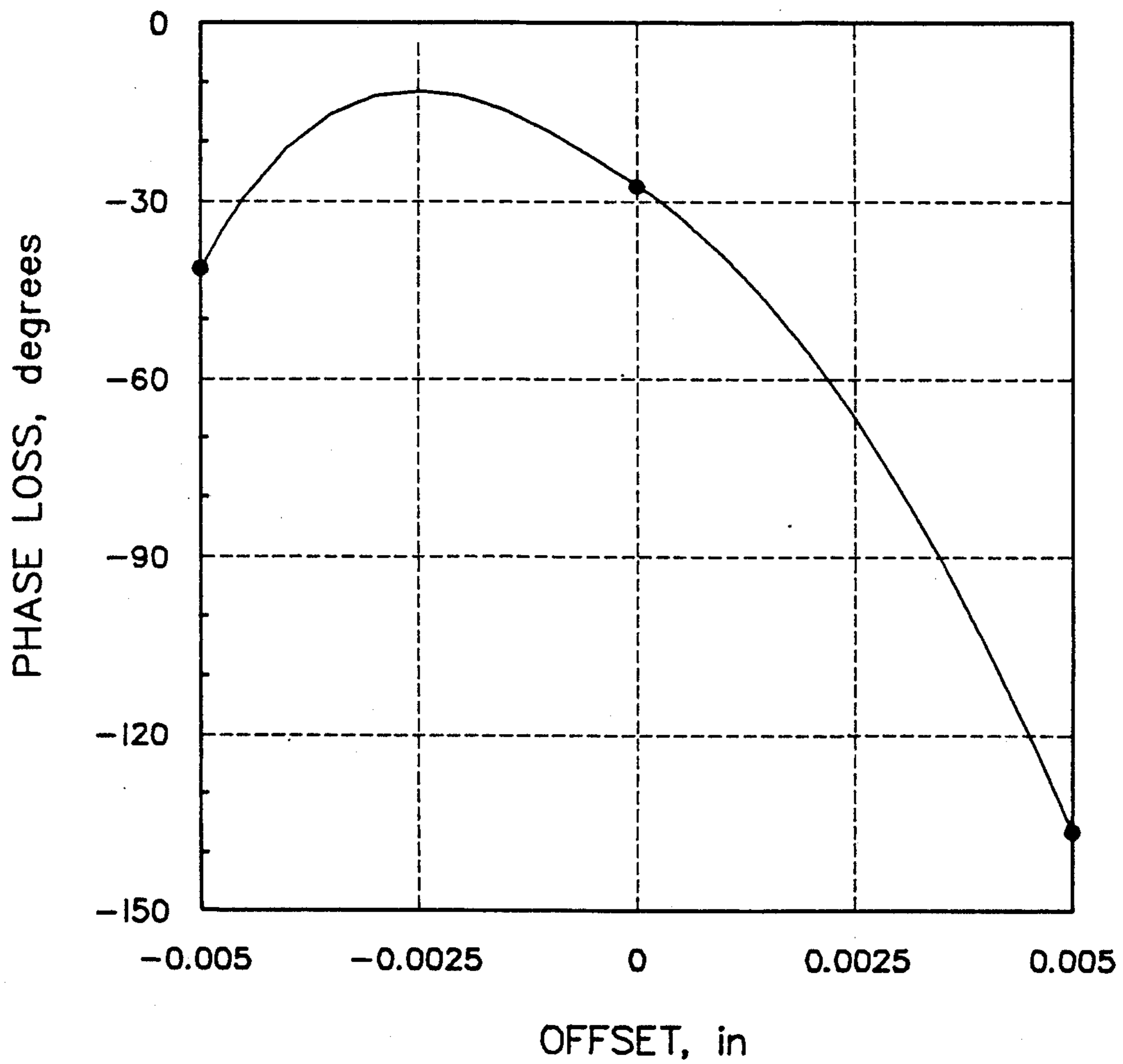
PHASE LOSS VERSUS OFFSET — FIRST TORSION MODE 70% MICRO-WHITNEY SUSPENSION
