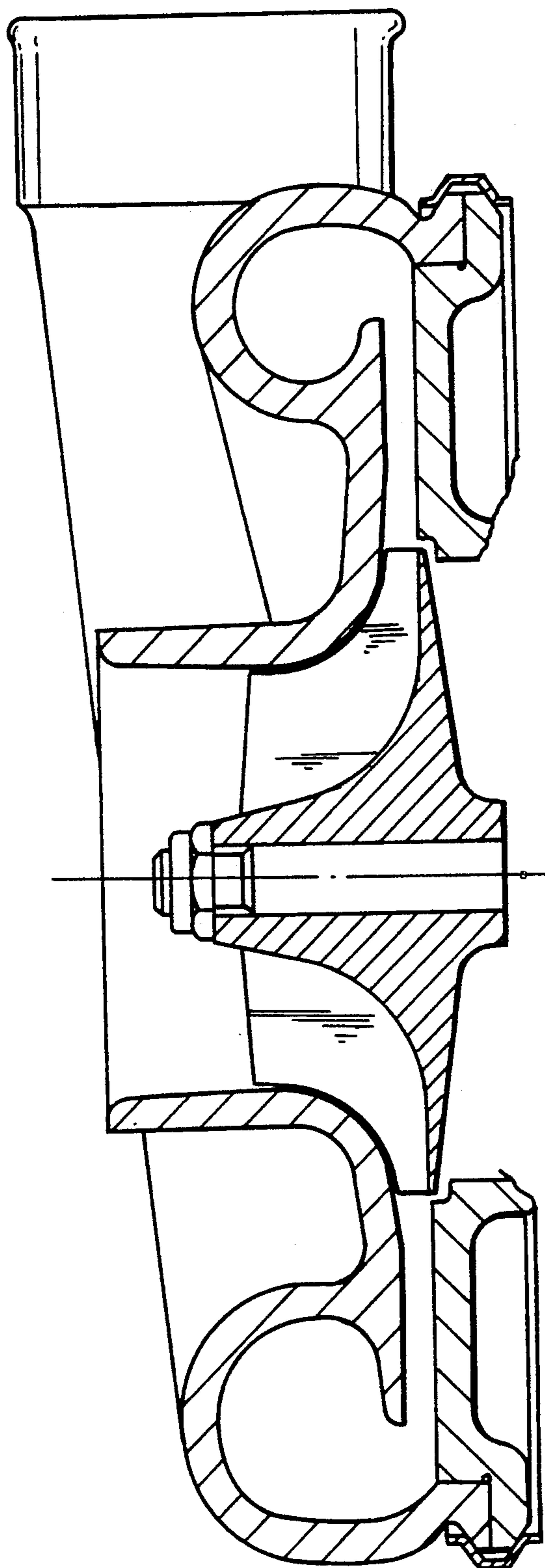
CENTRIFUGAL COMPRESSOR
