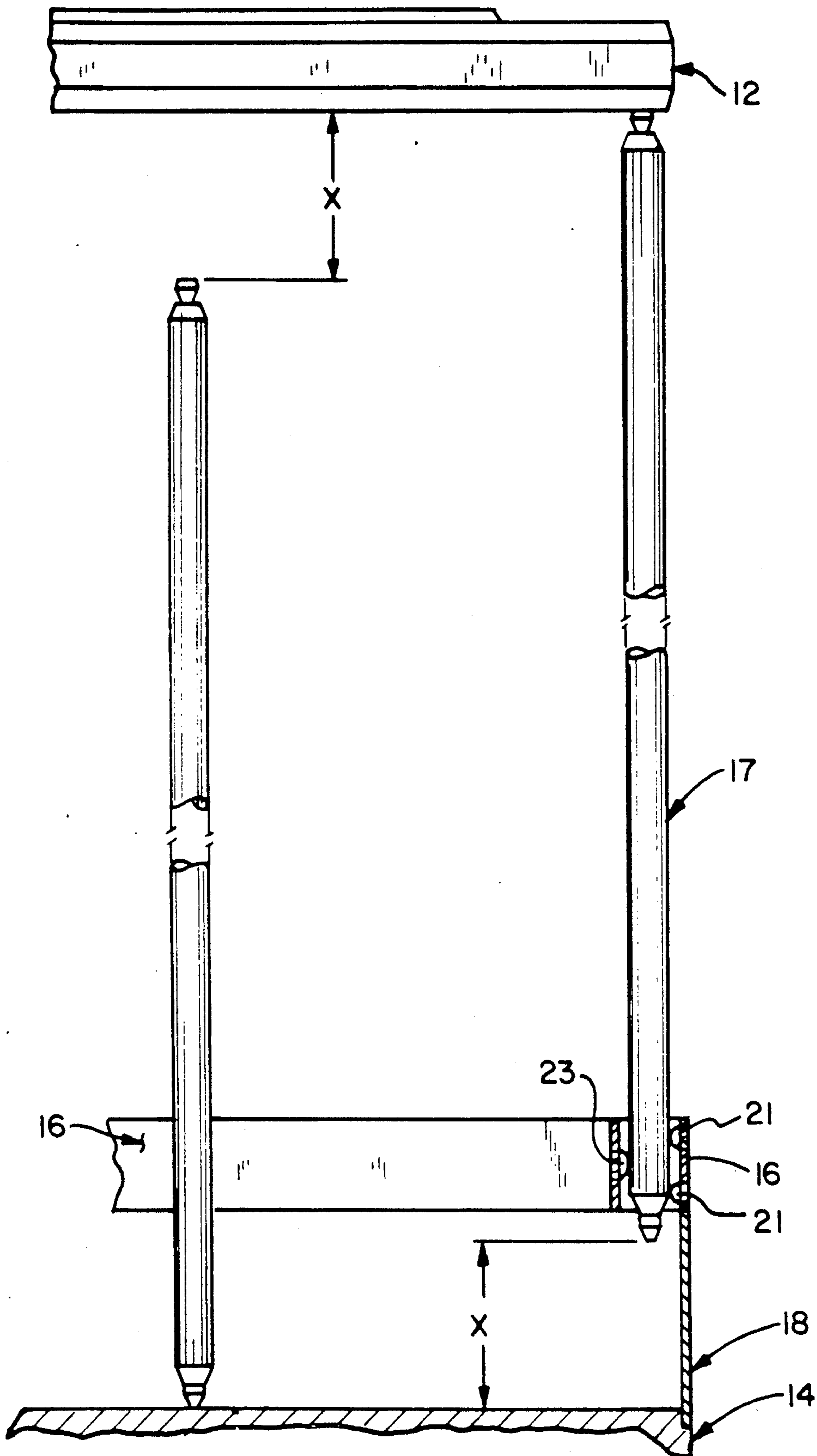
Fig. 2 (PRIOR ART)
