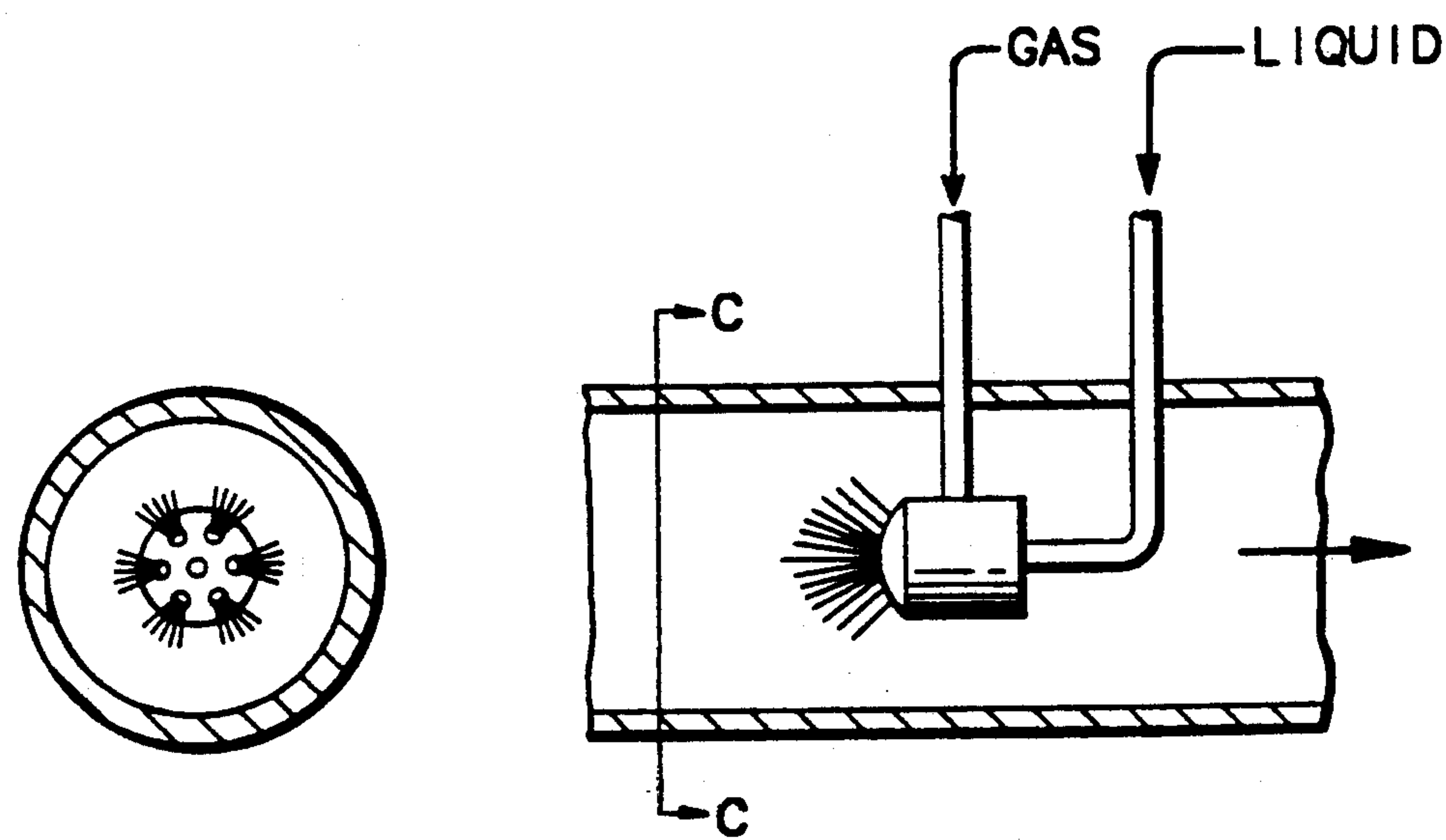
VIEW C-C
